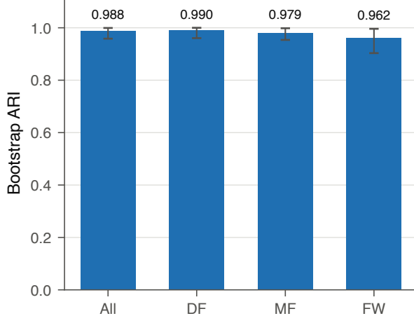
Stability, 50 resamples
