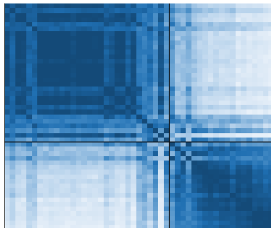
FW (n=49, mean ARI 0.60)
