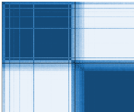
MF (n=181, mean ARI 0.82)
