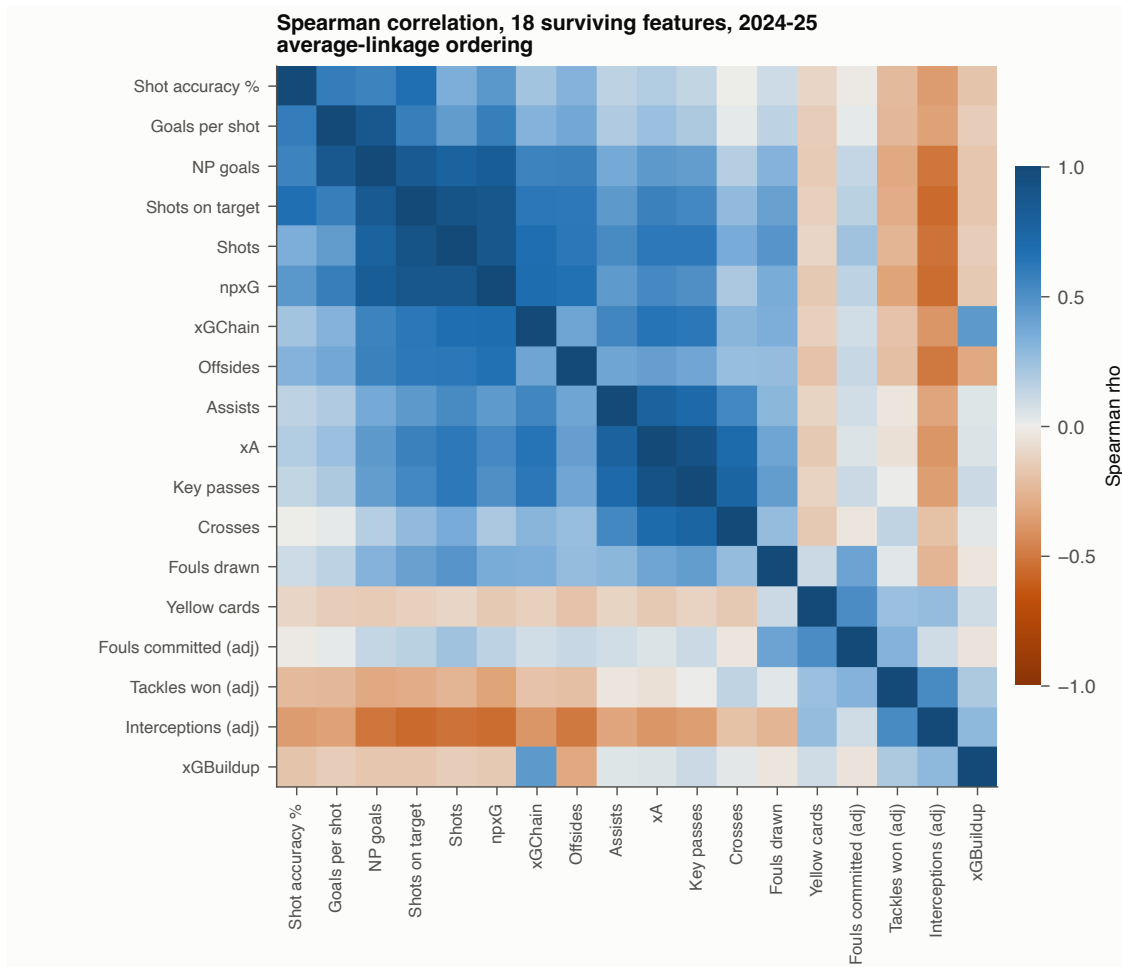
Figure 27: Hierarchically clustered Spearman correlation matrix over the outfield feature set in the primary season.
