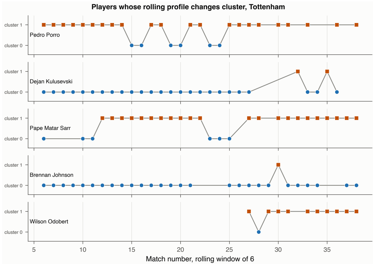
Figure 21: Rolling cluster assignment across the season for the Tottenham players who change cluster at least once, on a 6 match window. Players not shown occupied one cluster for the whole season.
