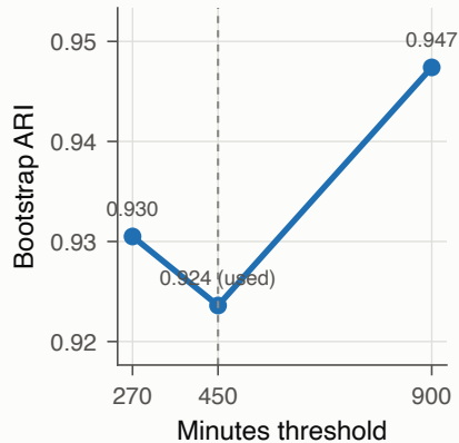
Bootstrap ARI
