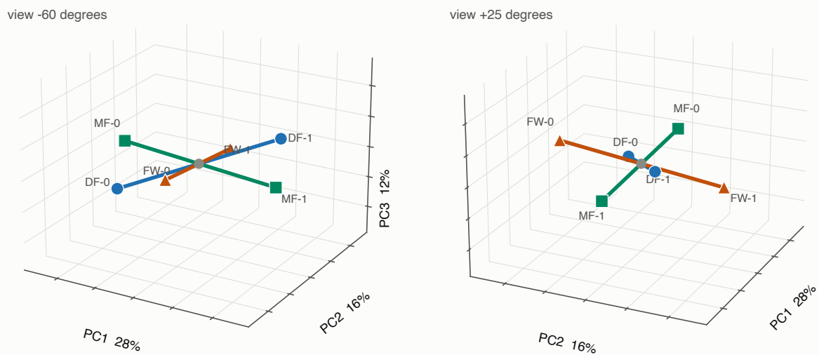
Figure 36: Archetype centroid directions, drawn as unit vectors so the figure shows orientation rather than magnitude. Each position group forms a single line through the origin, so the six archetypes describe three axes.
