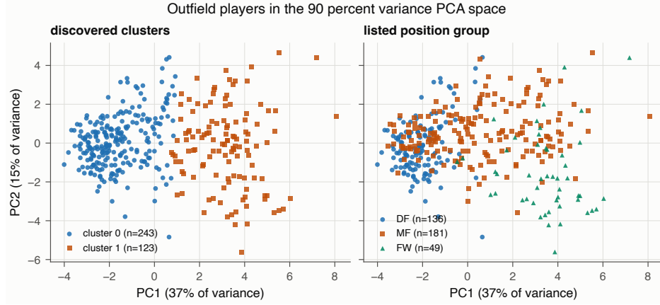
Figure 30: The selected partition shown in the principal component space.
