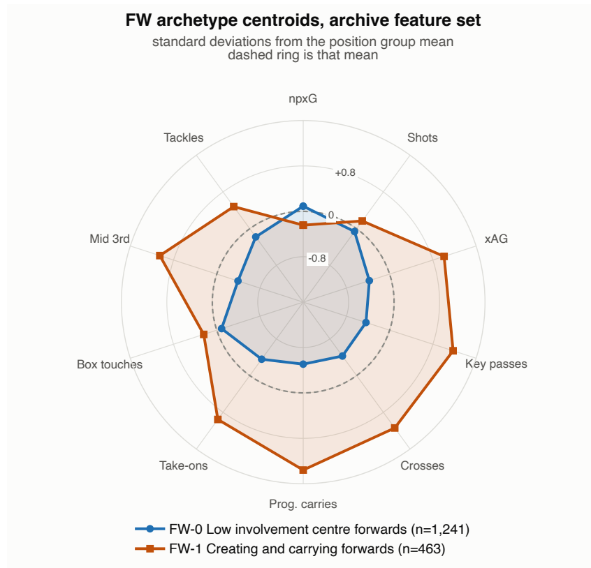
Figure 24: Forward archetypes, archive sample.
