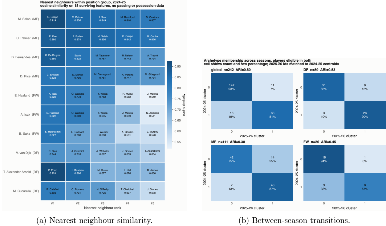
Figure 41: Similarity structure and cross-season replication.
