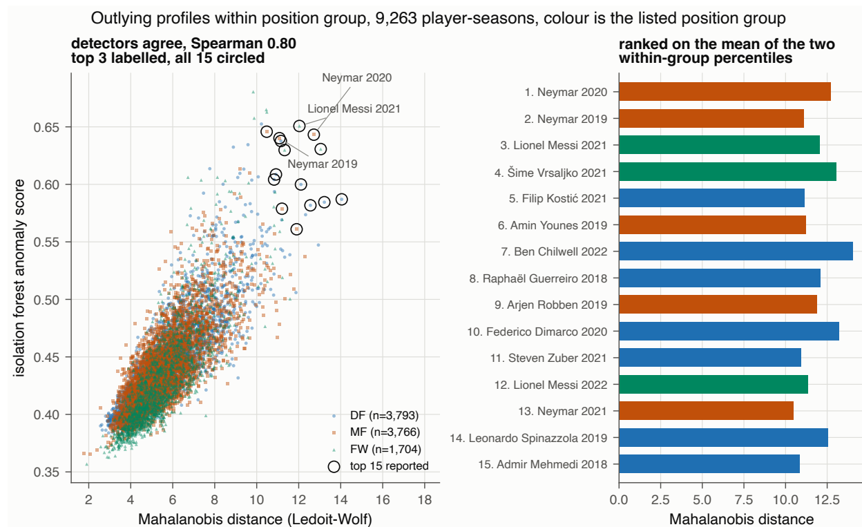
Figure 11: Isolation forest score against Mahalanobis distance within position group. The two detectors are computed independently and rank the same players highly, and the flagged points are dominated by players carrying compound listed positions.
