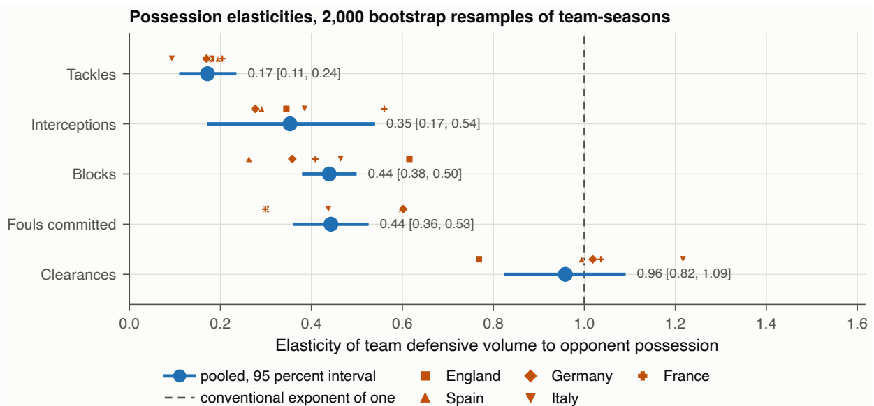
Figure 12: The five defensive possession elasticities with bootstrap intervals from 2,000 resamples of 490 team-seasons, against the conventional value of one, with each league's own refit shown as a smaller marker. Four intervals exclude one; the interval for clearances does not, and three league refits for clearances sit above one.
