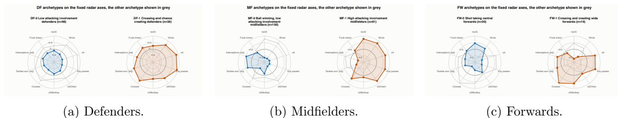
Figure 48: Archetype radars on the reduced sample.
