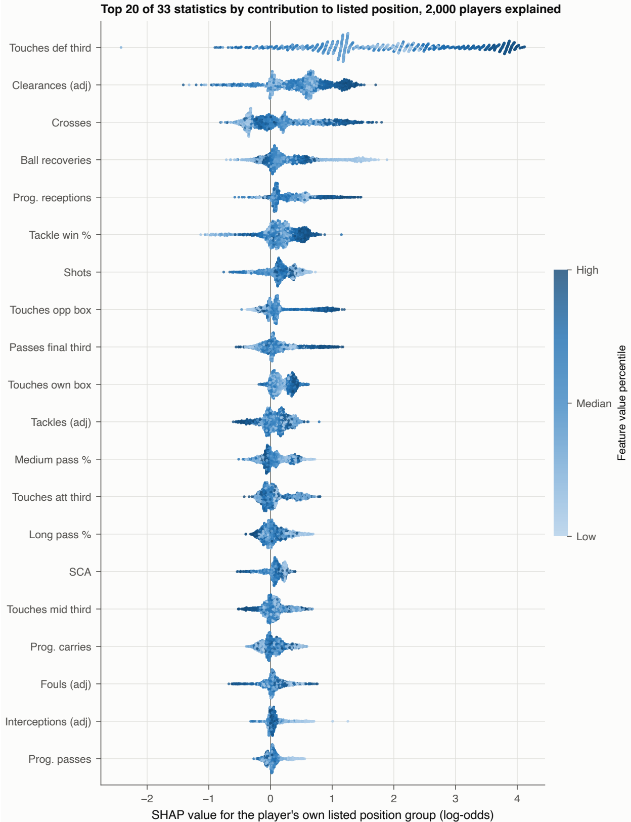
Figure 9: SHAP values for the gradient boosted model, showing for each player the contribution of each feature toward the position group the player is actually listed at. Territorial features dominate technical ones throughout.
