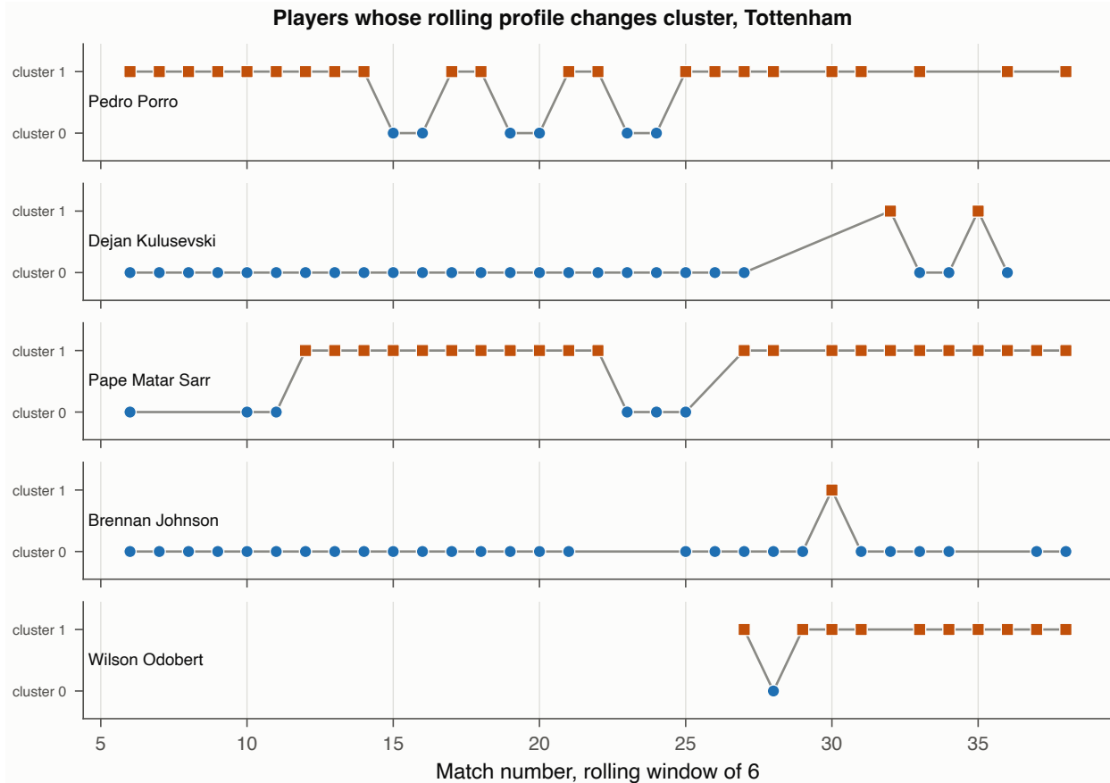
Figure 42: Rolling cluster assignment across the season for the Tottenham players who change cluster at least once, on a 6 match window. Players not shown occupied one cluster for the whole season.
