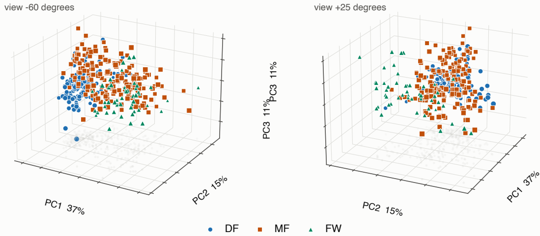
Figure 33: Outfield players in the first three principal components, from two viewpoints. Grey points on the floor are the vertical projection of each player, supplying a depth cue that a static rendering otherwise lacks.
