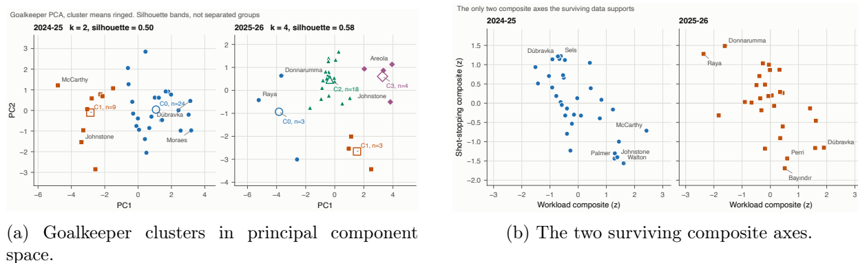
Figure 49: Goalkeeper structure on the reduced sample.
