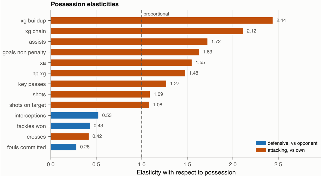
Figure 13: Possession elasticities for both families of statistic, fitted from team totals. Defensive volume responds to opponent possession less than proportionately, while attacking output responds to a team’s own possession more than proportionately. Crossing is the one attacking statistic that behaves like a defensive one.
