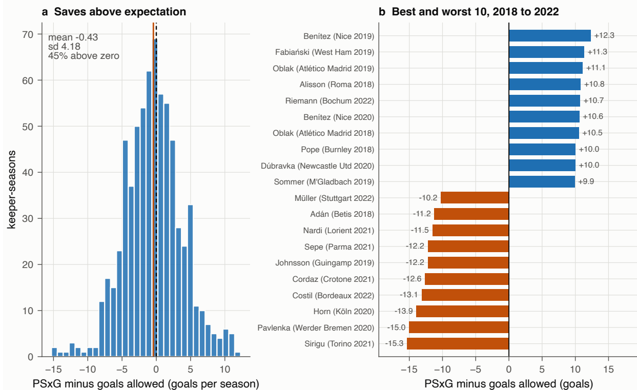
Figure 14: Goalkeepers ranked by post-shot expected goals minus goals allowed, which conditions on the difficulty of shots faced rather than only their volume.
