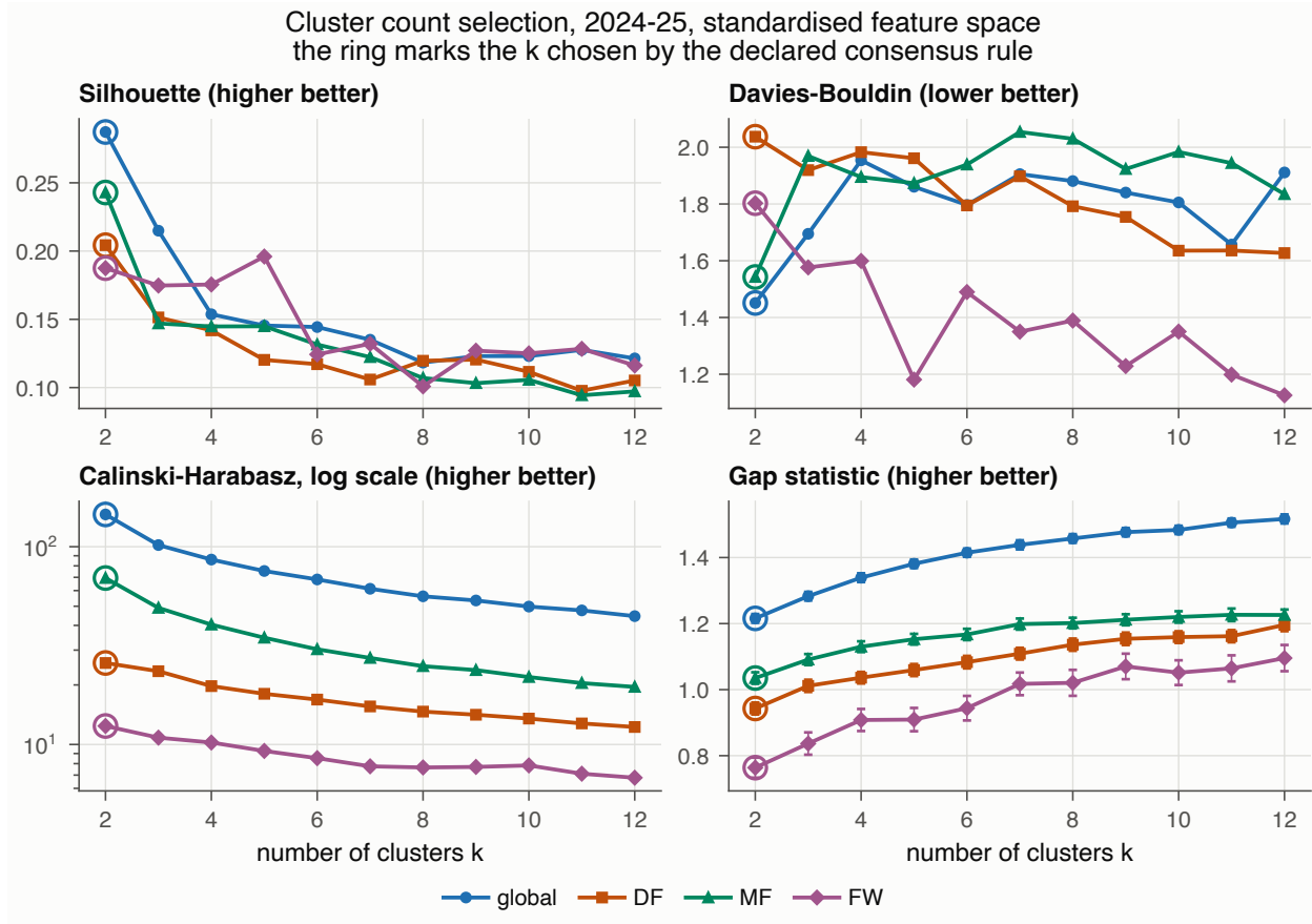
Figure 28: Cluster selection criteria across candidate cluster counts. The consensus rule was fixed before fitting and selects the same value in every scope.
