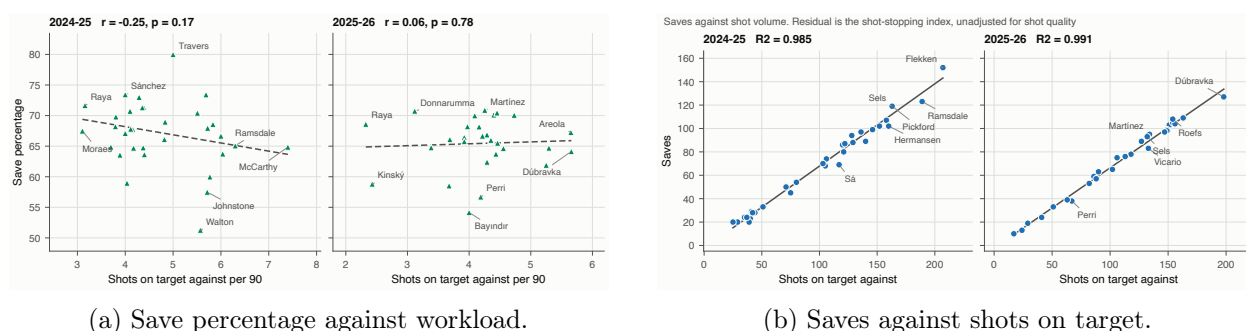
Figure 50: Goalkeeper shot stopping on the reduced sample. With expected goals on target with-drawn, save percentage against volume is the only shot stopping view the reduced sample supports, and it cannot separate difficulty from quantity.
