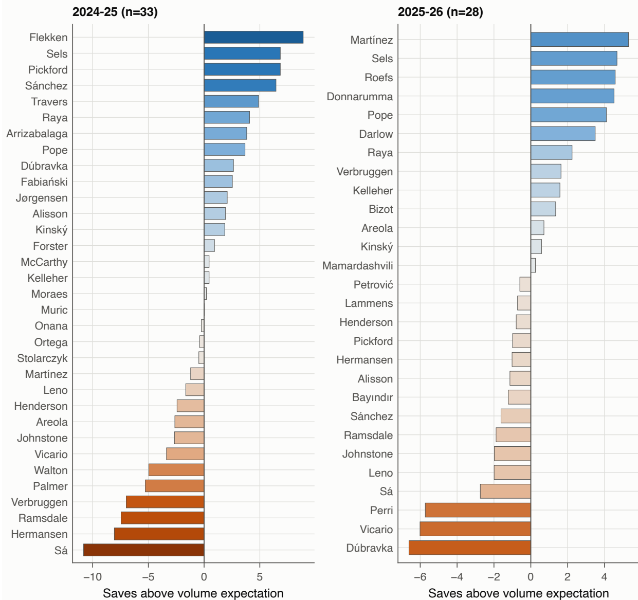
Figure 51: Goalkeeper shot stopping ranking on the reduced sample.
