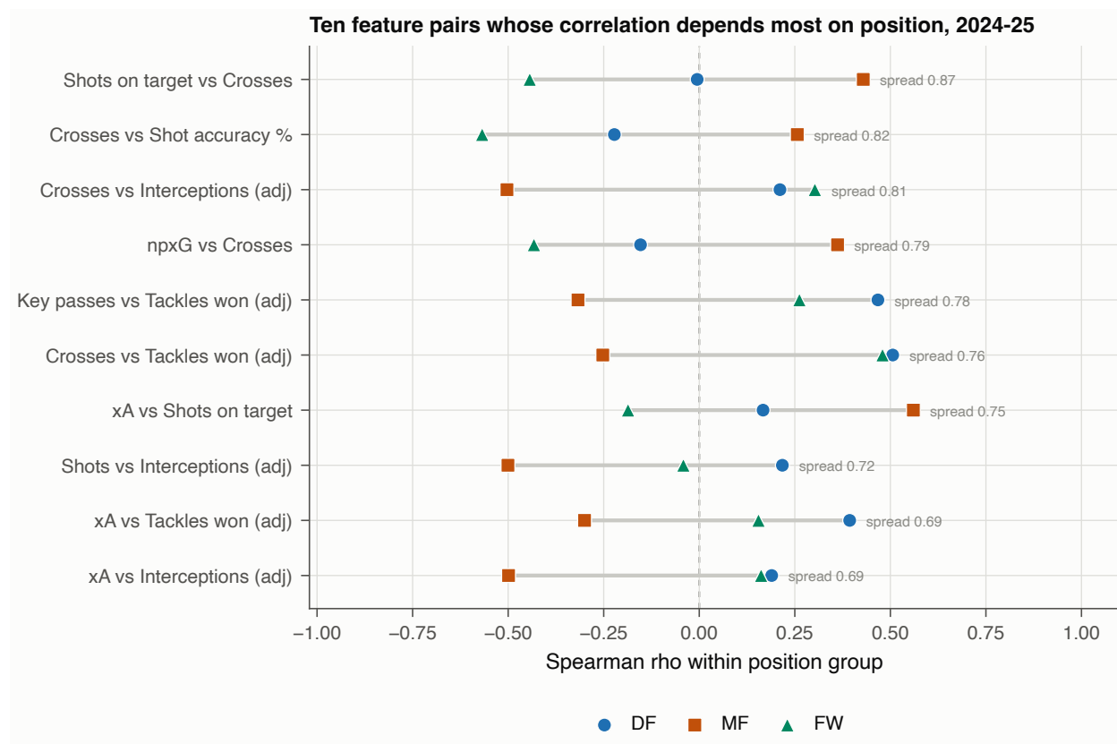
Figure 16: The ten feature pairs whose within-group correlation differs most across position groups in the earlier of the two reduced-sample seasons. Every pair changes sign between at least two groups.
