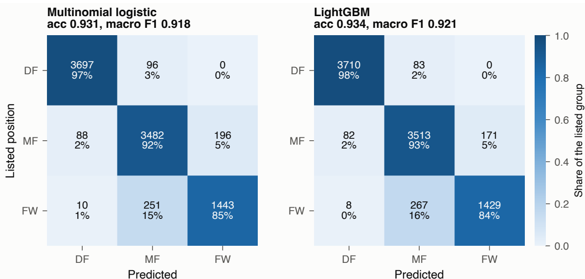
Figure 8: Out of fold confusion for both classifiers on 9,263 player seasons. The corners linking defenders and forwards are close to empty and every substantial error passes through midfield, which is what an ordered space with two poles produces.
