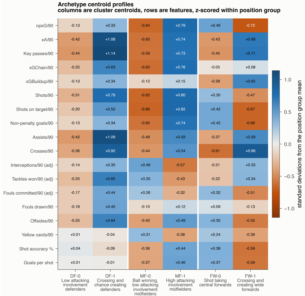
Figure 47: Centroid deviation of each archetype from its position group mean, reduced sample.
