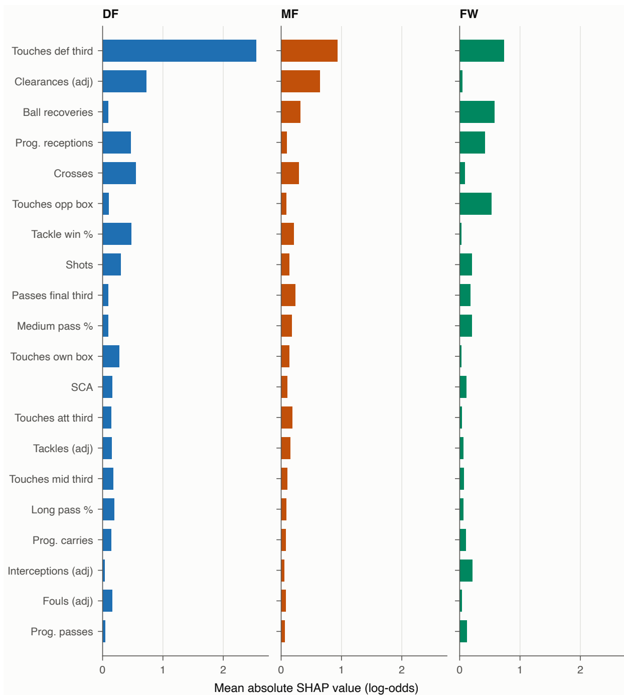
Figure 10: Mean absolute attribution per feature, split by position group. Touches in the defensive third dominate for all three, and the profile of what matters differs sharply between them: defenders are separated largely by defensive volume and crossing, forwards by where they receive the ball. The panel shows magnitude only; the direction each feature pushes is reported in the text.
