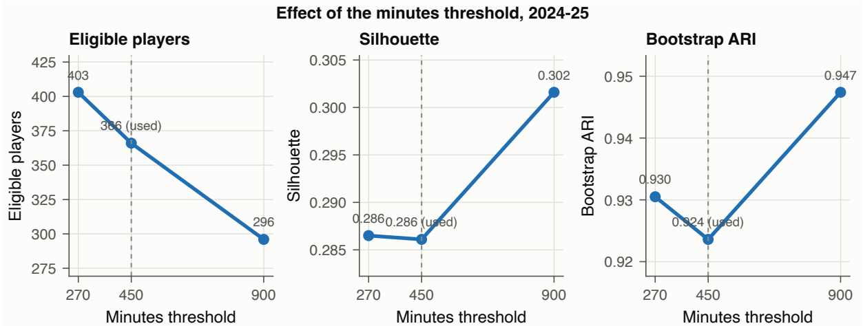
Figure 17: Eligible sample, silhouette and bootstrap stability across the candidate minutes thresholds. The dashed line marks the threshold used in the main analysis.
