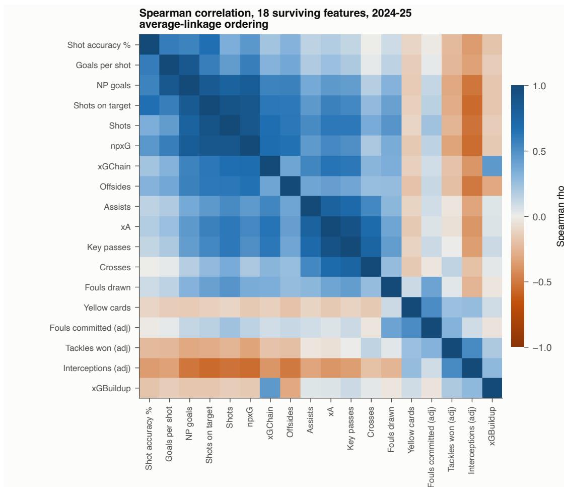
Figure 18: Hierarchically clustered Spearman correlation matrix over the outfield feature set in the earlier of the two reduced-sample seasons.
