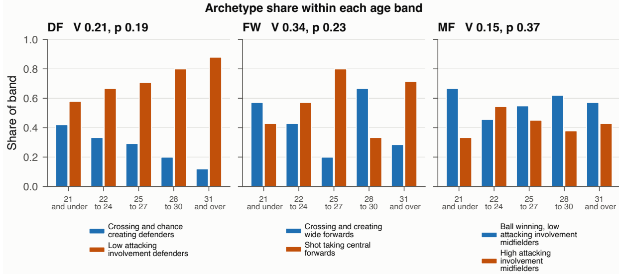
Figure 43: Share of each age band taken by each archetype, within position group. The defender panel falls monotonically with age, which a chi-square on bands does not detect and a rank correlation does.
