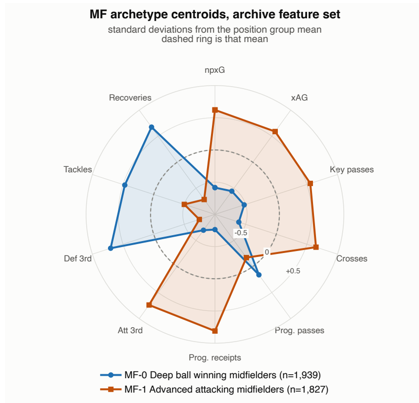
Figure 23: Midfielder archetypes, archive sample.
