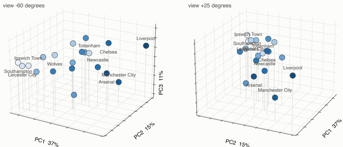
Figure 35: Clubs as minutes-weighted centroids in three components, shaded by final league position with darker shading for a higher finish. Vertical lines to the floor give the depth cue, and only the top and bottom of the table are labelled.
