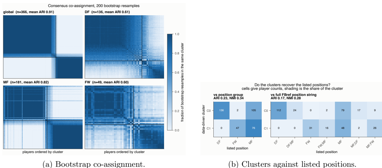
Figure 29: Cluster stability and the correspondence with listed positions.
