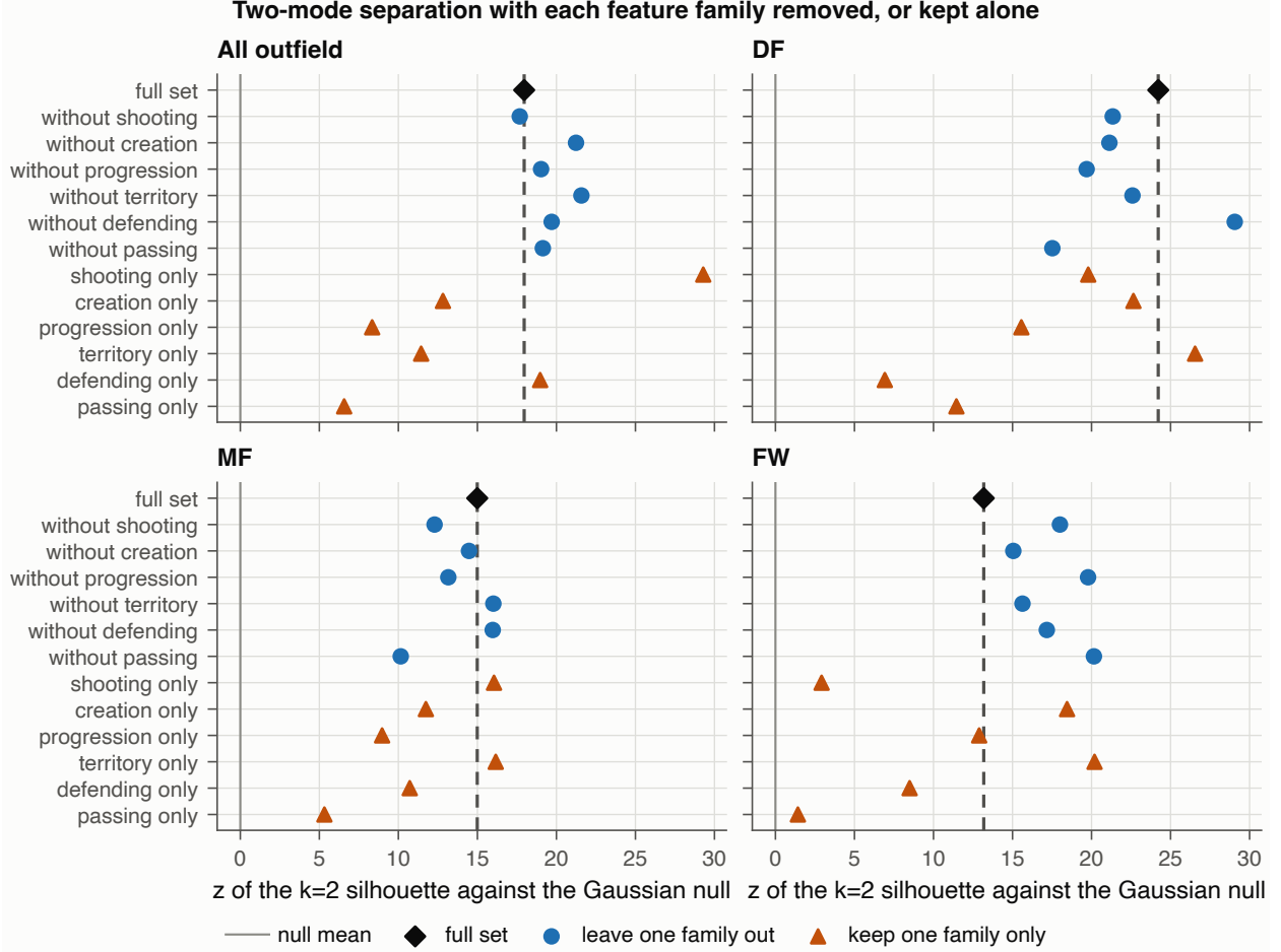
Figure 7: Standard score of the observed two-cluster silhouette against the clusterless null under every feature-family ablation, one panel per scope. Circles remove one family, triangles keep one family alone, and the vertical line is the full feature set. The adjusted Rand index against the full partition, which distinguishes the same two modes from a different pair, is in Table 2 and the text.
