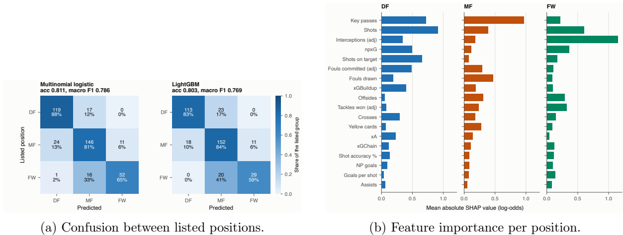
Figure 38: Supervised validation of the surviving feature set.
