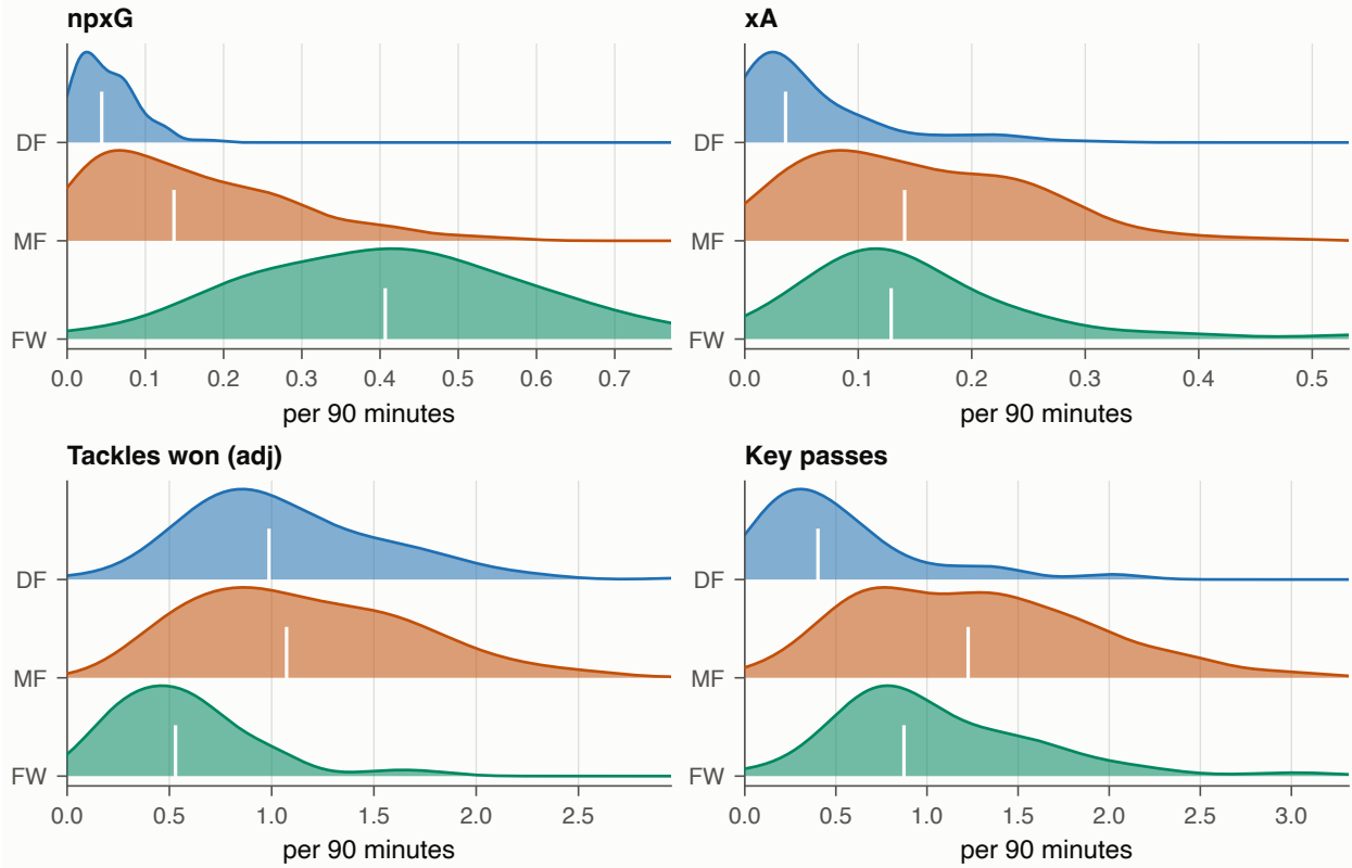
Figure 31: Distributions of four representative per-90 statistics across position groups in the earlier of the two reduced-sample seasons. The separation between groups is clear for shot volume and for defensive actions, and much weaker for creation.
