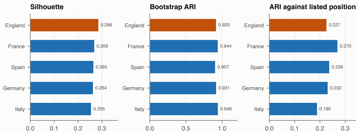
Figure 37: The pipeline applied unchanged to each of the big five leagues in the primary season. The selected number of clusters, the silhouette, bootstrap stability and agreement with listed positions are all close across competitions.
