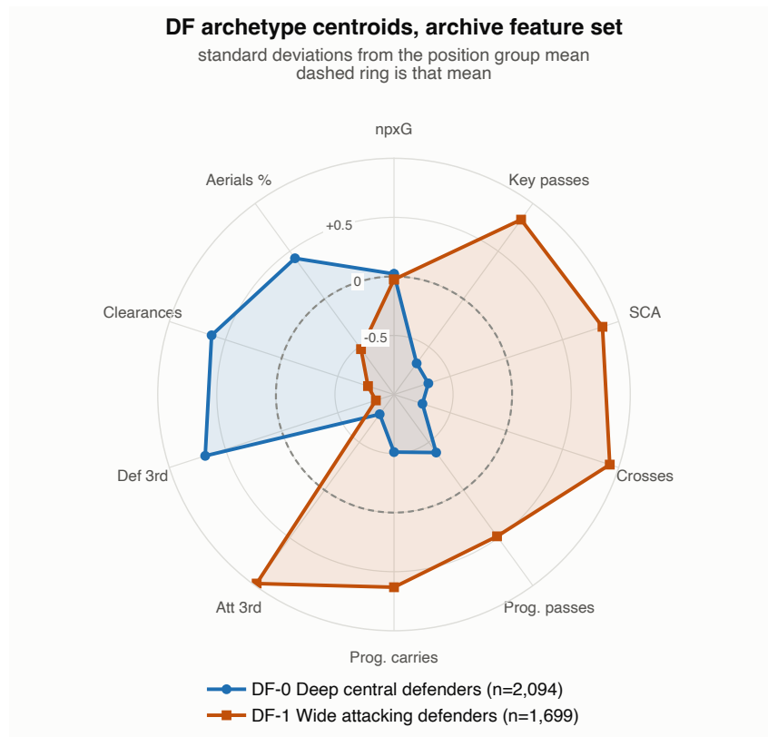
Figure 22: Defender archetypes, archive sample.
