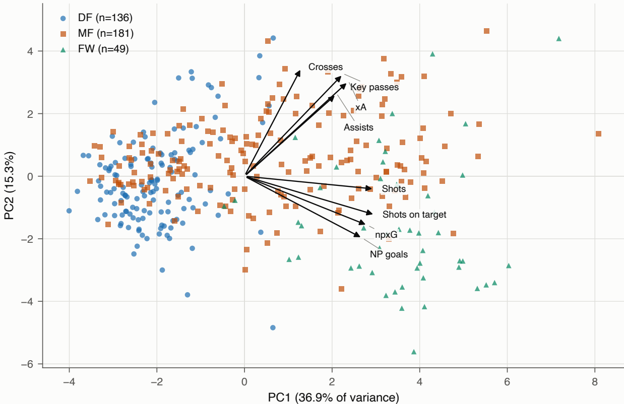
PCA biplot of the surviving feature set, 2024-25
