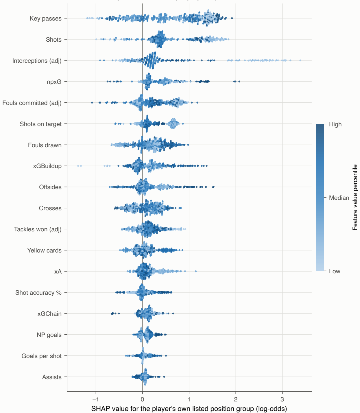
Which surviving statistics identify a player's position
