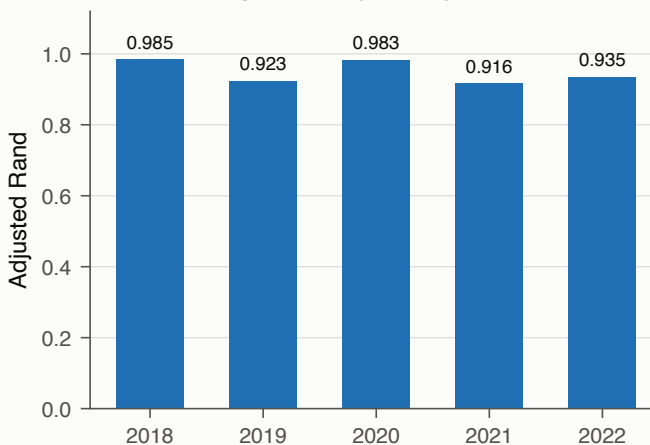
Season fits against the pooled partition
