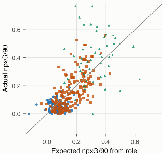
Chain columns removed, R^2 = 0.535
