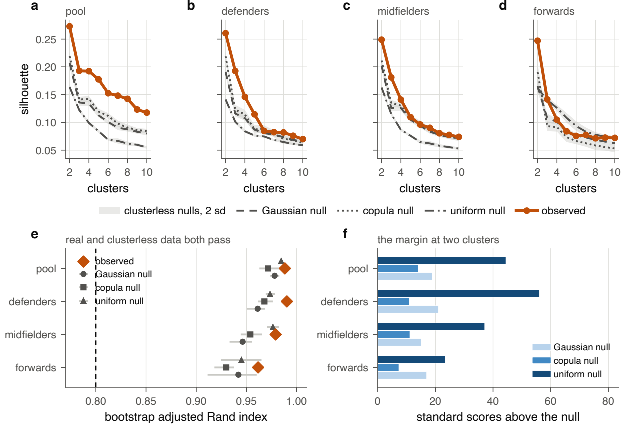
Figure 1: Two modes are real and nothing finer is. a to d , observed silhouette against three kinds of data built to contain no clusters, one panel per scope. Each null is simulated 100 times and drawn as its mean with a band of two standard deviations: a Gaussian matched on covariance, a copula that keeps every real marginal and correlation, and the uniform reference of the gap statistic. The observed curve separates from all three at two clusters. Within a position group it rejoins a band as the number of clusters grows, at three, five and six clusters for forwards, midfielders and defenders; in the pooled scope it stays above all three at every candidate number, which is what the two-mode division that scope contains produces when the same cloud is cut into more pieces. e , bootstrap adjusted Rand index on the real data against the same quantity on the clusterless simulations, with the range over simulated datasets and the dashed line at 0.8, the screen a published taxonomy would cite as evidence that its partition is stable. The real data score a little higher than the clusterless data, by as little as 0.003, and both sides clear the screen comfortably, which is why passing it is not evidence that groups exist. f , the margin at two clusters, as standard scores above each null.
