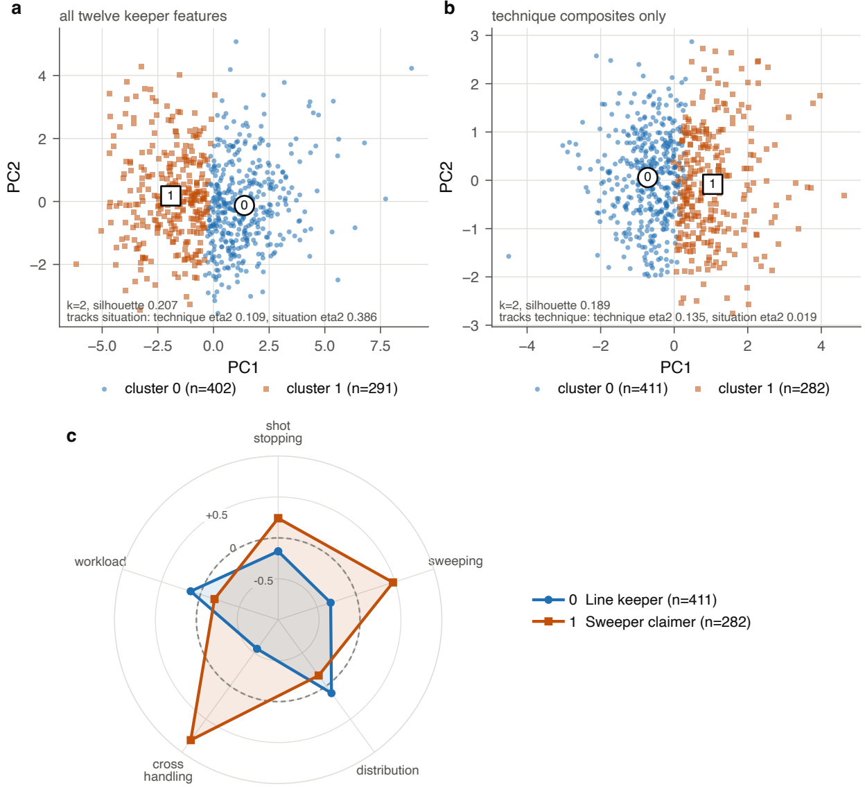
Figure 6: Goalkeeper structure on the primary sample. a and b , the technique partition, which separates goalkeepers who stay on their line from those who come off it. c , the two cluster centroids on the five composite axes, in standard deviations from the eligible pool mean, with the dashed ring marking that mean and the distribution axis signed so that a higher value means shorter passing. The clusters separate on cross handling and sweeping together, while distribution and shot stopping vary continuously across both rather than distinguishing them.
