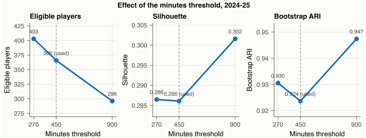
Figure 27: Eligible sample, silhouette and bootstrap stability across the candidate minutes thresholds. The dashed line marks the threshold used in the main analysis.
