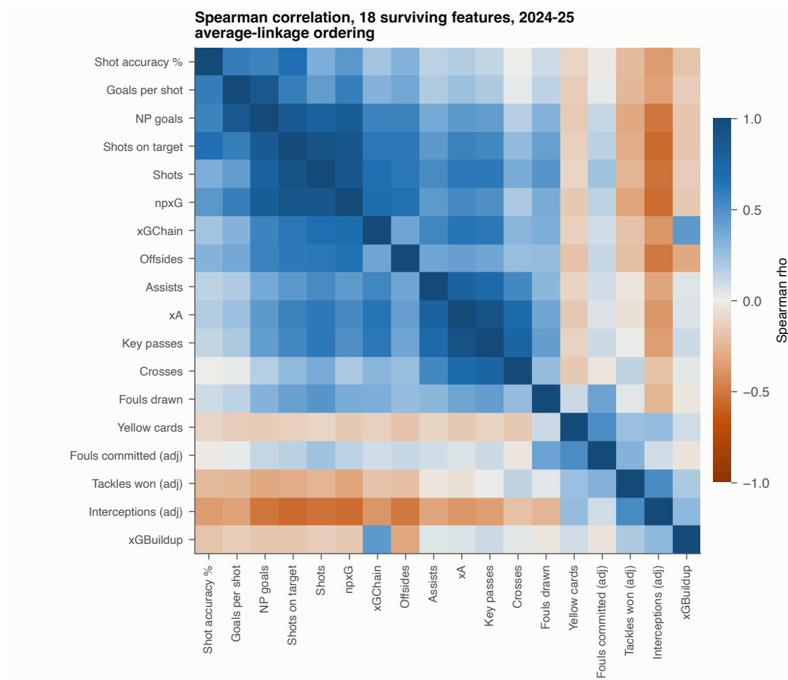
Figure 28: Hierarchically clustered Spearman correlation matrix over the outfield feature set in the primary season.
