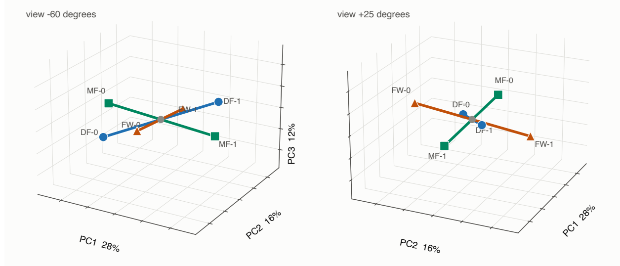
Figure 9: Archetype centroid directions, drawn as unit vectors so the figure shows orientation rather than magnitude. Each position group forms a single line through the origin, so the six archetypes describe three axes.
