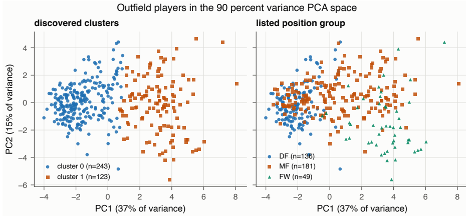
Figure 12: The selected partition shown in the principal component space.
