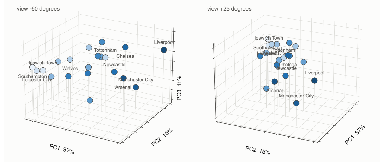
Figure 8: Clubs as minutes-weighted centroids in three components, shaded by final league position with darker shading for a higher finish. Vertical lines to the floor give the depth cue, and only the top and bottom of the table are labelled.
