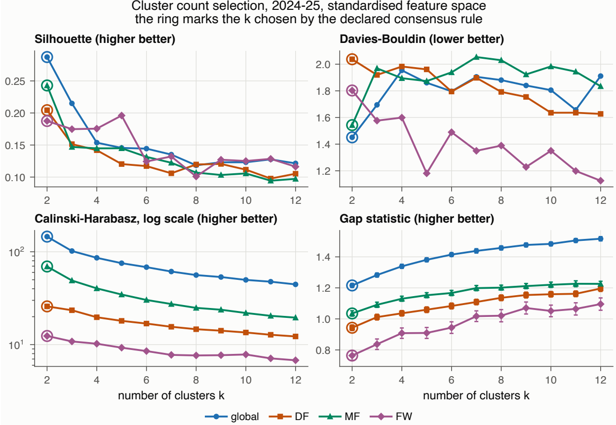
Figure 10: Cluster selection criteria across candidate cluster counts. The consensus rule was fixed before fitting and selects the same value in every scope.
