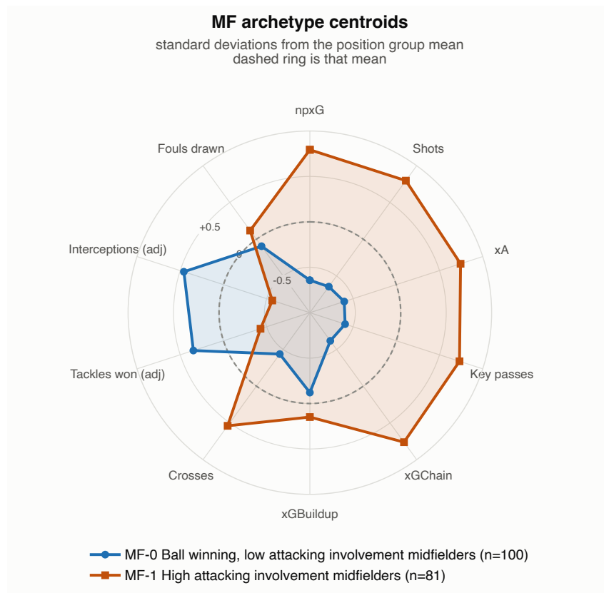
Figure 32: Midfielder archetypes.
