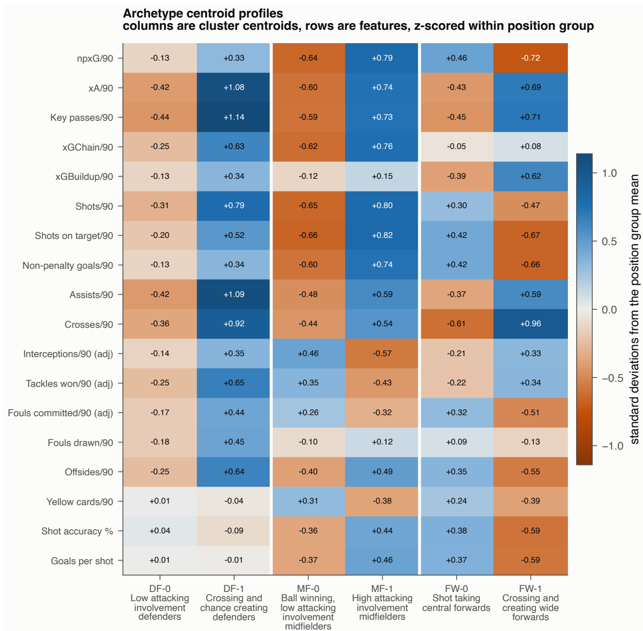
Figure 16: Centroid deviation of each archetype from its position group mean, across the full feature set. Within each position group the two profiles are necessarily mirror images, since the features are standardised within group before clustering.
