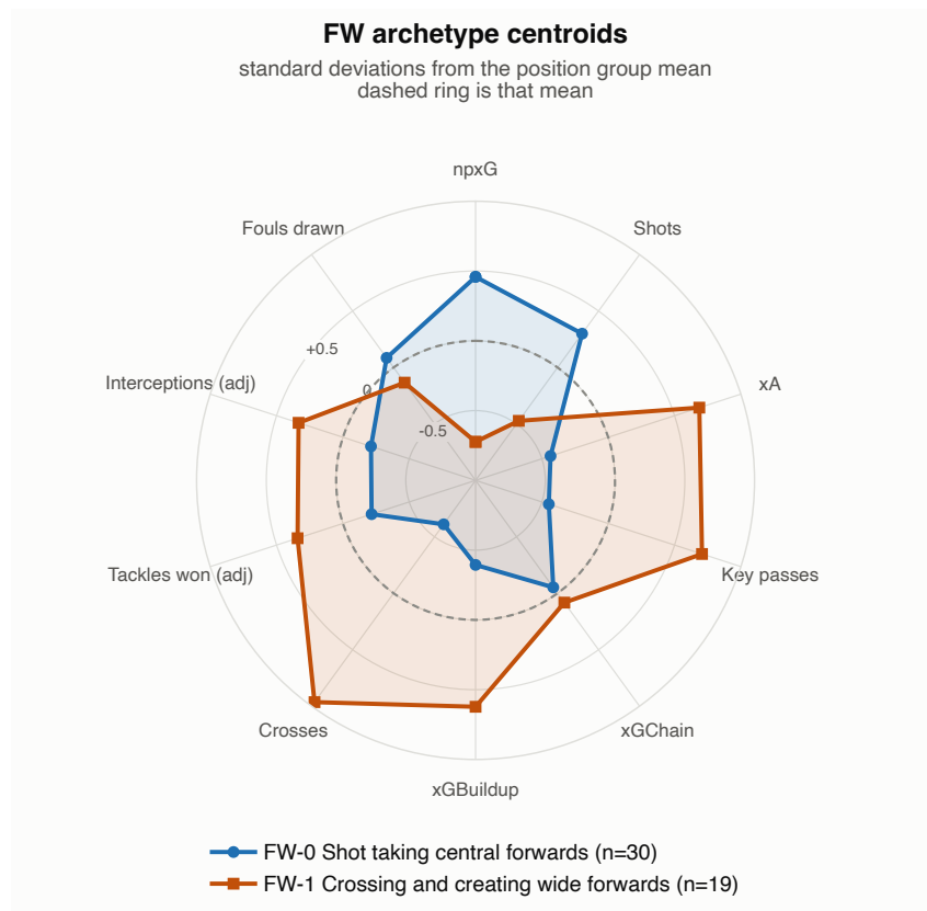
Figure 33: Forward archetypes.
