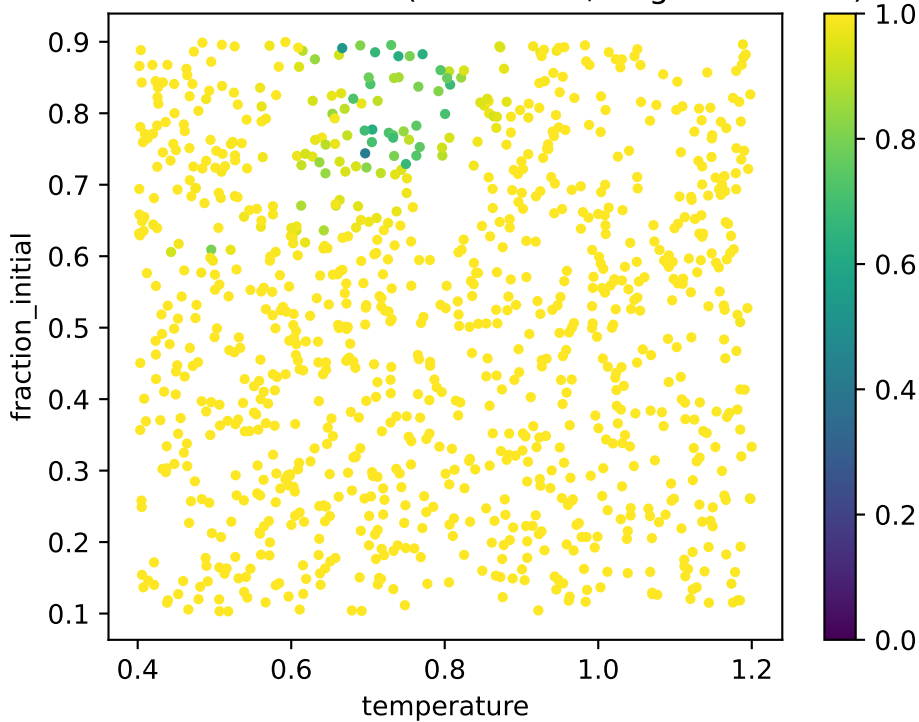
corr2d: worst retention (directional, ridge-stabilized)
