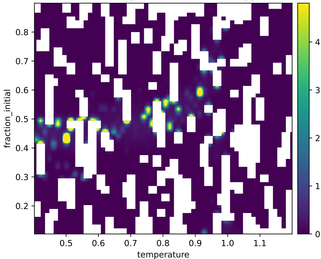
corr2d: heatmap forward LOO R^2 (clipped)
