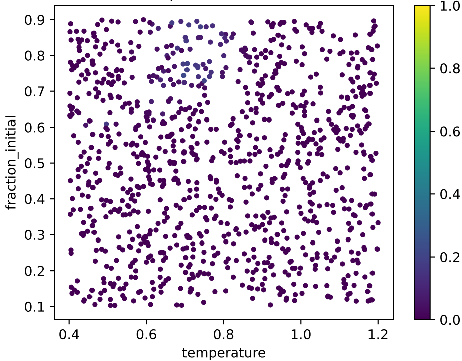
corr2d: unexplained fraction (baseline)
