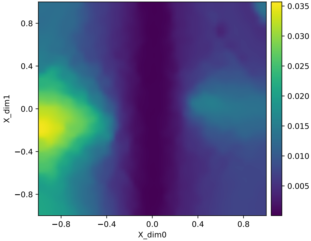
Forward map singular value smin(J) | pinch | repeats | Y=corr2d | q=16385 heatmap (adaptive)
