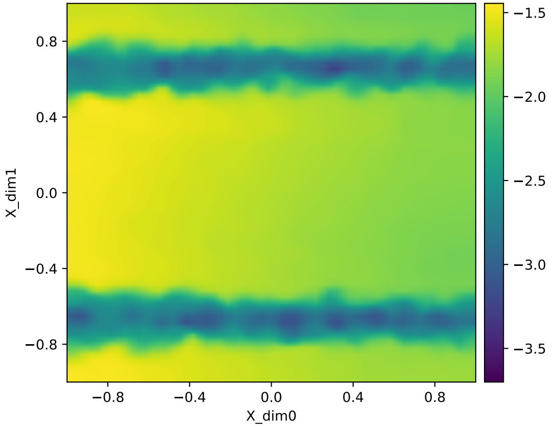
Forward map log10 singular value log10(smin(J)) | ribbon | repeats | Y=corr2d | q=16385 heatmap (adaptive)
