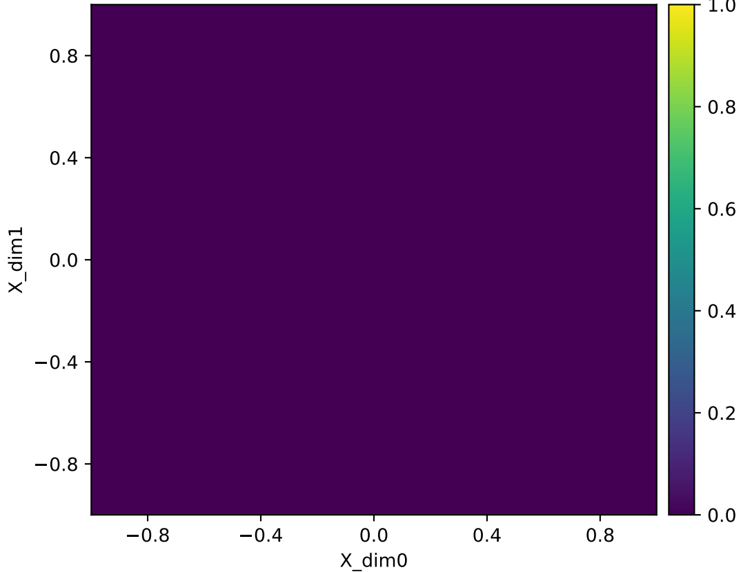
Forward map log10 singular value log10(smin(J)) | nowarp | repeats | Y=radial1d | q=65 heatmap (fixed [0,1])
