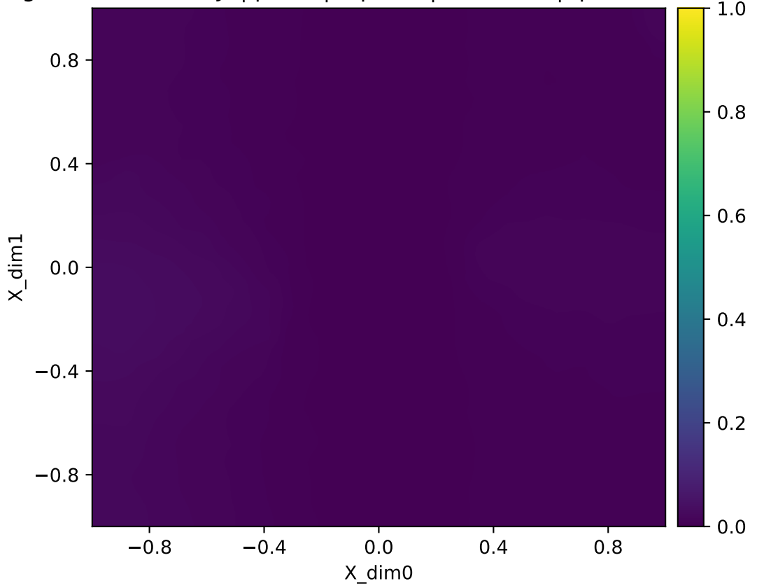
Forward map singular value smin(J) | pinch | repeats | Y=corr2d | q=16385 heatmap (fixed [0,1])
