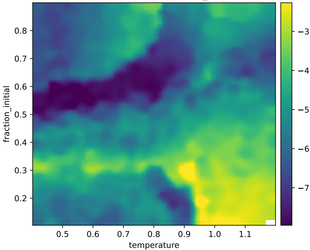
corr2d: heatmap logdet_Cx
