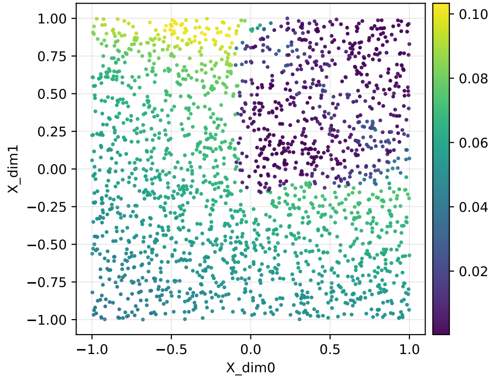
Forward map singular value \text{smin}(J) | fold | repeats | Y=radial1d | q=65 (adaptive)
