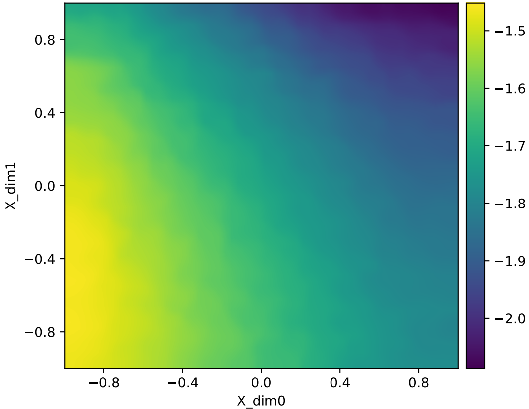
Forward map log10 singular value log10(smin(J)) | nowarp | repeats | Y=corr2d | q=16385 heatmap (adaptive)
