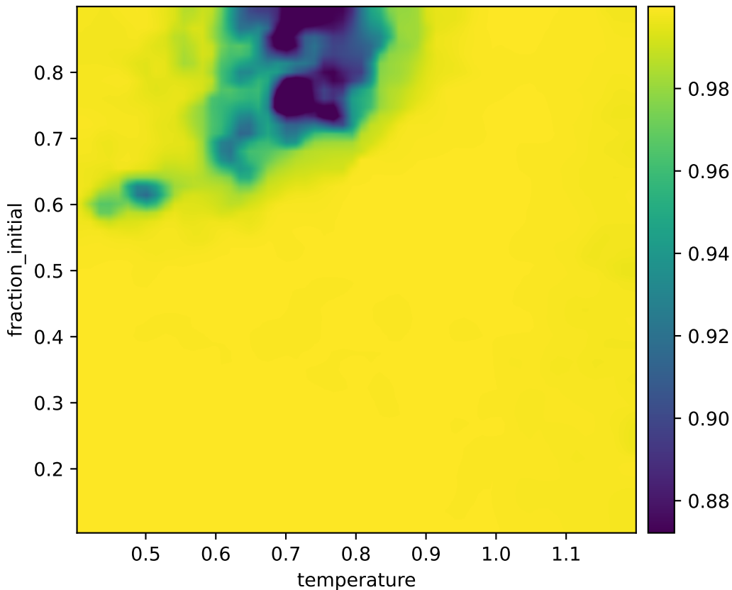
corr2d: heatmap explained fraction (baseline)
