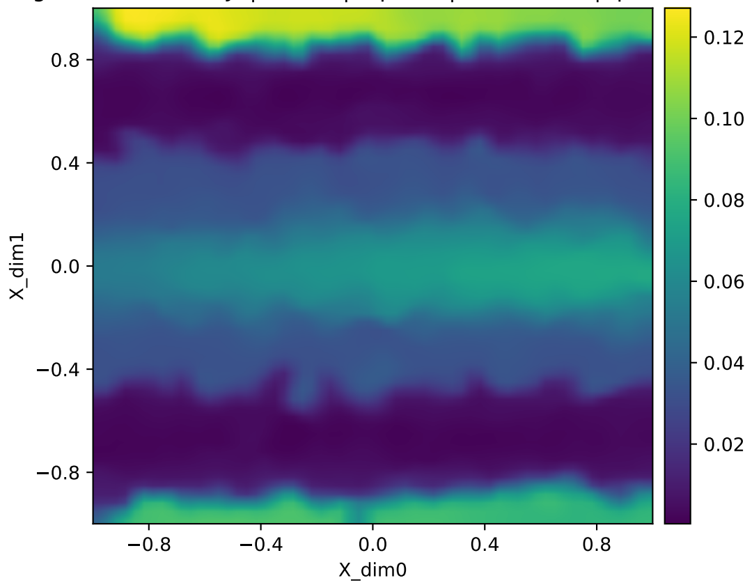
Forward map singular value \text{smin}(J) | ribbon | repeats | Y=\text{radial1d} | q=65 heatmap (adaptive)
