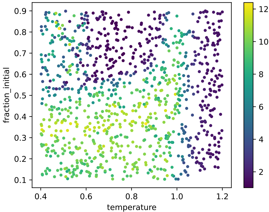
corr2d: stable rank of local K
