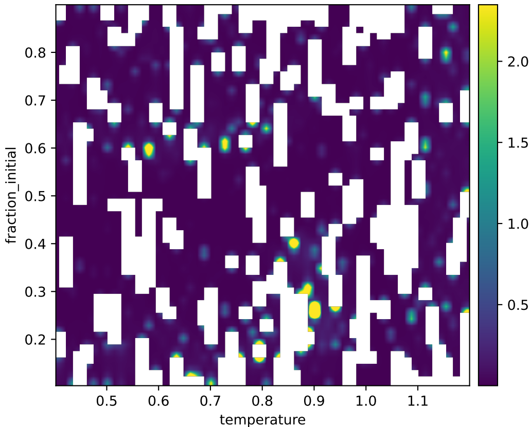
corr2d: heatmap lambda2 (2D controllability gate)
