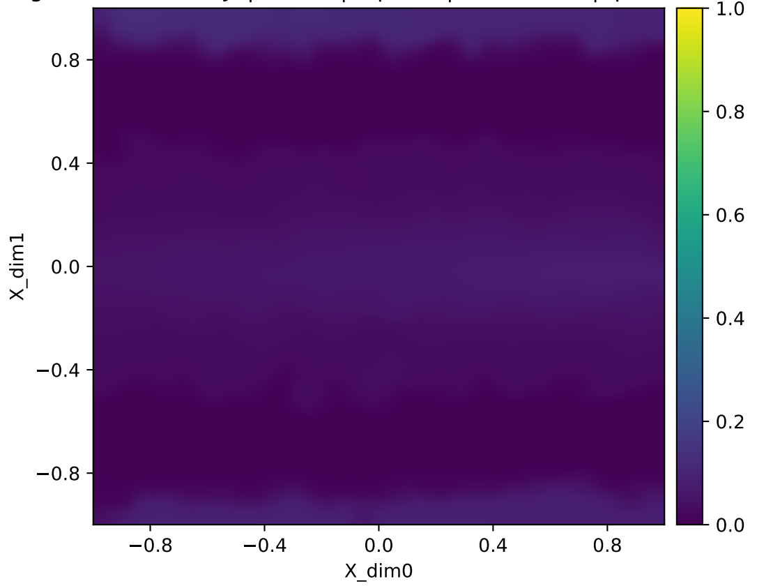
Forward map singular value smin(J) | ribbon | repeats | Y=radial1d | q=65 heatmap (fixed [0,1])
