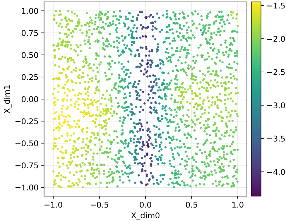
Forward map log10 singular value log10(smin(J)) | pinch | repeats | Y=corr2d | q=16385 (adaptive)
