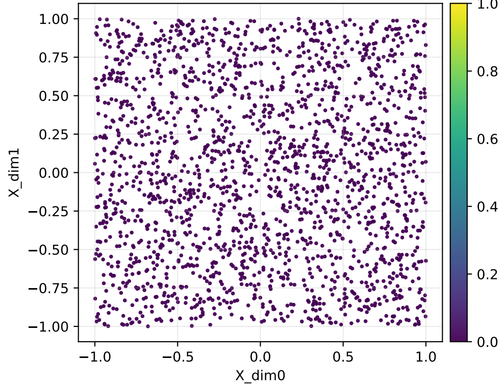
Forward map log10 singular value log10(smin(J)) | fold | repeats | Y=radial1d | q=65 (fixed [0,1])
