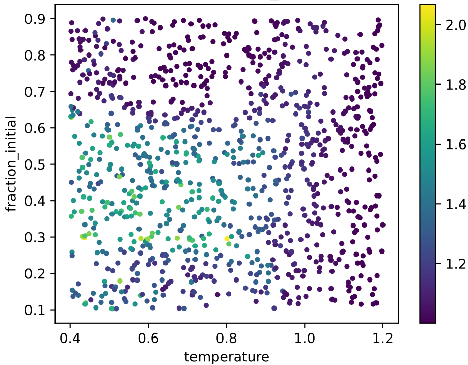
corr2d: effrank(K_gate)
