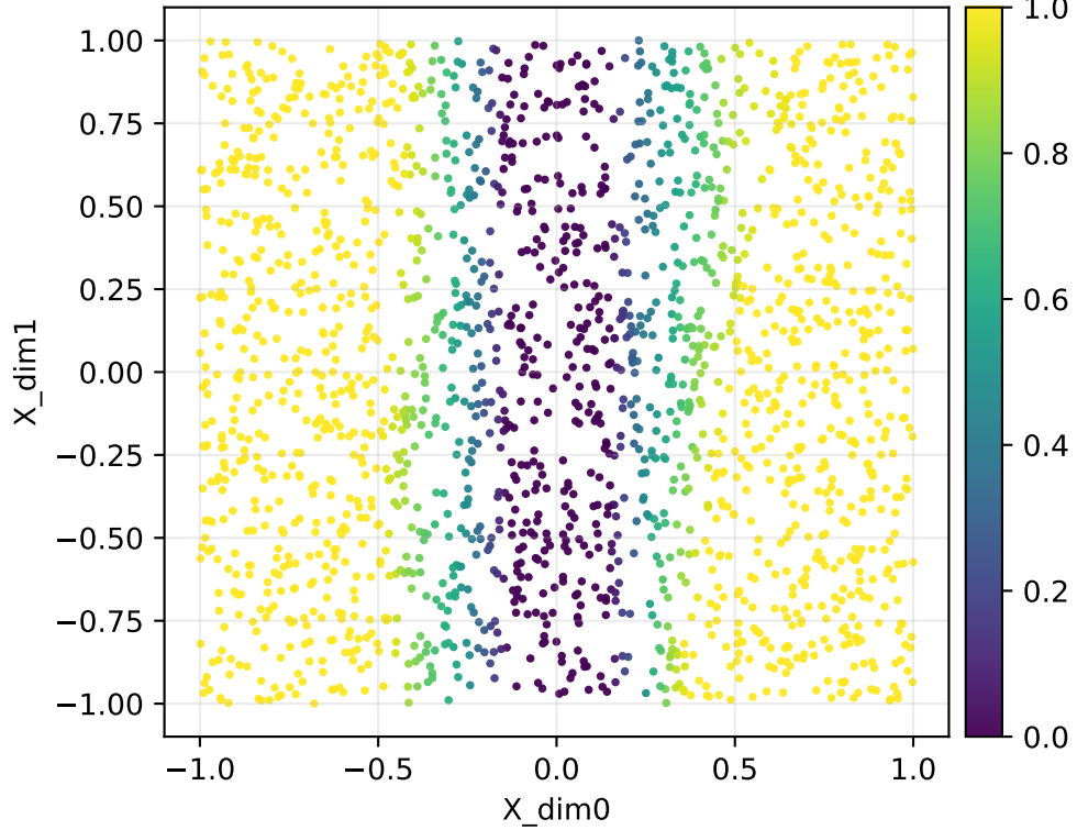
Forward map log10 singular value log10(smin(J)) | pinch | fixed | Y=raw_flat | q=16384 (fixed [0,1])
