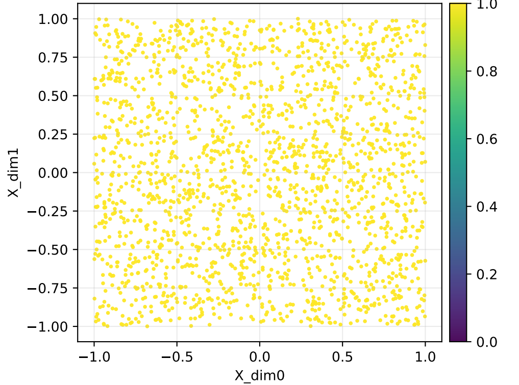
Forward map singular value \text{smin}(J) | nowarp | fixed | Y=raw_flat | q=16384 (fixed [0,1])
