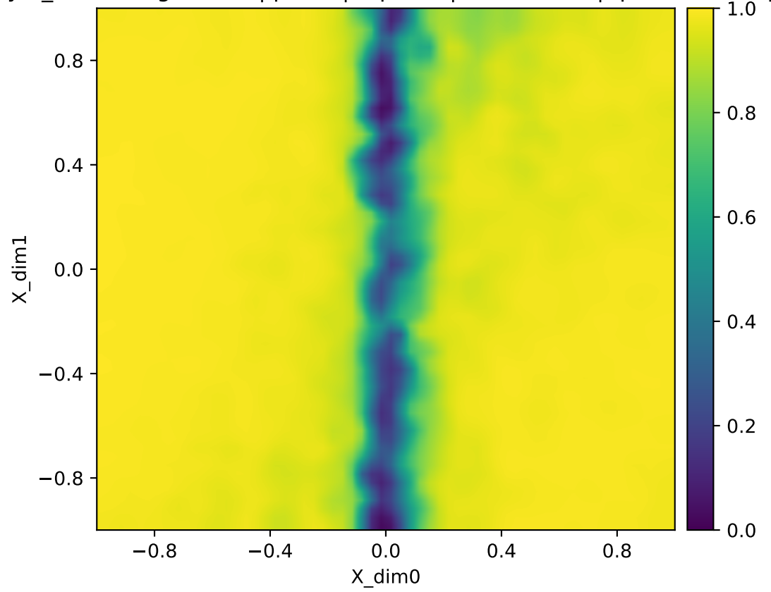
Inverse locality e_inv (Y-neigh -> X) | pinch | repeats | Y=radial1d | q=65 heatmap (fixed [0,1])
