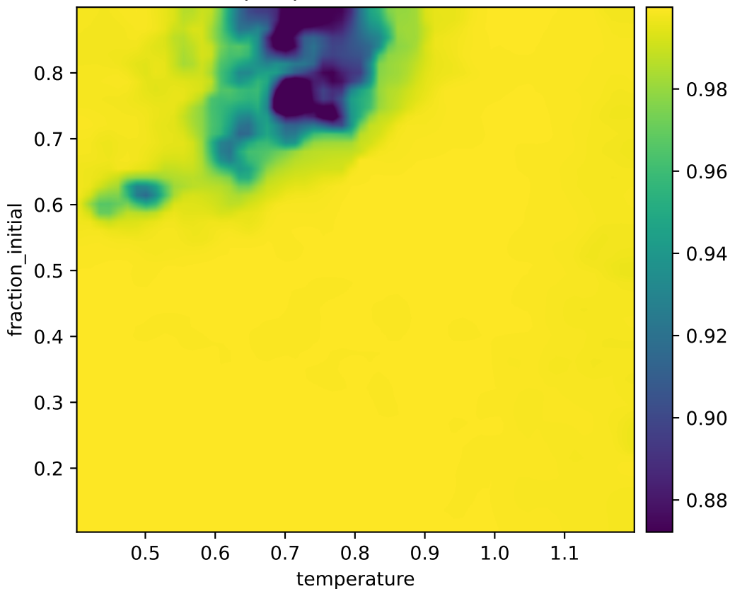
corr2d: heatmap explained fraction (baseline KRR)
