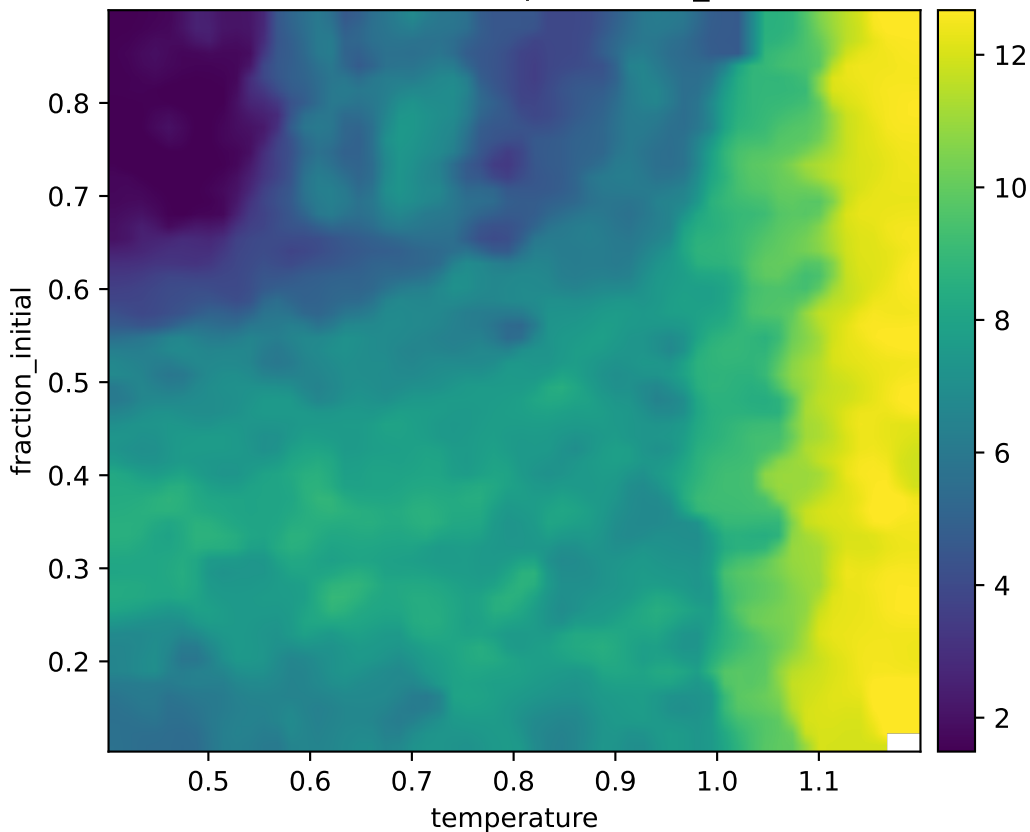
radial1d: heatmap effective_rank
