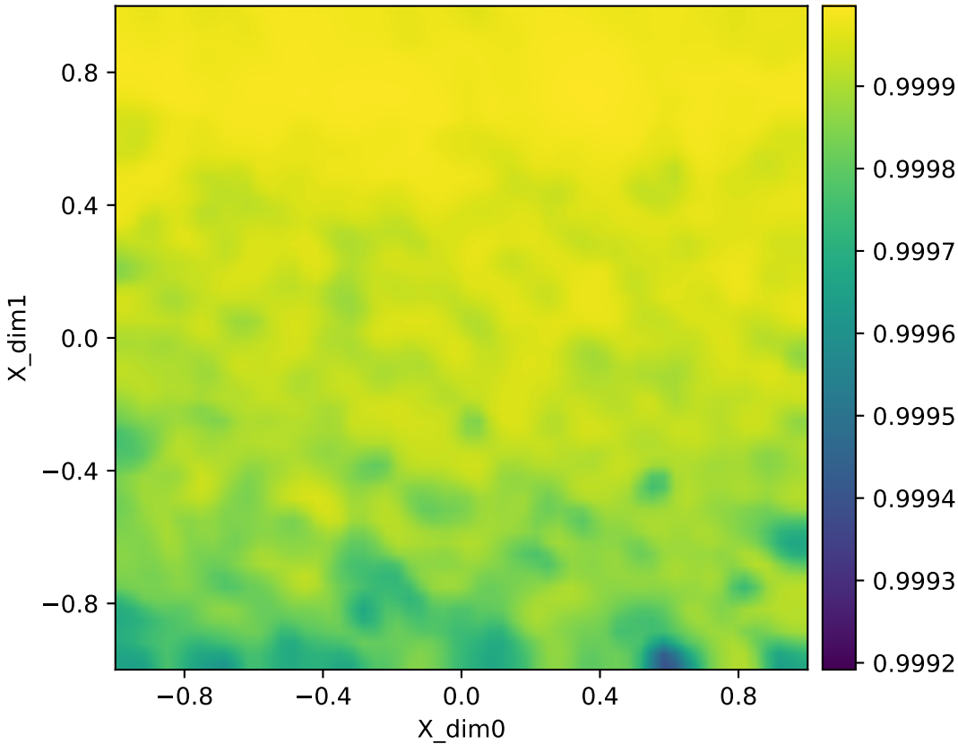
Inverse locality e_inv (Y-neigh -> X) | nowarp | fixed | Y=row_flat | q=16384 heatmap (adaptive)
