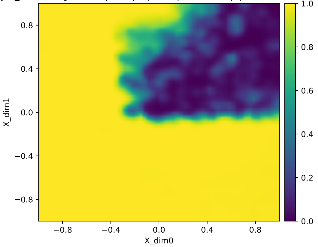
Inverse locality e_inv (Y-neigh -> X) | fold | repeats | Y=corr2d | q=16385 heatmap (fixed [0,1])
