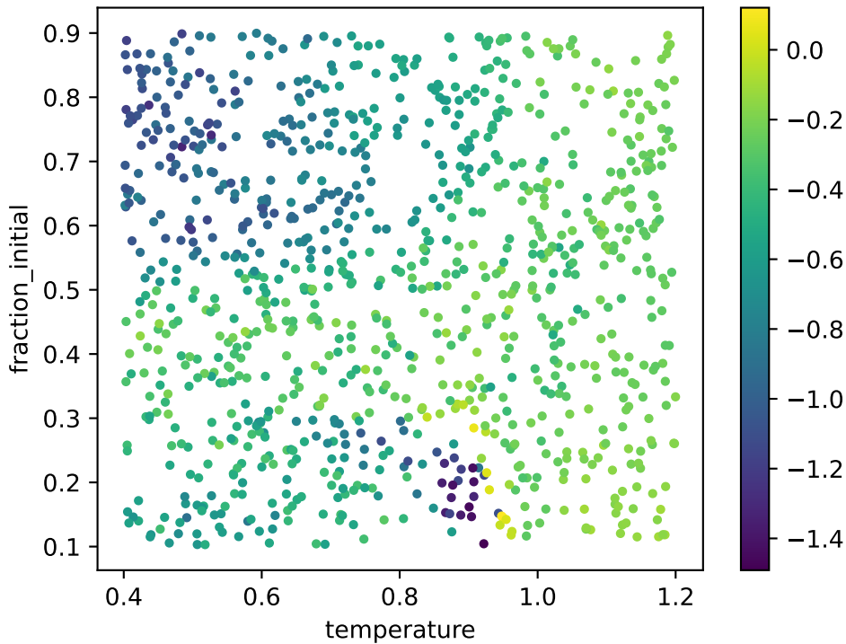
corr2d: log10 local X energy tr(X)
