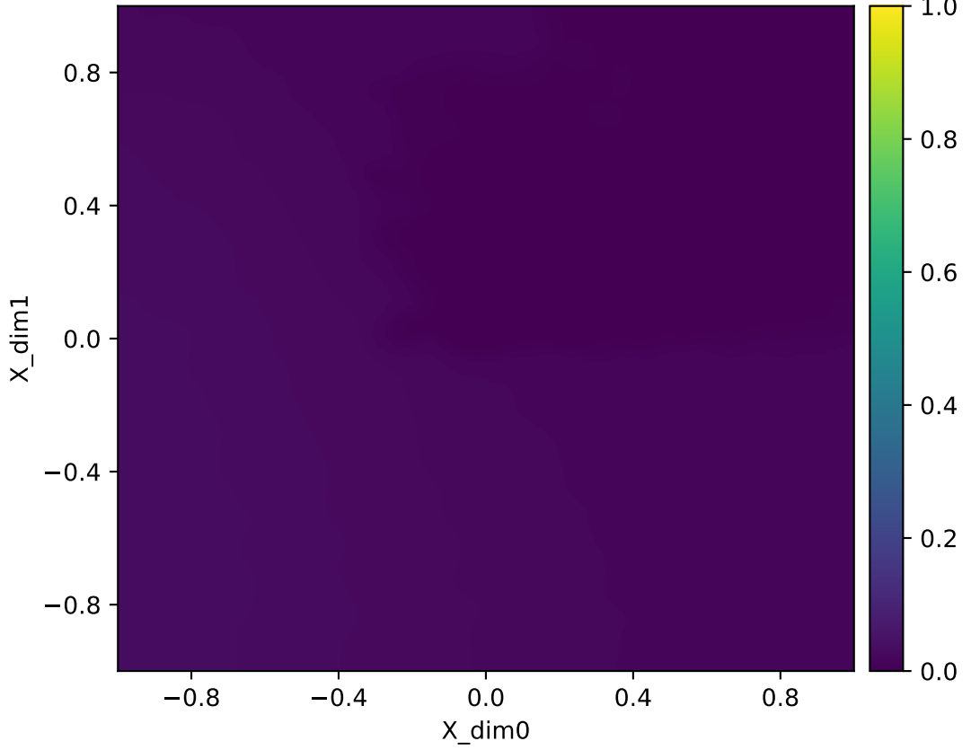
Forward map singular value smin(J) | fold | repeats | Y=corr2d | q=16385 heatmap (fixed [0,1])
