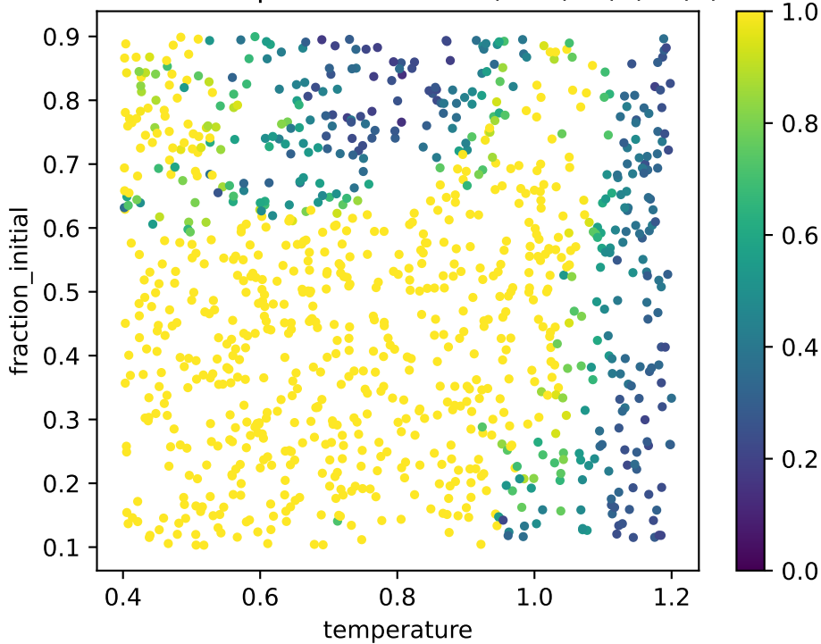
corr2d: unexplained fraction (LOO) \text{tr}(\mathbf{R})/\text{tr}(\mathbf{X})
