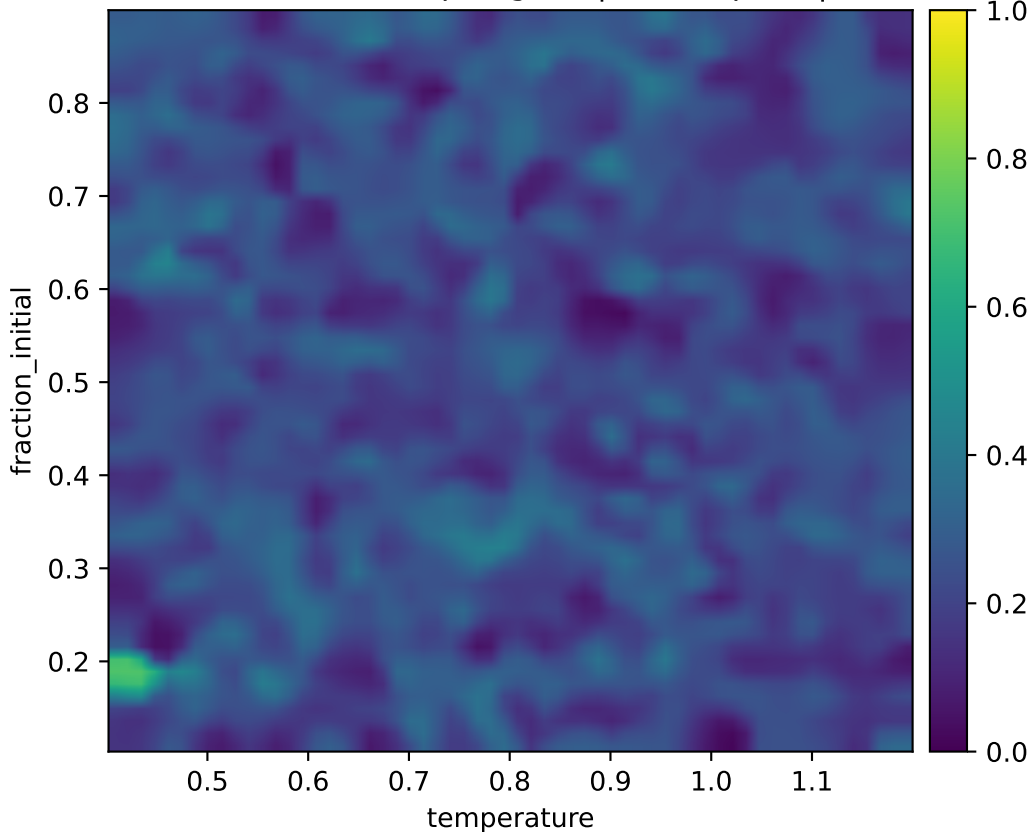
corr2d: heatmap align = |\mathbf{v}_0^T \sqrt{\mathbf{w}}|
