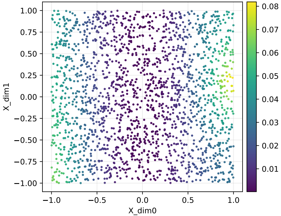
Forward map singular value \text{smin}(J) | pinch | repeats | Y=\text{radial1d} | q=65 (adaptive)
