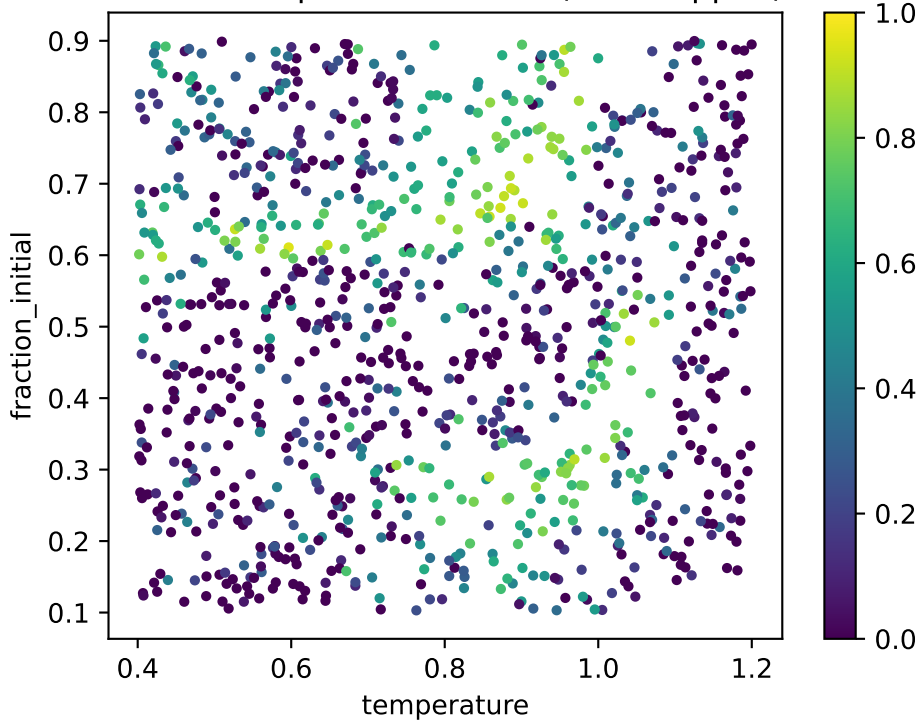
radial1d: explained fraction (rank-capped)
