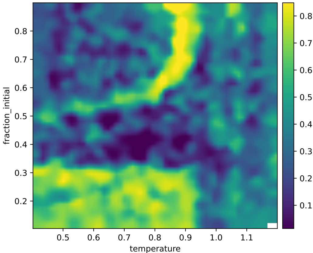
corr2d: heatmap null-calibrated explained fraction
