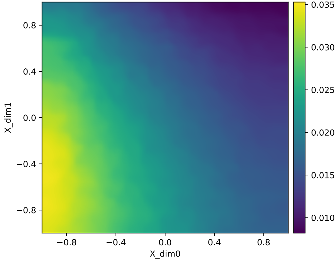
Forward map singular value \text{smin}(J) | nowarp | repeats | Y=corr2d | q=16385 heatmap (adaptive)
