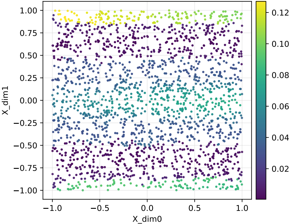
Forward map singular value \text{smin}(J) | ribbon | repeats | Y=\text{radial1d} | q=65 (adaptive)
