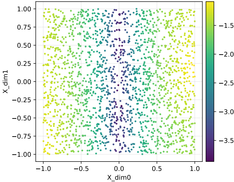
Forward map log10 singular value log10(smin(J)) | pinch | repeats | Y=radial1d | q=65 (adaptive)
