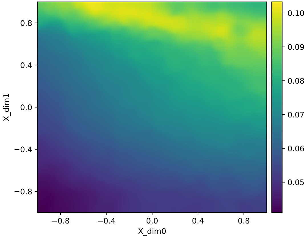
Forward map singular value \text{smn}(J) | nowarp | repeats | Y=radial1d | q=65 heatmap (adaptive)
