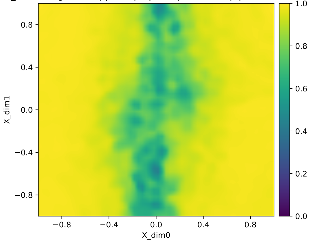
Inverse locality e_inv (Y-neigh -> X) | pinch | repeats | Y=corr2d | q=16385 heatmap (fixed [0,1])
