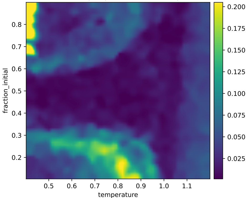
corr2d: heatmap explained fraction (laplacian)
