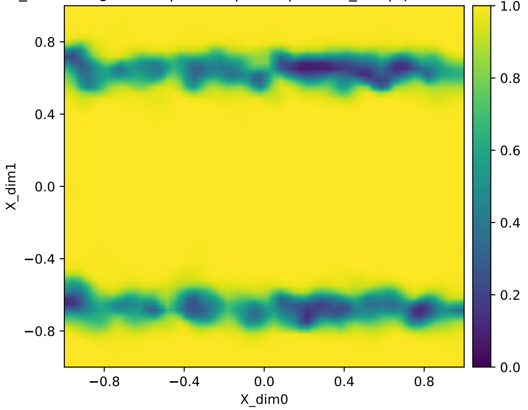
Inverse locality e_inv (Y-neigh -> X) | ribbon | fixed | Y=raw_flat | q=16384 heatmap (fixed [0,1])
