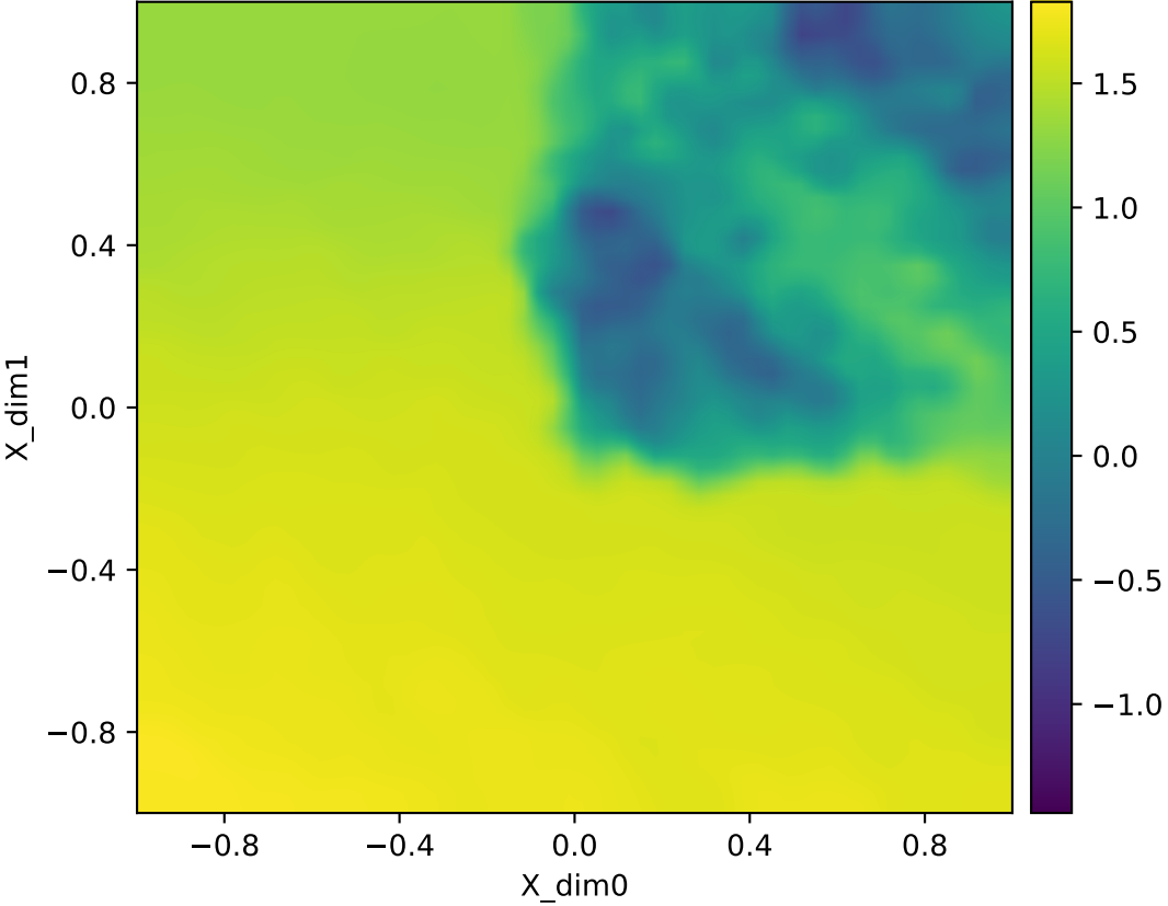
Forward map log10 singular value log10(smin(J)) | fold | fixed | Y=raw_flat | q=16384 heatmap (adaptive)
