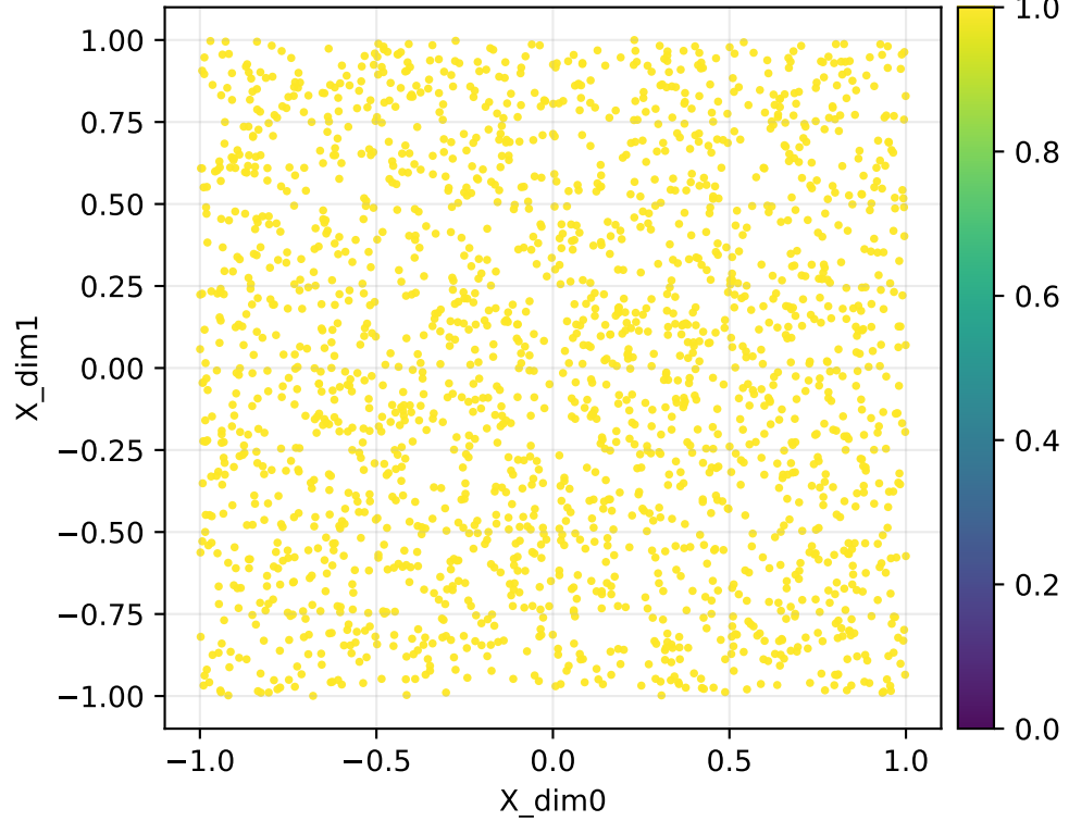
Forward map log10 singular value log10(smin(J)) | nowarp | fixed | Y=raw_flat | q=16384 (fixed [0,1])
