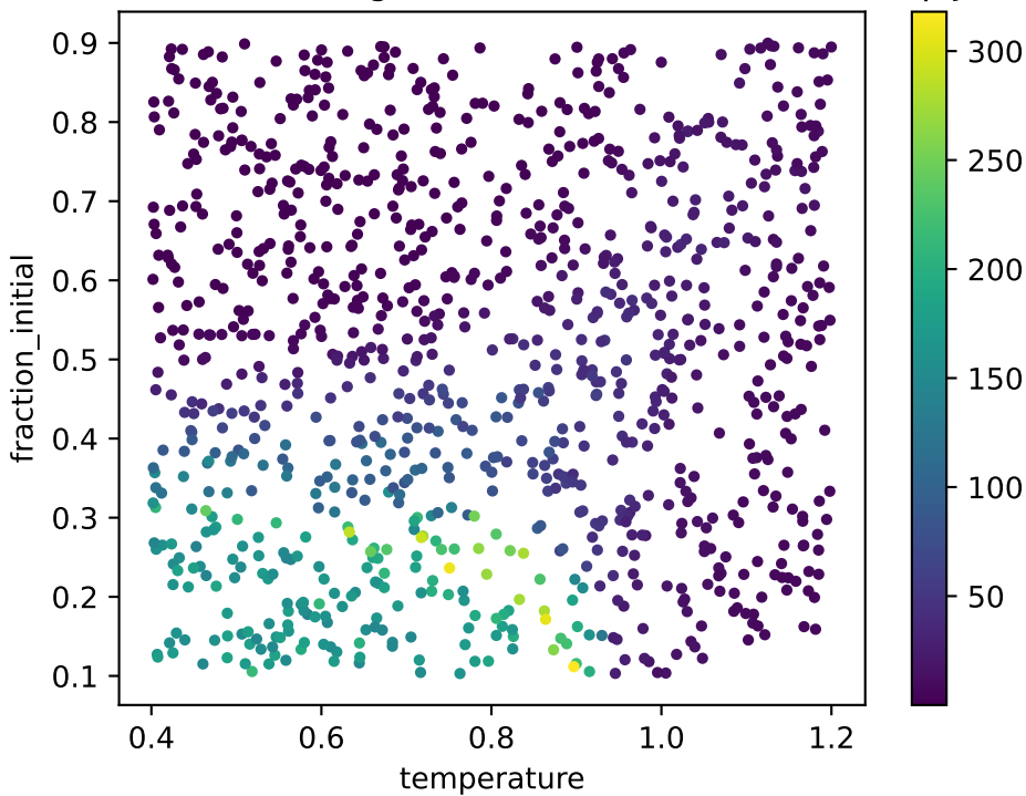
corr2d: smallest singular value of local forward map J
