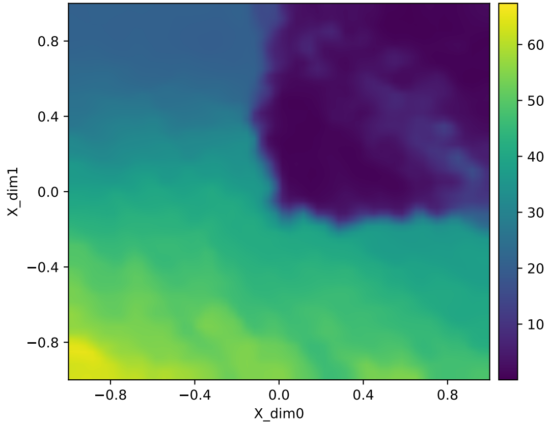
Forward map singular value \text{smin}(J) | fold | fixed | Y=raw_flat | q=16384 heatmap (adaptive)
