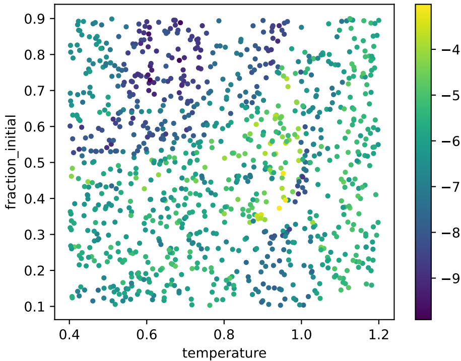
radial1d: logdet local Cov(X) (ridge-stabilized)
