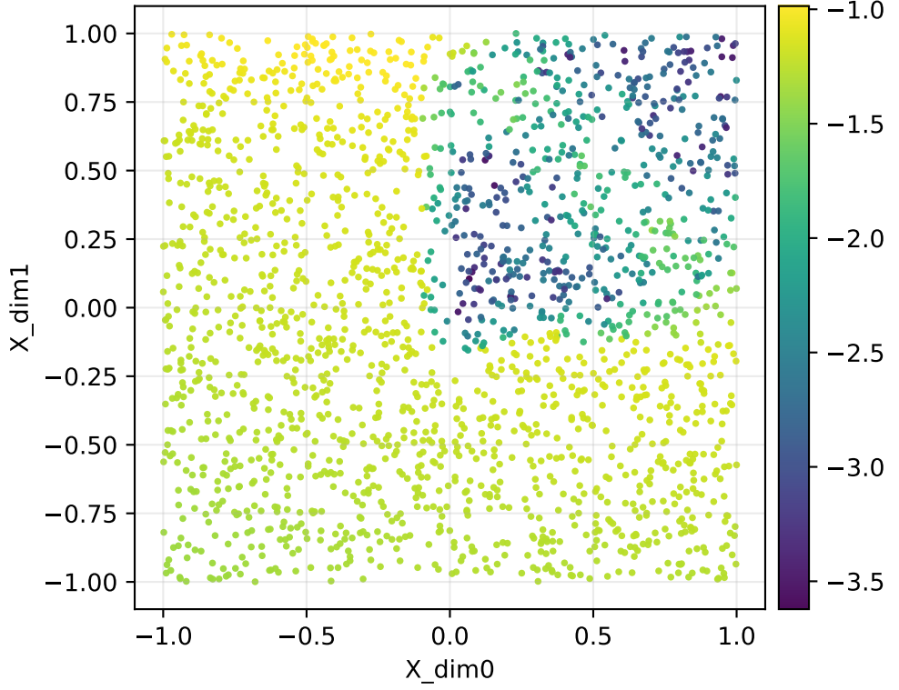
Forward map log10 singular value log10(smin(J)) | fold | repeats | Y=radial1d | q=65 (adaptive)
