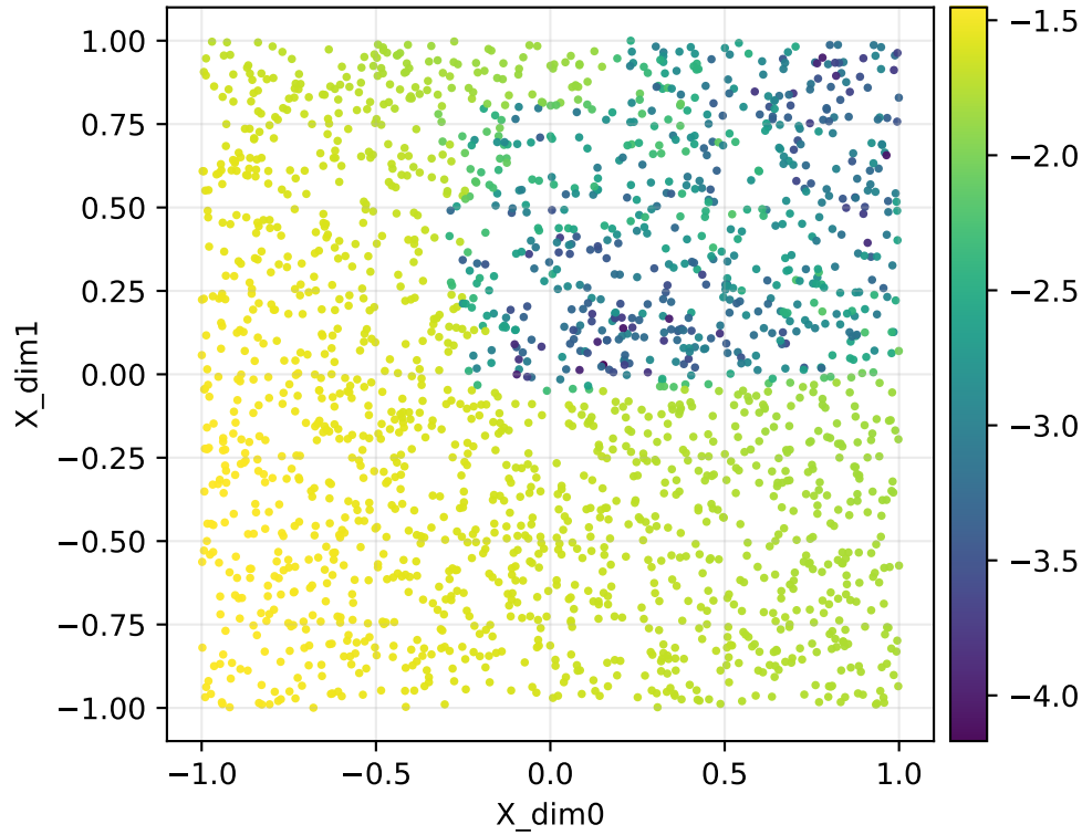
Forward map log10 singular value log10(smin(J)) | fold | repeats | Y=corr2d | q=16385 (adaptive)
