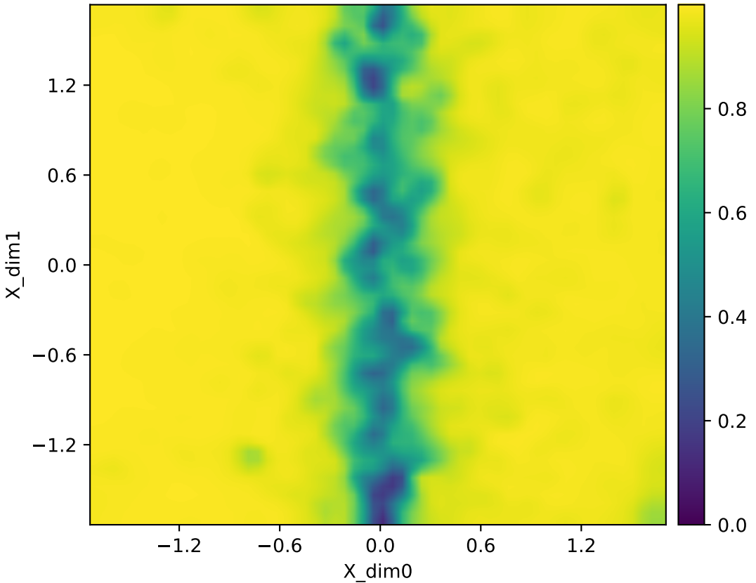
Inverse locality e_inv (Y-neigh -> X) | pinch | repeats | Y=radial1d | q=65 heatmap (adaptive)
