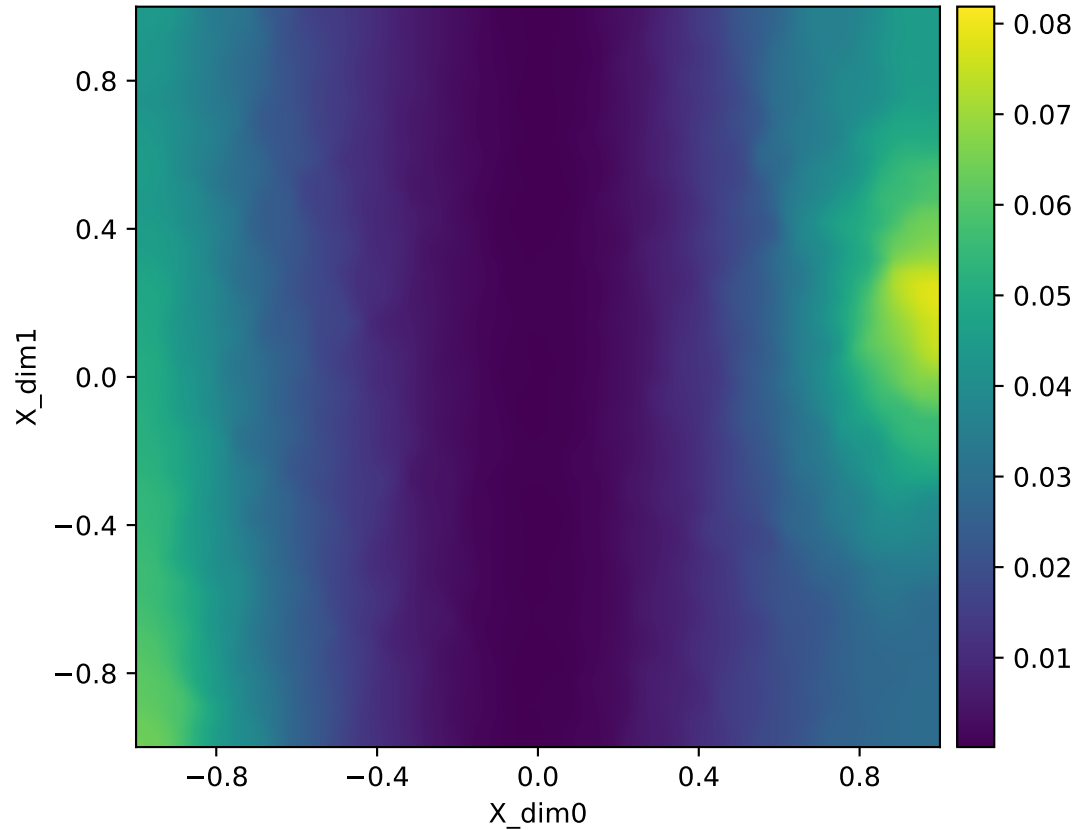
Forward map singular value \text{smin}(J) | pinch | repeats | Y=\text{radial1d} | q=65 heatmap (adaptive)
