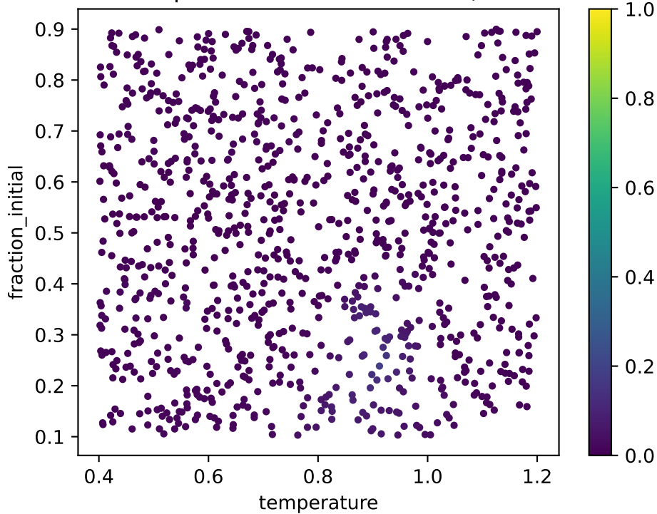
corr2d: 2nd-direction explained fraction lambda2 (2D controllability gate)
