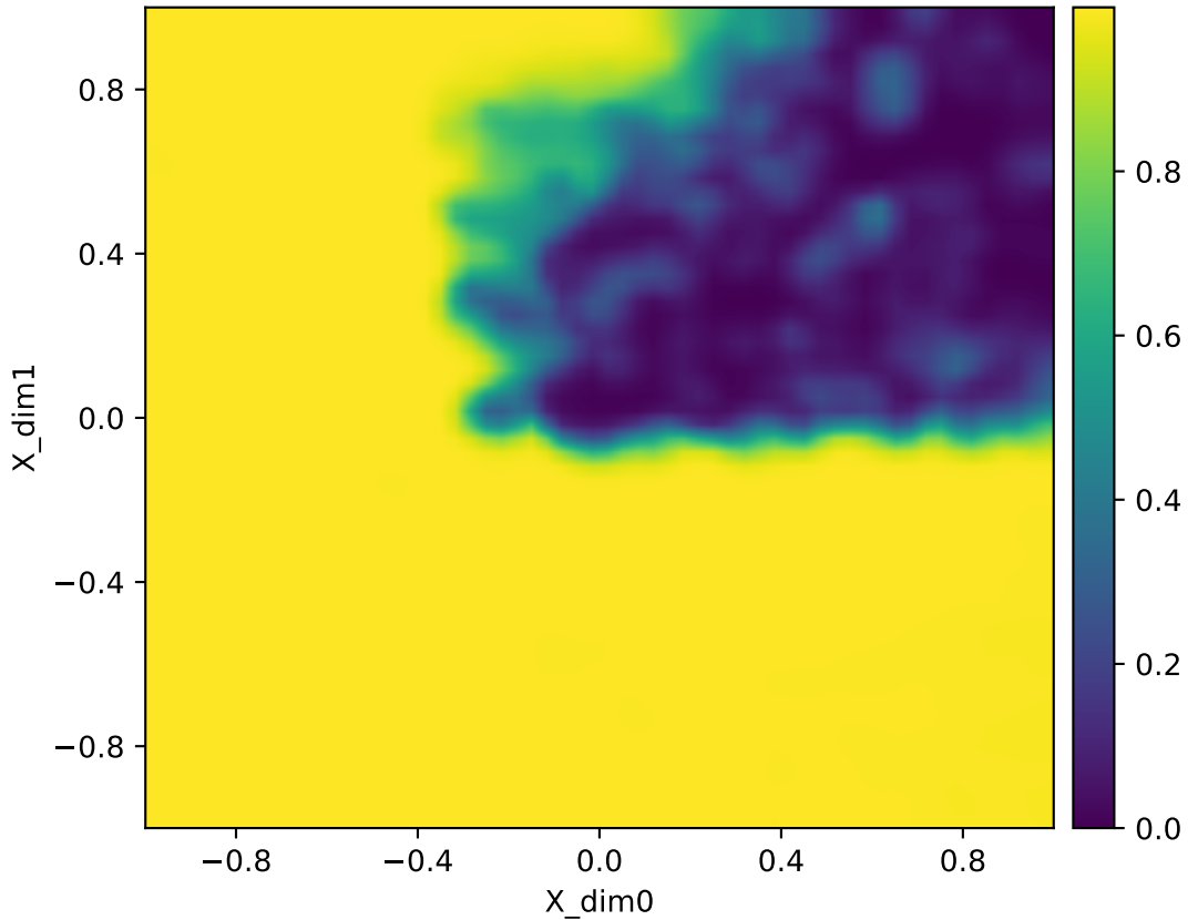
Inverse locality e_inv (Y-neigh -> X) | fold | repeats | Y=corr2d | q=16385 heatmap (adaptive)
