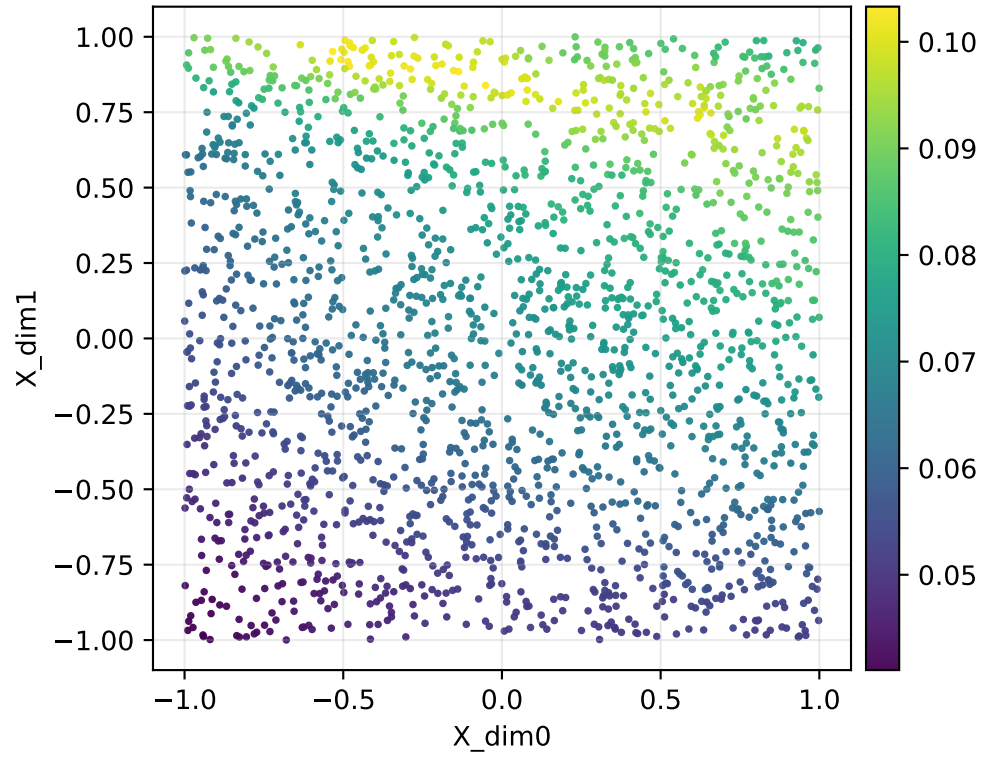
Forward map singular value \text{smin}(J) | nowarp | repeats | Y=radial1d | q=65 (adaptive)
