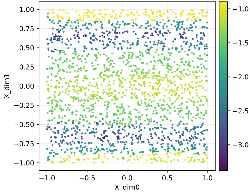
Forward map log10 singular value log10(smin(J)) | ribbon | repeats | Y=radial1d | q=65 (adaptive)
