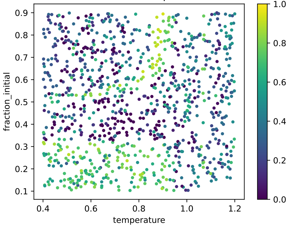
corr2d: null-calibrated explained fraction
