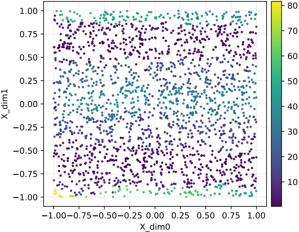
Forward map singular value \text{smin}(J) | ribbon | fixed | Y=raw_flat | q=16384 (adaptive)
