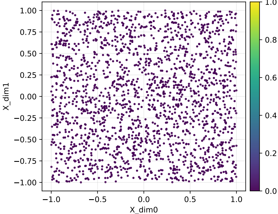
Forward map log10 singular value log10(smin(J)) | nowarp | repeats | Y=radial1d | q=65 (fixed [0,1])
