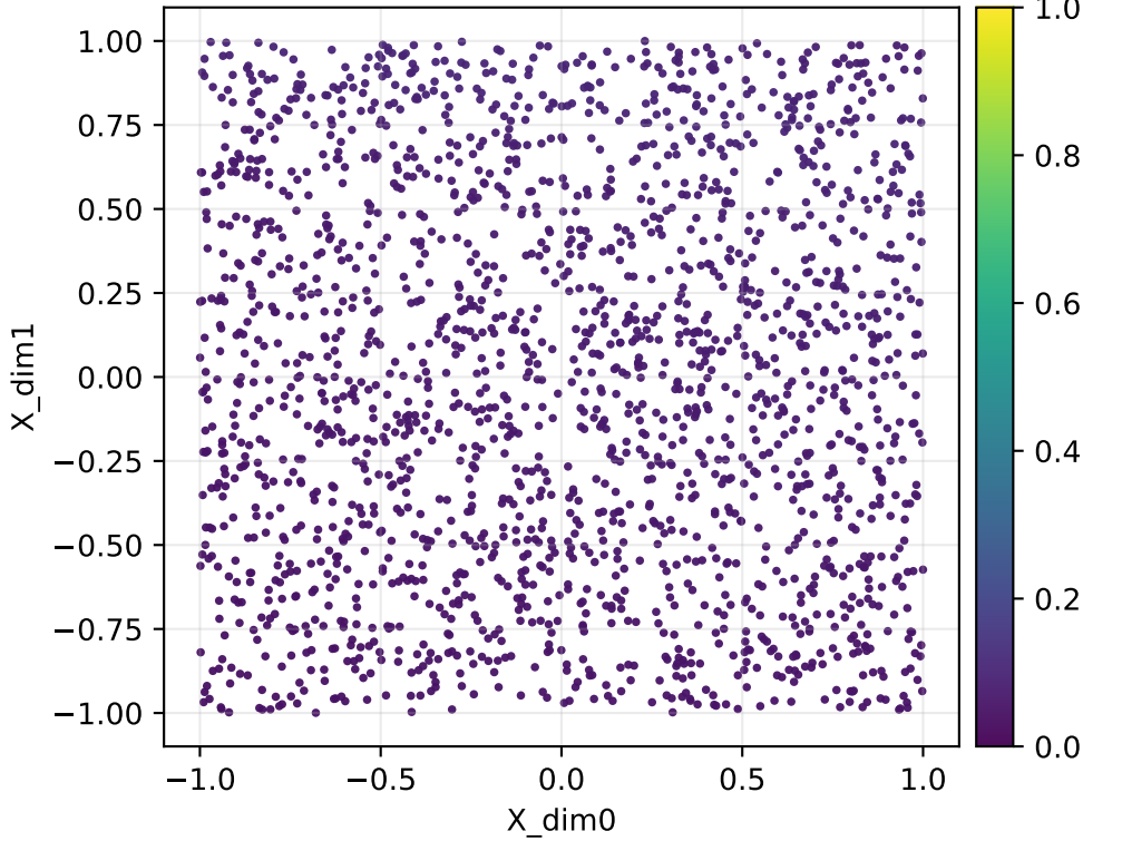
Forward map singular value \text{smin}(J) | nowarp | repeats | Y=radial1d | q=65 (fixed [0,1])
