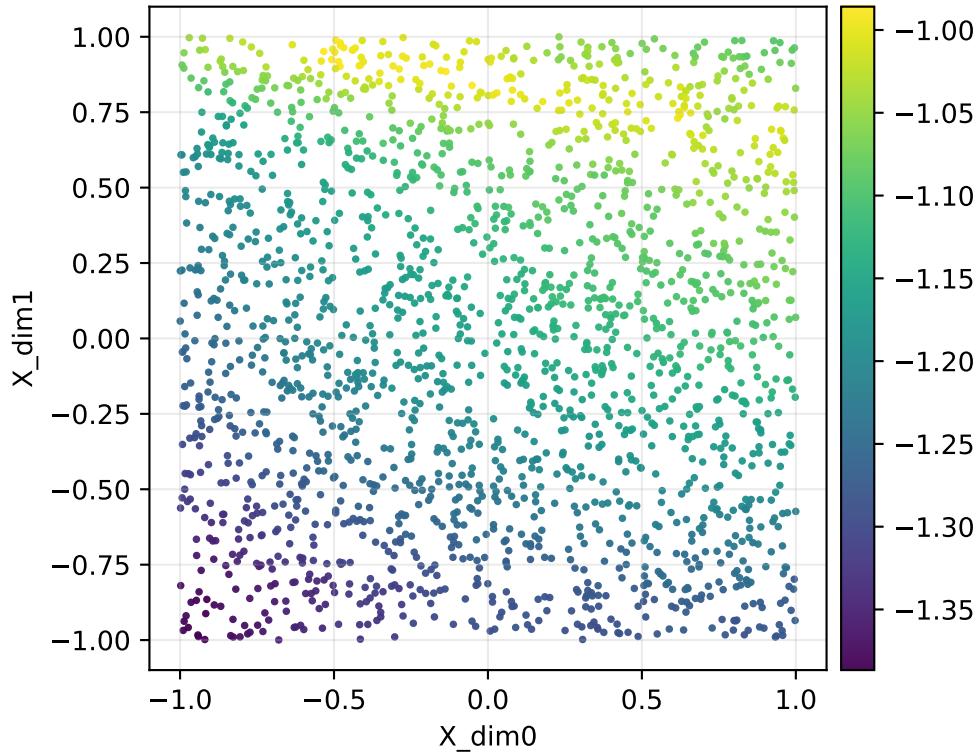
Forward map log10 singular value log10(smin(J)) | nowarp | repeats | Y=radial1d | q=65 (adaptive)
