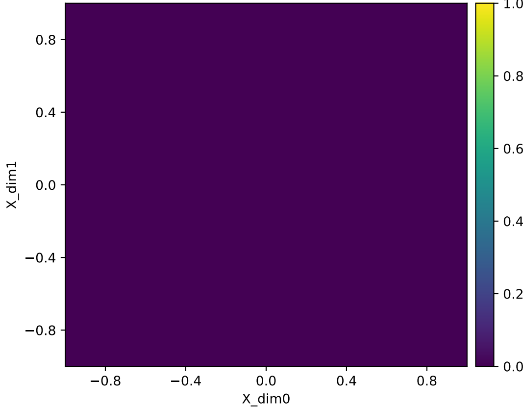
Forward map log10 singular value log10(smin(J)) | pinch | repeats | Y=corr2d | q=16385 heatmap (fixed [0,1])
