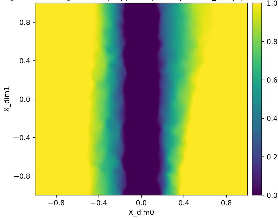
Forward map log10 singular value log10(smin(J)) | pinch | fixed | Y=raw_flat | q=16384 heatmap (fixed [0,1])
