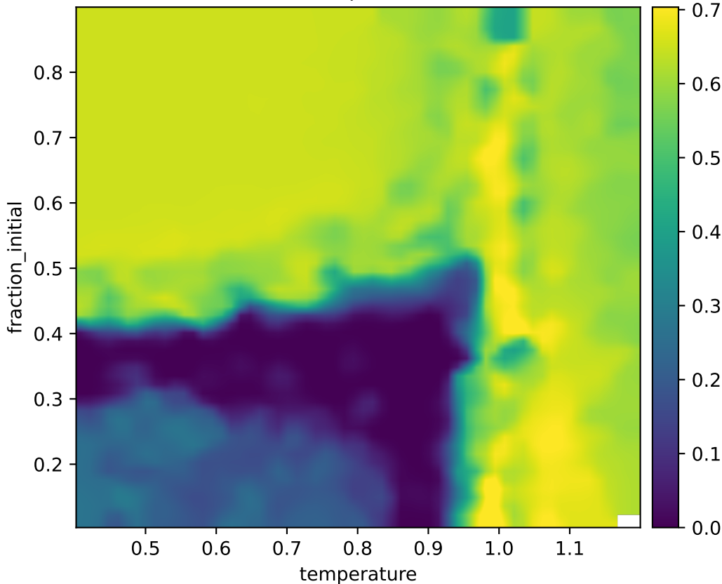
corr2d: heatmap worst retention
