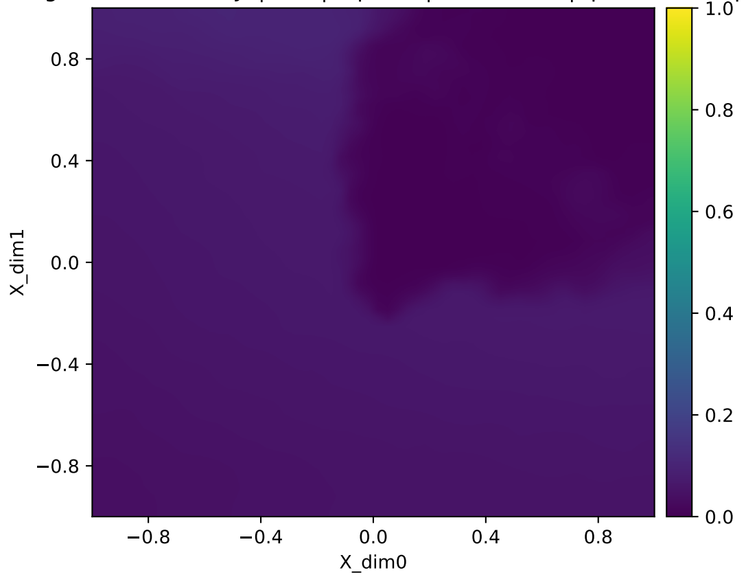
Forward map singular value smin(J) | fold | repeats | Y=radial1d | q=65 heatmap (fixed [0,1])
