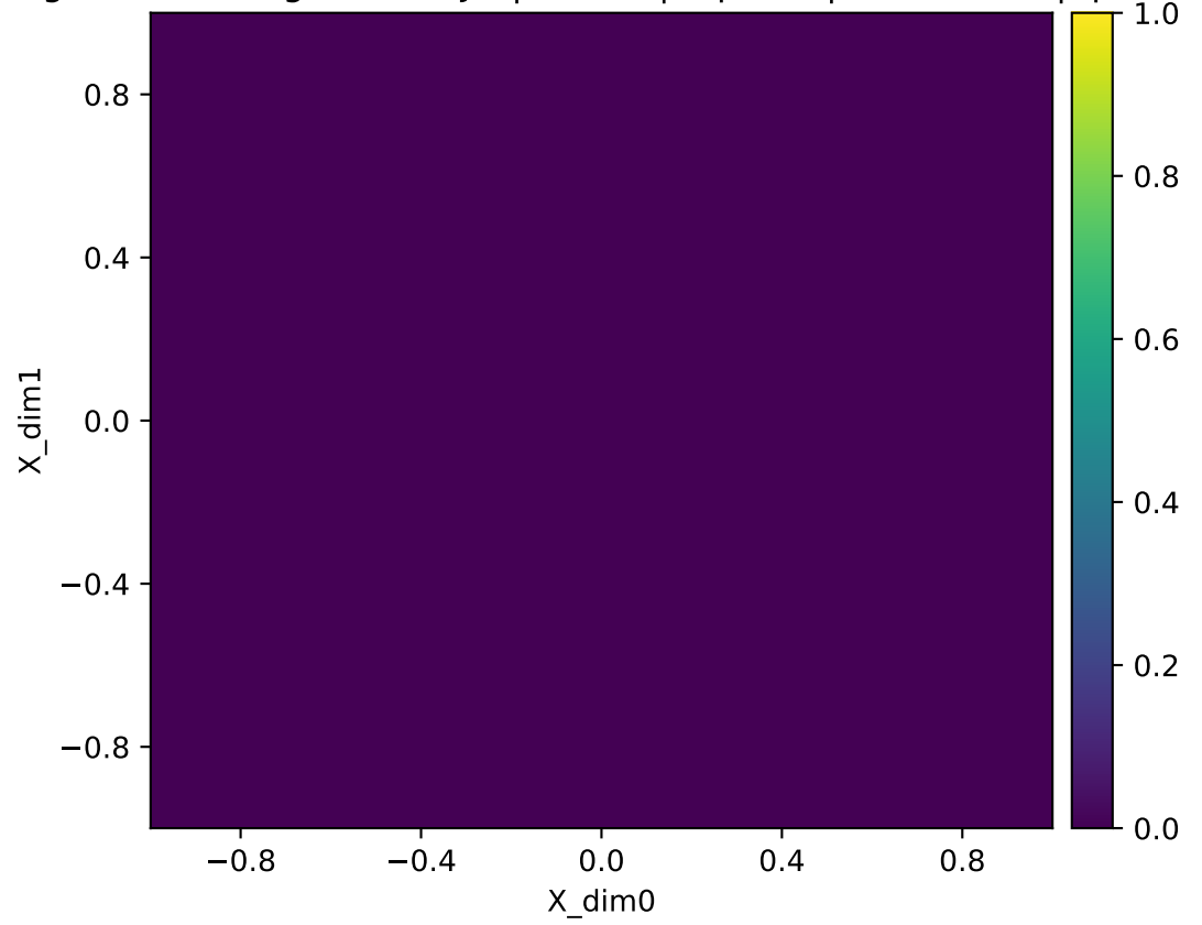
Forward map log10 singular value log10(smin(J)) | ribbon | repeats | Y=radial1d | q=65 heatmap (fixed [0,1])
