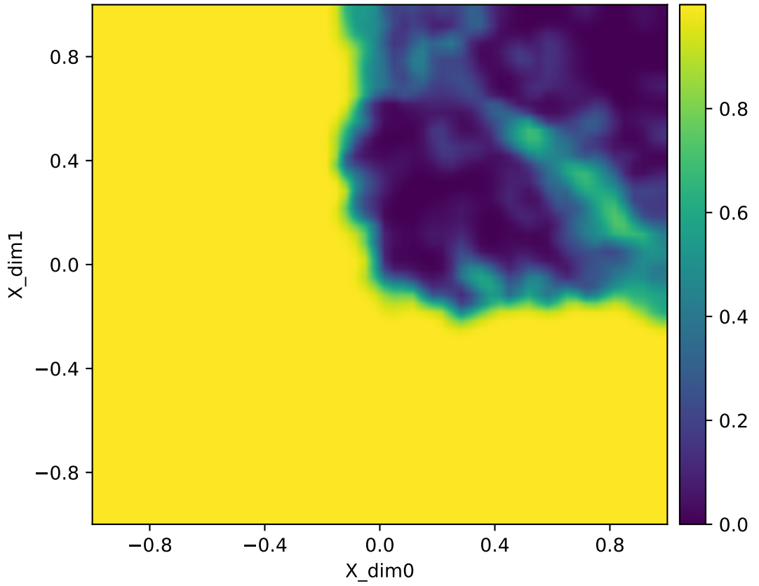
Inverse locality e_inv (Y-neigh -> X) | fold | fixed | Y=raw_flat | q=16384 heatmap (adaptive)
