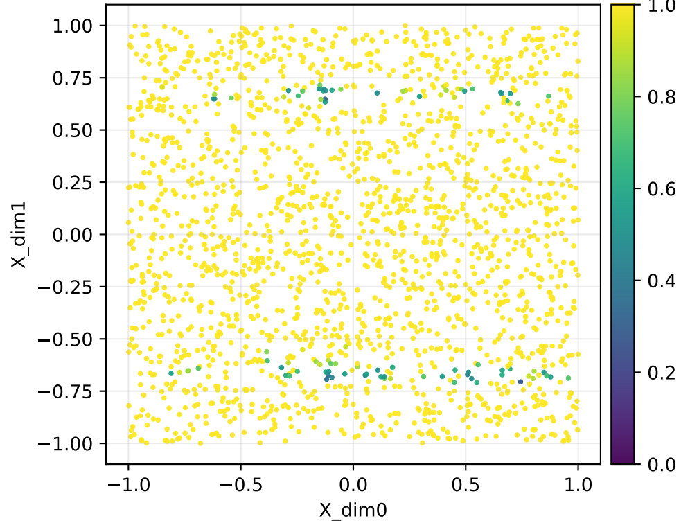
Forward map singular value \text{smin}(J) | ribbon | fixed | Y=raw_flat | q=16384 (fixed [0,1])
