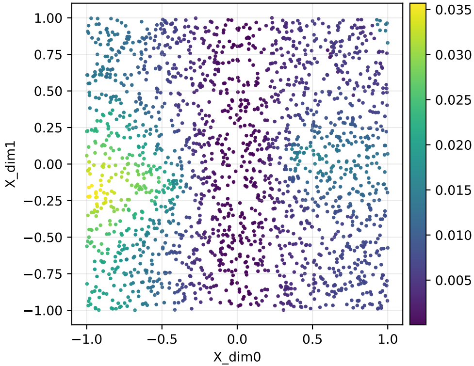
Forward map singular value s_{\min}(J) | pinch | repeats | Y=\text{corr2d} | q=16385 (adaptive)
