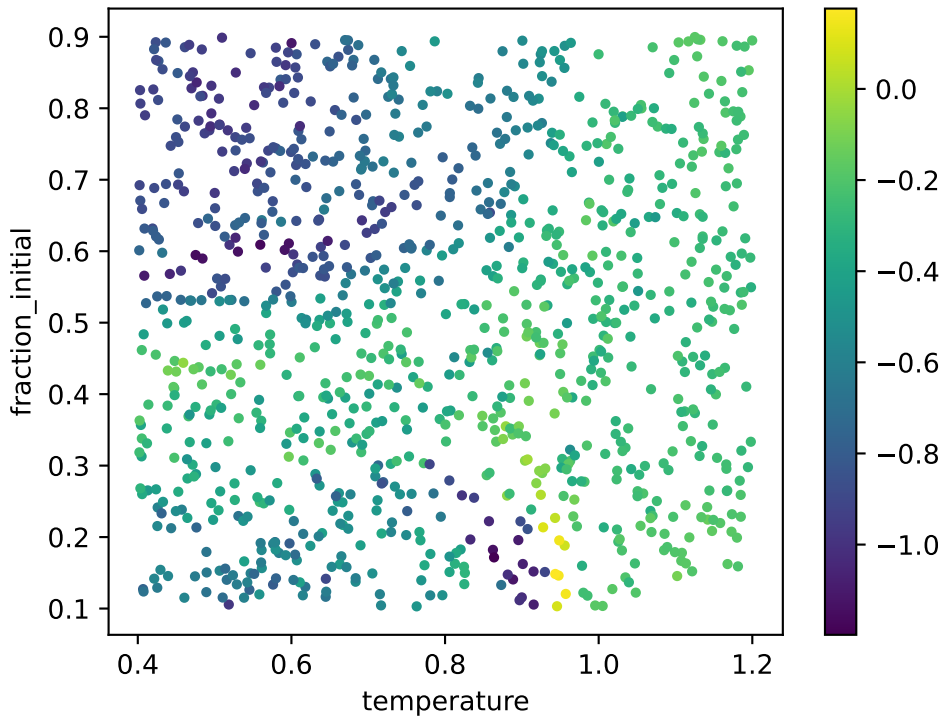
corr2d: log10 local X energy tr(X) (excitation)
