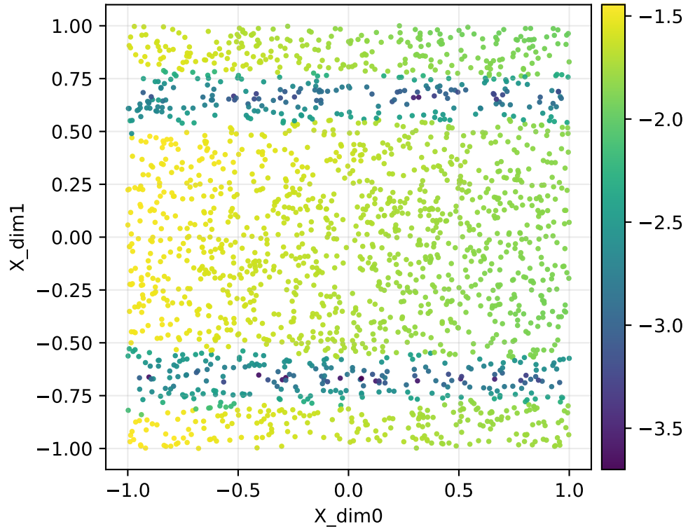
Forward map log10 singular value log10(smin(J)) | ribbon | repeats | Y=corr2d | q=16385 (adaptive)
