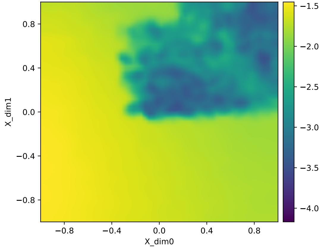
Forward map log10 singular value log10(smin(J)) | fold | repeats | Y=corr2d | q=16385 heatmap (adaptive)
