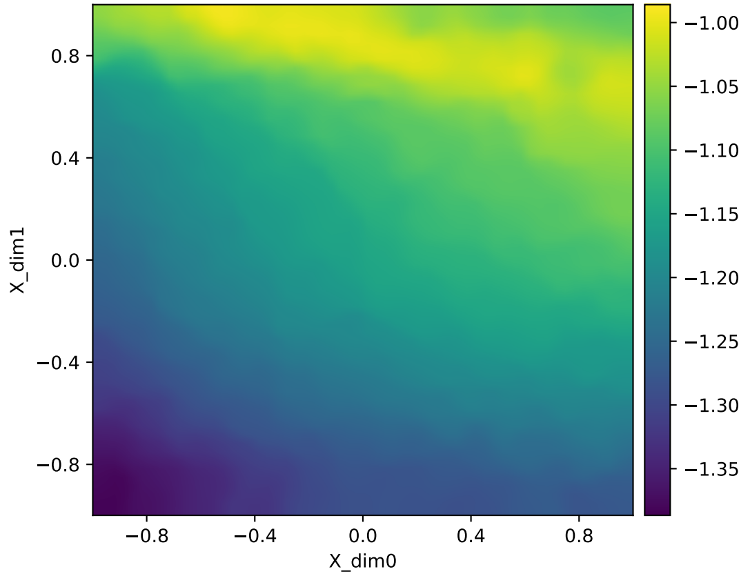
Forward map log10 singular value log10(smin(J)) | nowarp | repeats | Y=radial1d | q=65 heatmap (adaptive)
