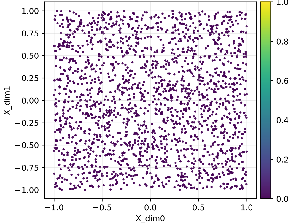
Forward map log10 singular value log10(smin(J)) | ribbon | repeats | Y=radial1d | q=65 (fixed [0,1])
