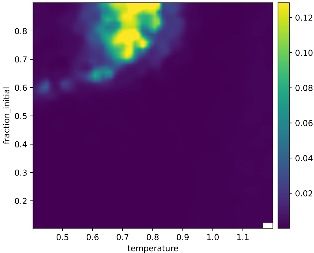
corr2d: heatmap unexplained fraction
