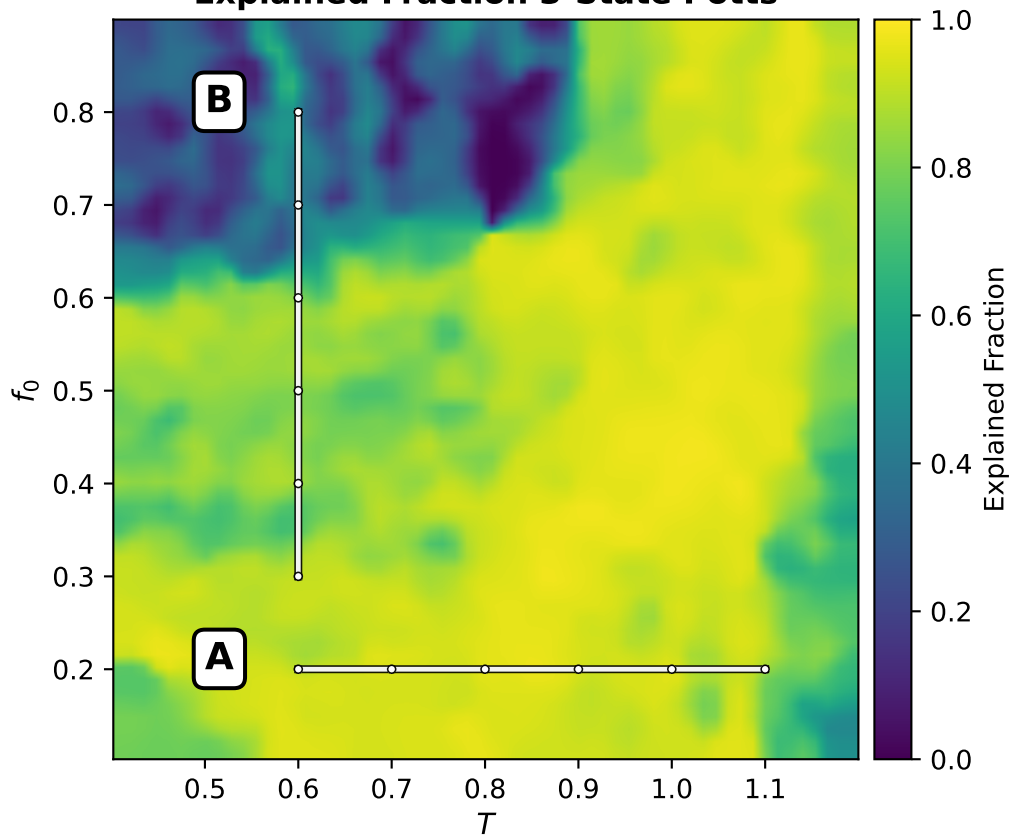
Explained Fraction 3-State Potts
