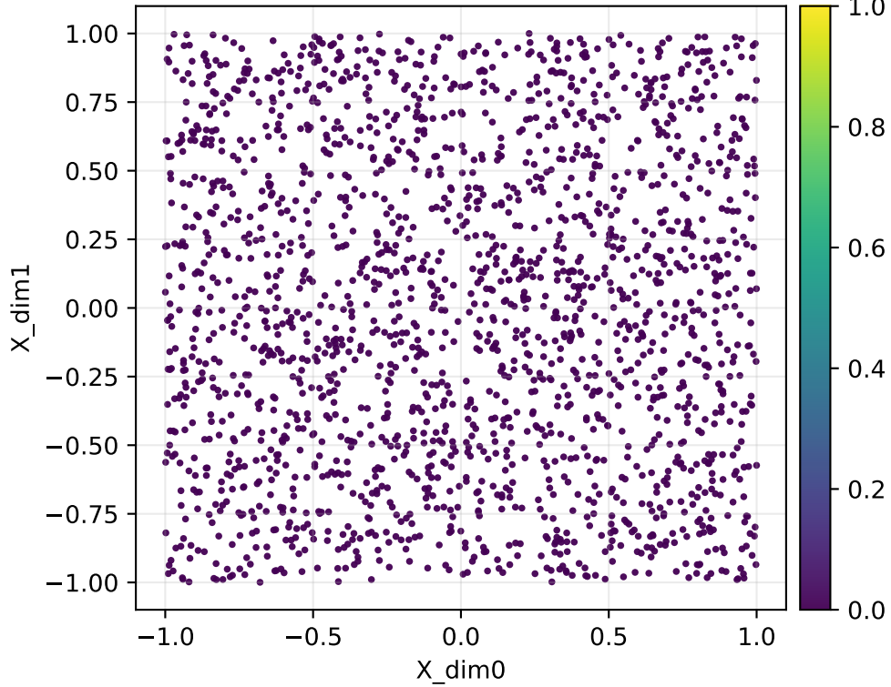
Forward map log10 singular value log10(smin(J)) | nowarp | repeats | Y=corr2d | q=16385 (fixed [0,1])
