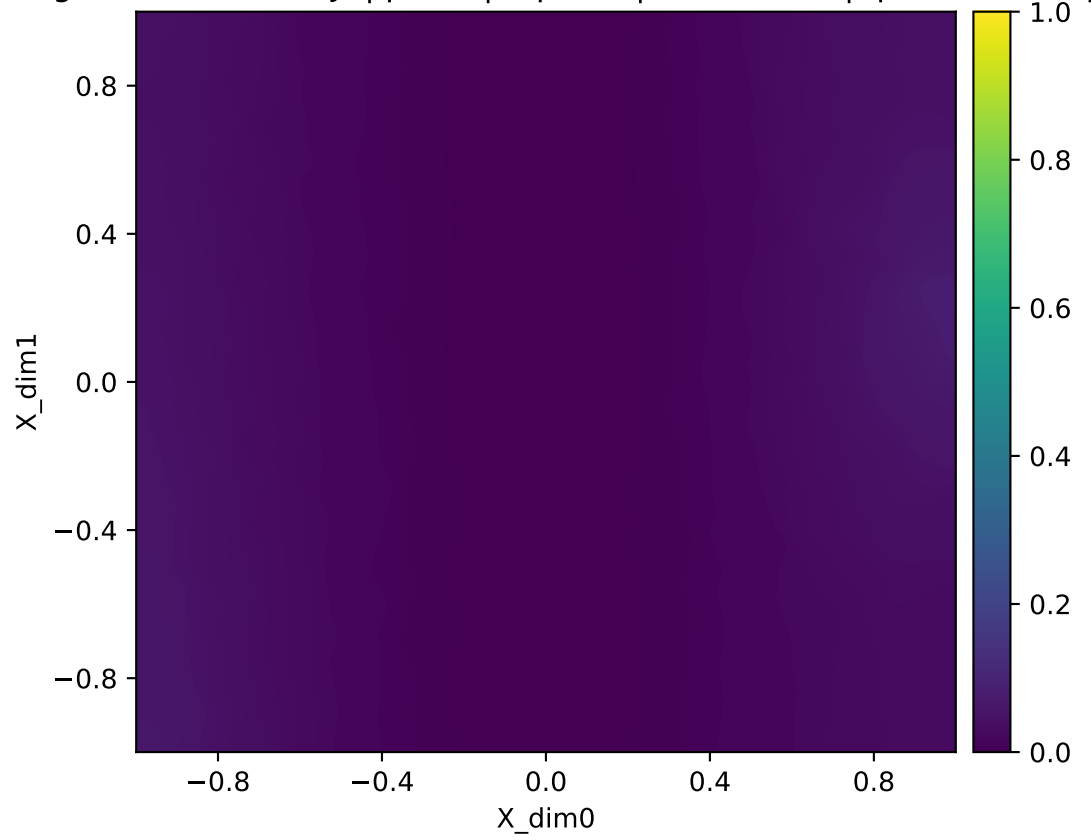
Forward map singular value smin(J) | pinch | repeats | Y=radial1d | q=65 heatmap (fixed [0,1])
