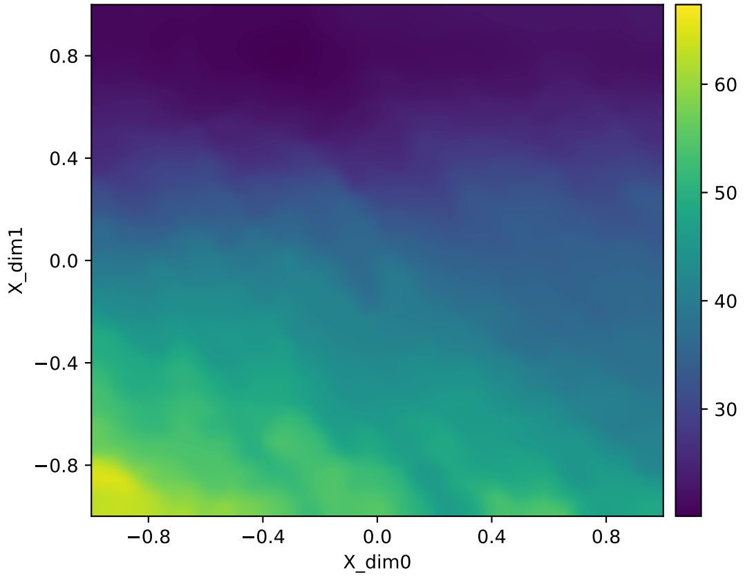
Forward map singular value smin(J) | nowarp | fixed | Y=raw_flat | q=16384 heatmap (adaptive)
