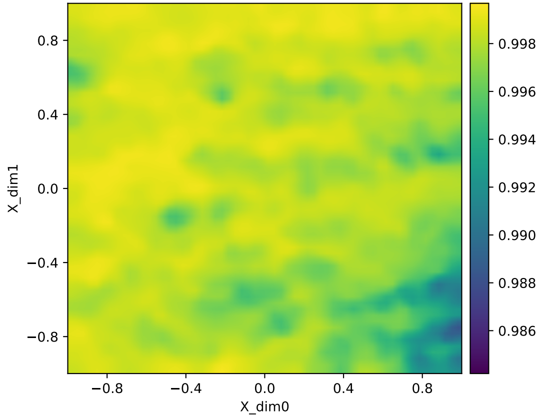
Inverse locality e_inv (Y-neigh -> X) | nowarp | repeats | Y=corr2d | q=16385 heatmap (adaptive)
