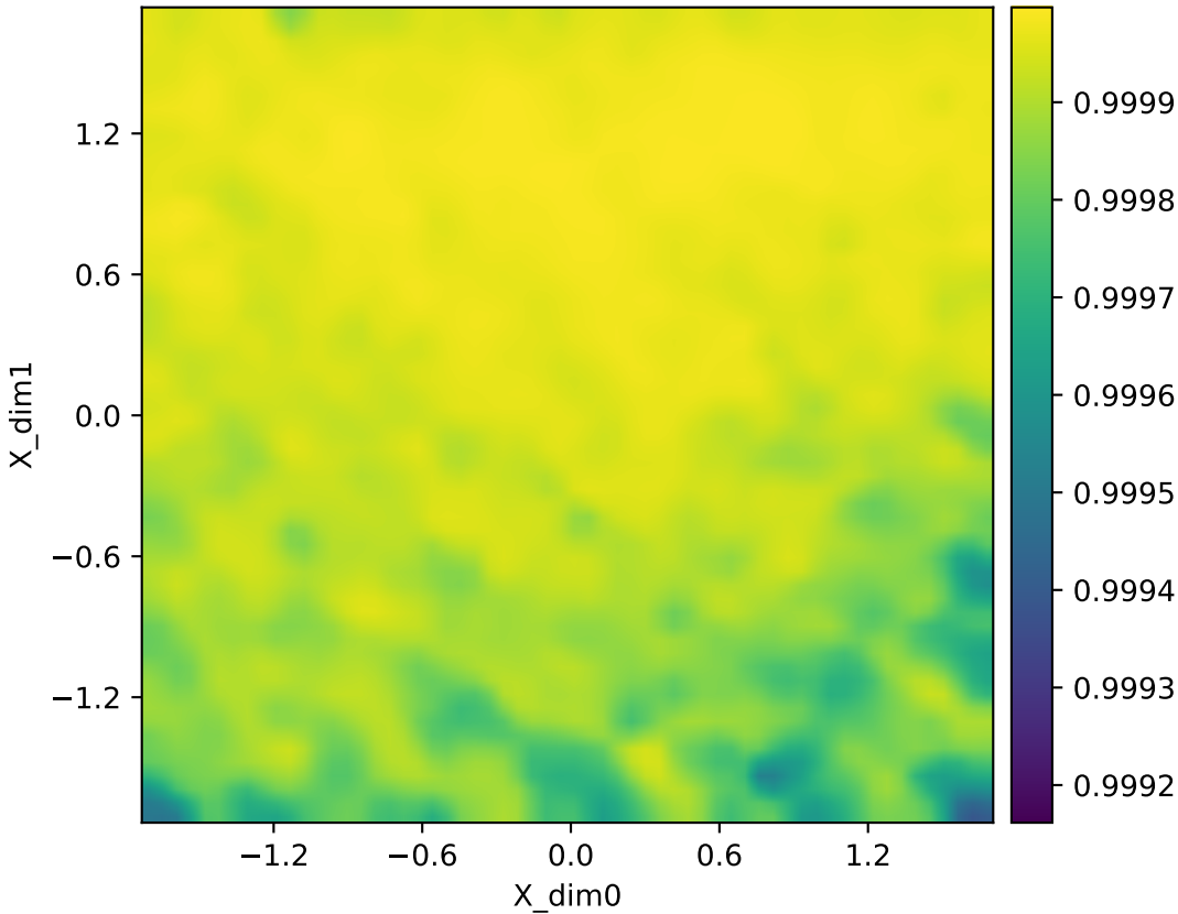
Inverse locality e_inv (Y-neigh -> X) | nowarp | fixed | Y=raw_flat | q=16384 heatmap (adaptive)
