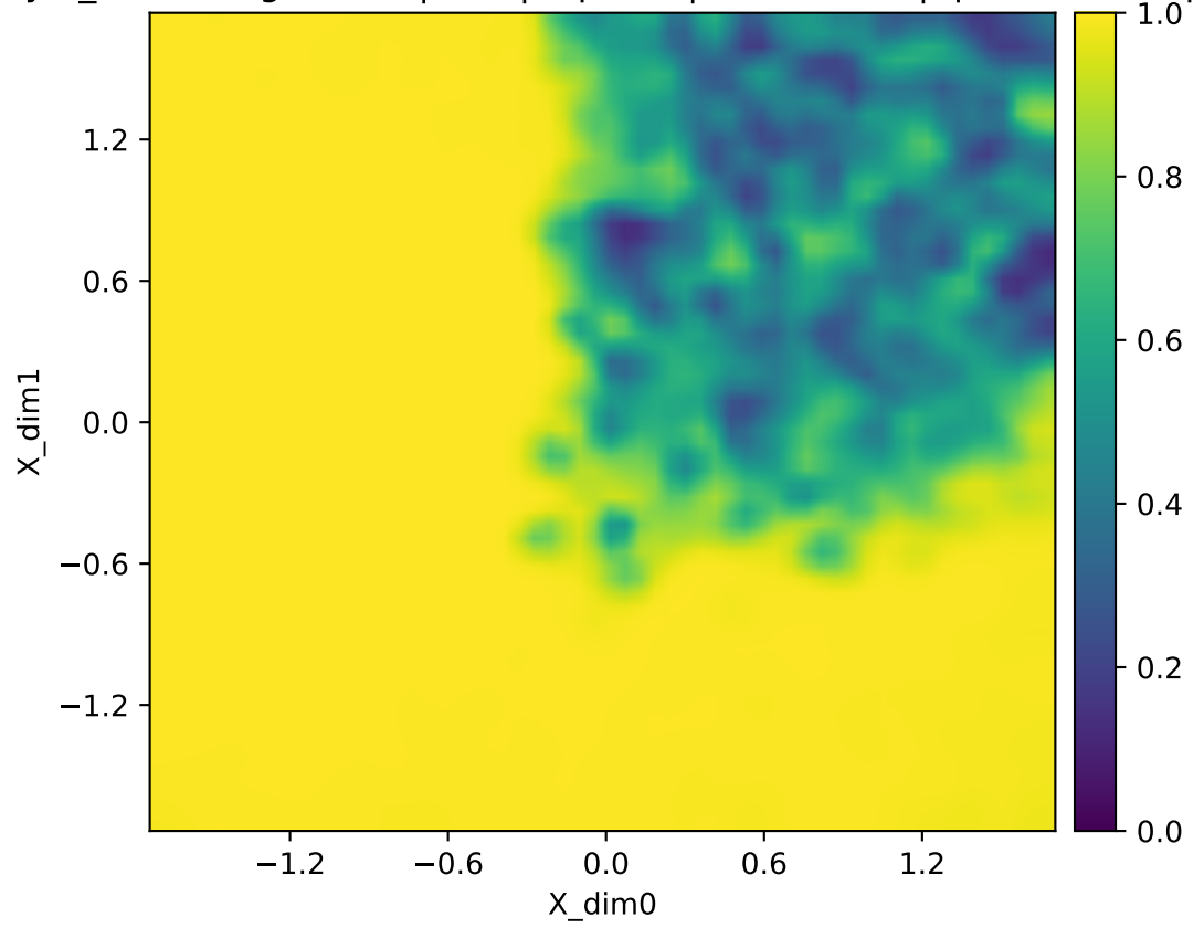
Inverse locality e_inv (Y-neigh -> X) | fold | repeats | Y=radial1d | q=65 heatmap (fixed [0,1])
