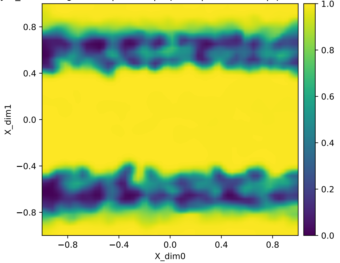
Inverse locality e_inv (Y-neigh -> X) | ribbon | repeats | Y=radial1d | q=65 heatmap (fixed [0,1])
