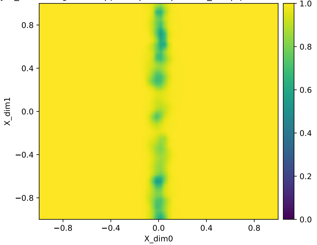
Inverse locality e_inv (Y-neigh -> X) | pinch | fixed | Y=raw_flat | q=16384 heatmap (fixed [0,1])
