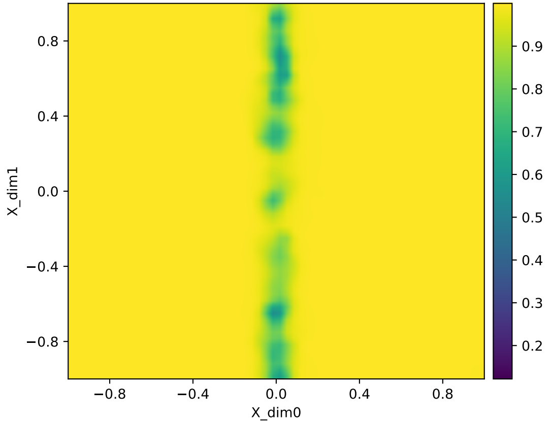
Inverse locality e_inv (Y-neigh -> X) | pinch | fixed | Y=raw_flat | q=16384 heatmap (adaptive)
