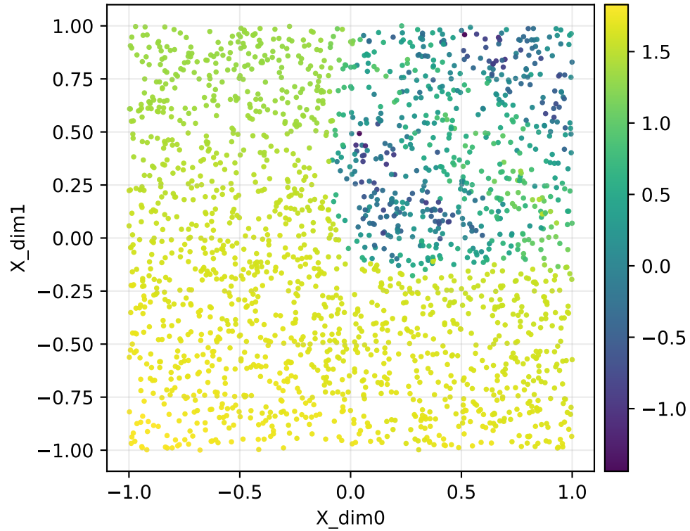
Forward map log10 singular value log10(smin(J)) | fold | fixed | Y=raw_flat | q=16384 (adaptive)
