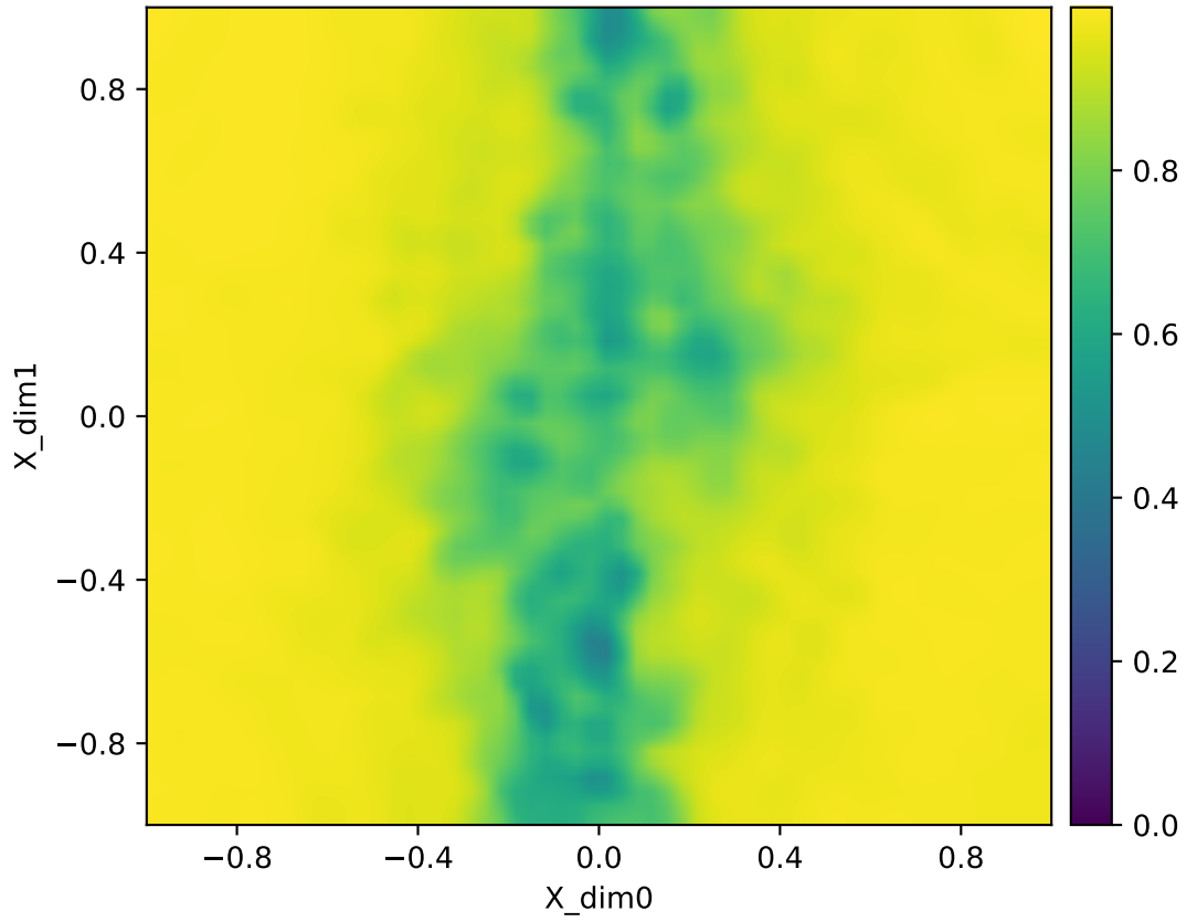
Inverse locality e_inv (Y-neigh -> X) | pinch | repeats | Y=corr2d | q=16385 heatmap (adaptive)
