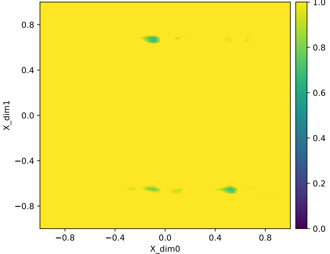
Forward map singular value smin(J) | ribbon | fixed | Y=raw_flat | q=16384 heatmap (fixed [0,1])
