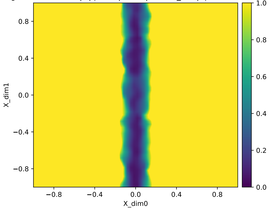
Forward map singular value smin(J) | pinch | fixed | Y=raw_flat | q=16384 heatmap (fixed [0,1])
