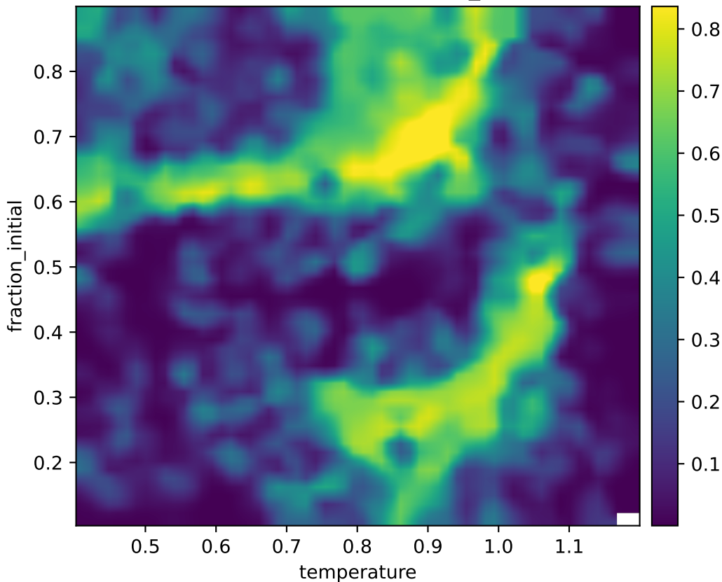
radial1d: heatmap explained_rankcap
