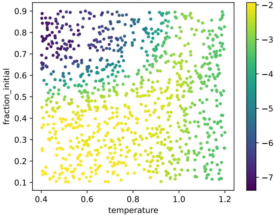
corr2d: log10 E_noise_raw (repeat-based)
