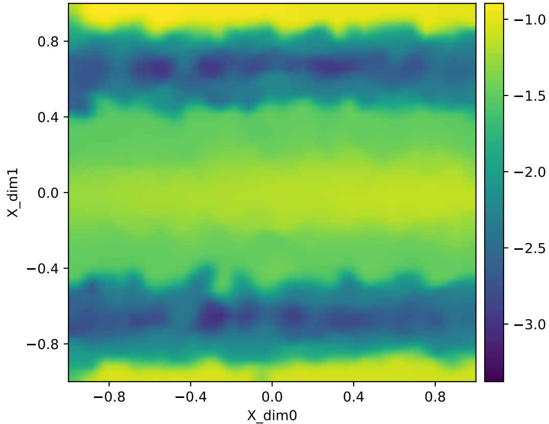
Forward map log10 singular value log10(smin(J)) | ribbon | repeats | Y=radial1d | q=65 heatmap (adaptive)
