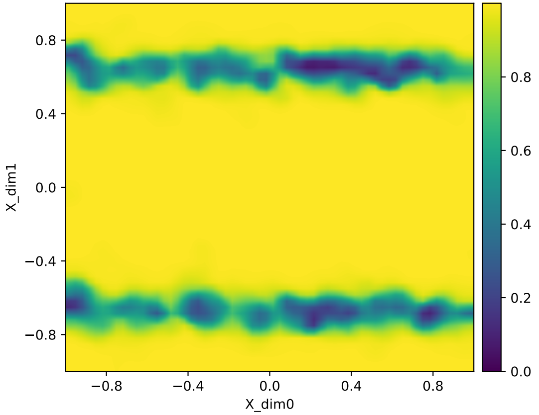
Inverse locality e_inv (Y-neigh -> X) | ribbon | fixed | Y=raw_flat | q=16384 heatmap (adaptive)
