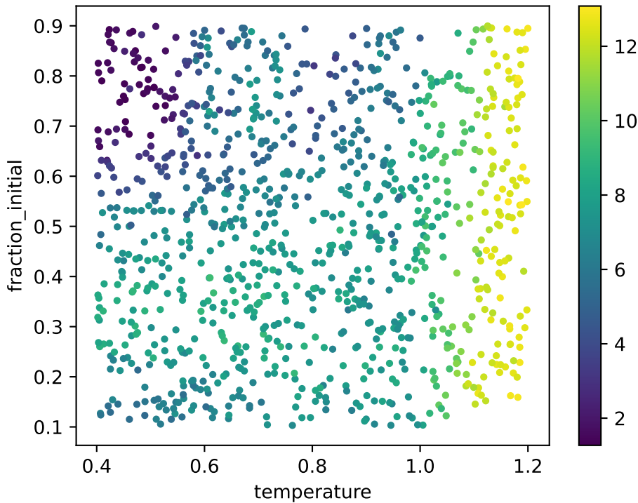
radial1d: effective rank (entropy) of local K
