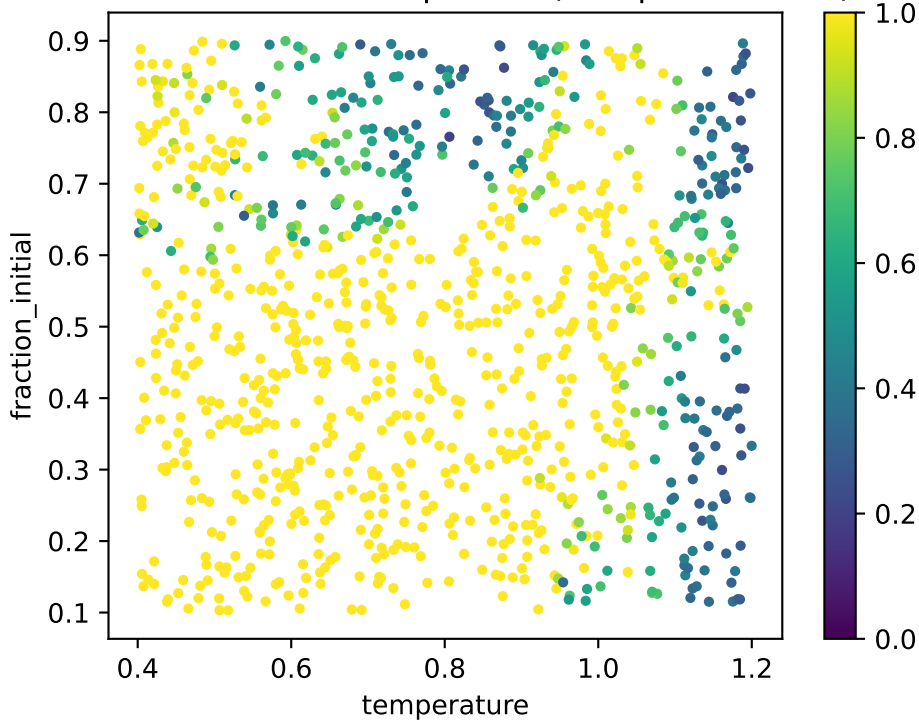
corr2d: max coord unexplained (collapse detector)
