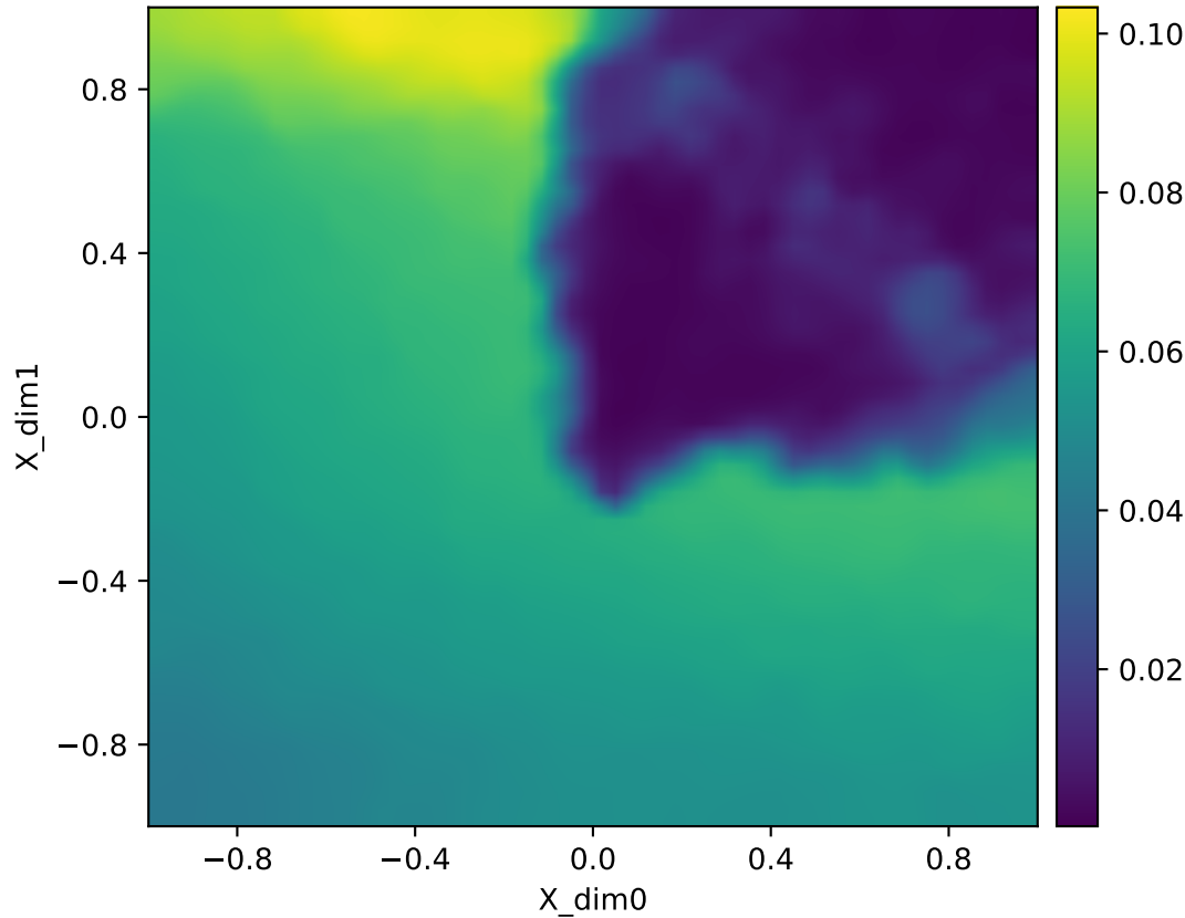
Forward map singular value smin(J) | fold | repeats | Y=radial1d | q=65 heatmap (adaptive)
