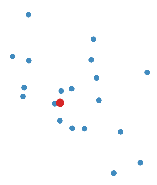
B) 1) X (standardized)
