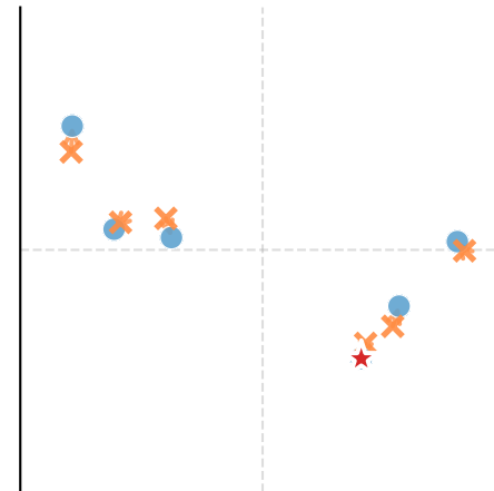
(4) LOO Score: 0.927
