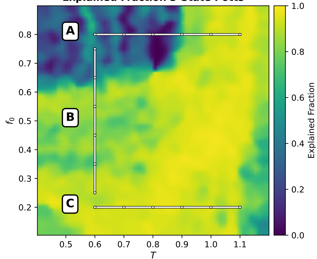
Explained Fraction 3-State Potts
