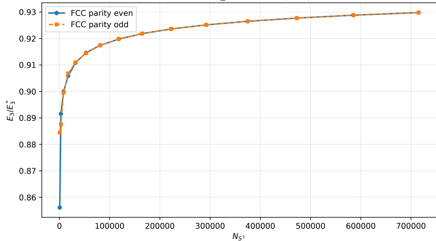
KR(O): E3 ratio vs N_S^3 for FCC parity choices
