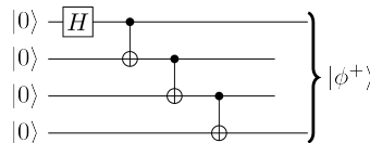
Figure 3: Length-3 EPR pair generation
