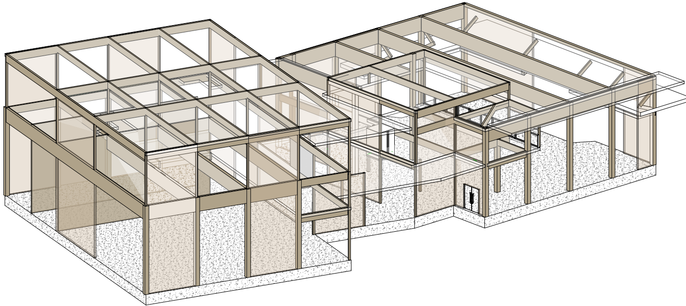
STRUCTURAL AXON 3/16''=1'
