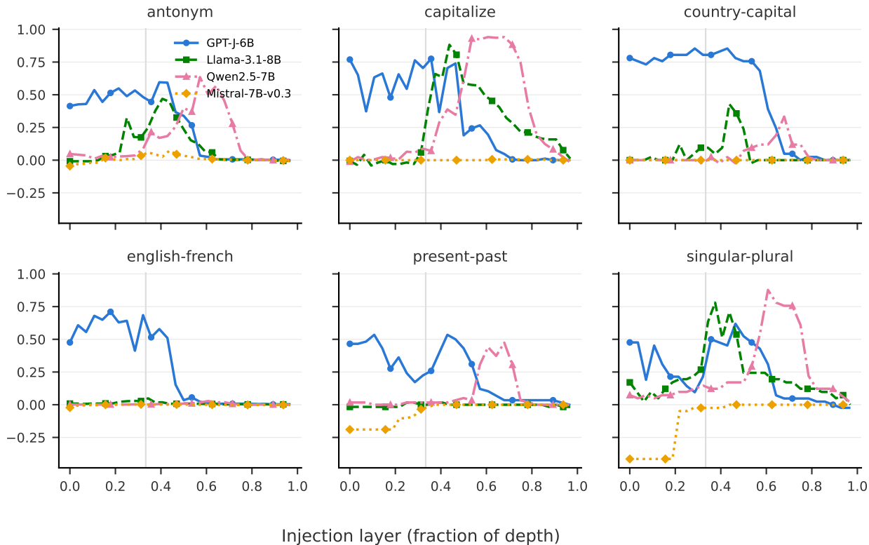
Zero-shot FV effect
