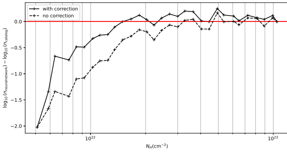
Fig. A.2: Differences in log space between the catalog core densities and the neural-network-predicted densities as a function of column density. The cloud is Orion B, neural network is UNet, and the dense-core catalog is from Könyves et al. (2020). The thick black line shows the density difference using the correction (Eq. A.4: L_d = 10 pc); the dotted black line shows the result without the correction. The red horizontal line indicates zero difference, i.e., where the neural-network prediction matches the catalog density.
