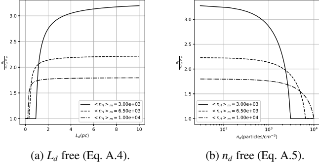
Fig. A.1: Correction \langle n_H \rangle_m \rightarrow n_c for different \langle n_H \rangle_m ; the vertical axis shows the ratio n_c / \langle n_H \rangle_m . The used parameters are r_c = 0.05 pc and N_H = 10^{22} cm ^{-2} .
