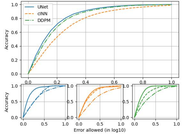
Fig. 9: Accuracy of the neural networks: UNet (blue), cINN (orange), and DDPM (green). Top panel: overall accuracy comparison between the networks. Bottom panels: accuracy curves for each network, binned by true mass-weighted average volume density (solid line: n_H \leq 200 cm ^{-3} ; dashed line: 200 cm ^{-3} < n_H \leq 10^4 cm ^{-3} ; dash-dotted line: n_H > 10^4 cm ^{-3} ).
