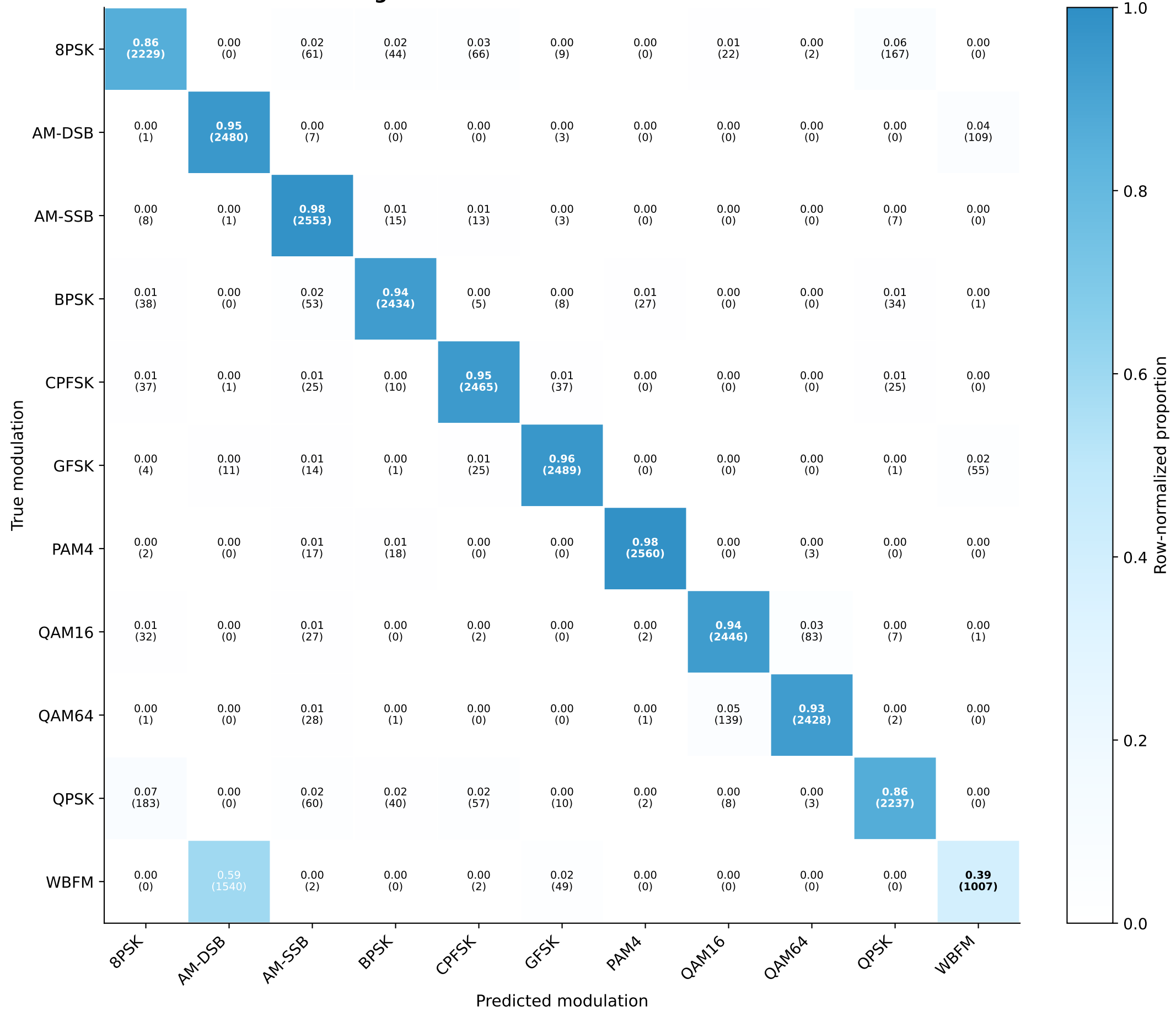
Figure 4. Normalized Confusion Matrix
