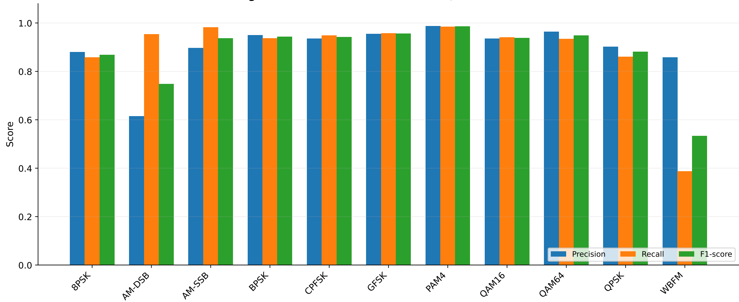
Figure 5. Per-Modulation Precision, Recall and F1
