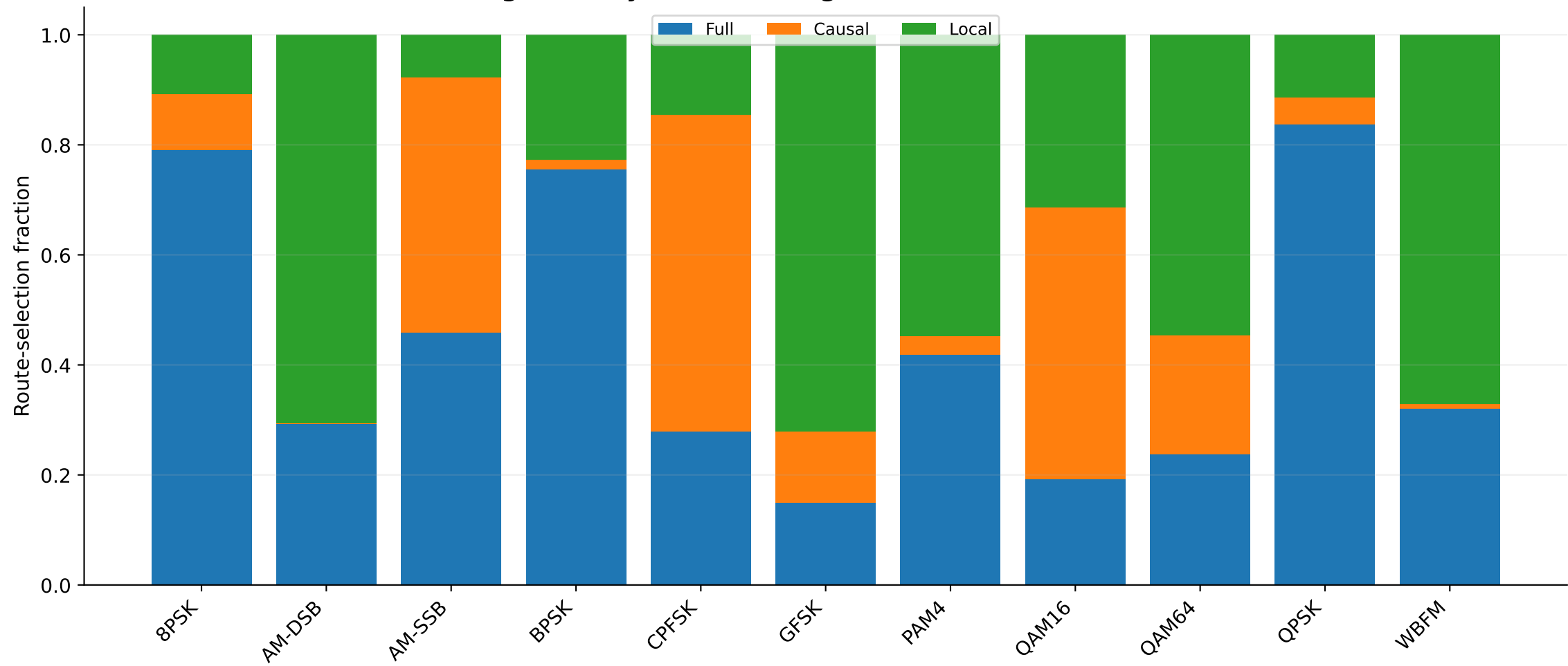
Figure 7. Dynamic Routing versus Modulation Class
