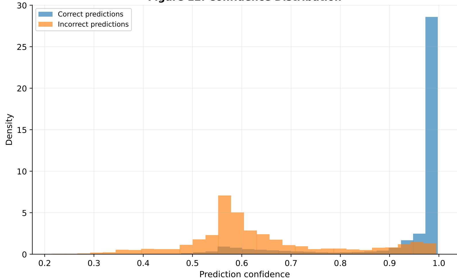
Figure 12. Confidence Distribution
