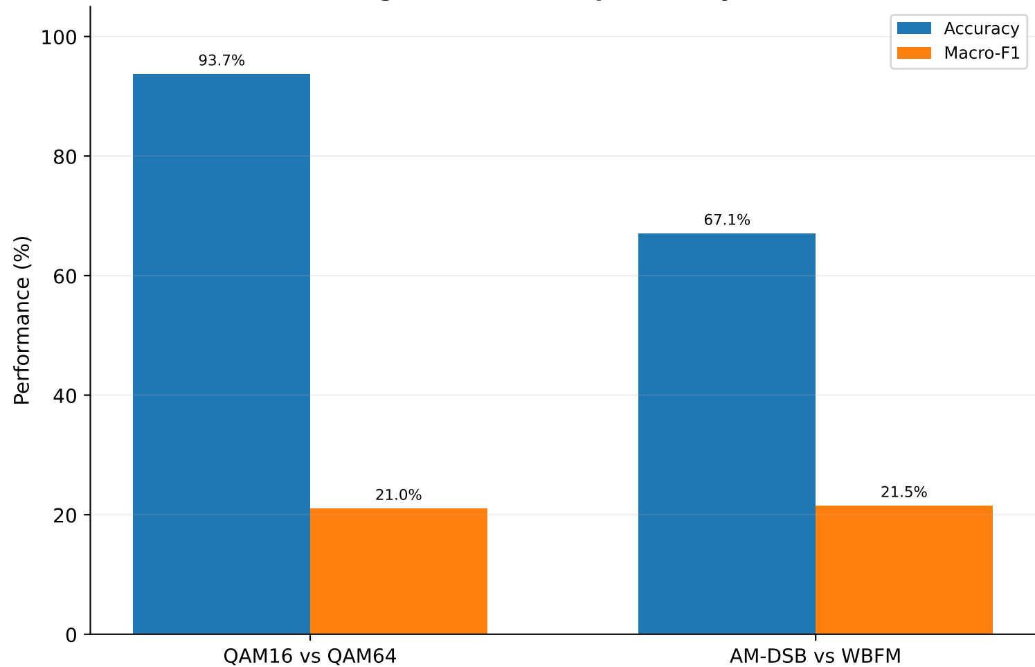
Figure 19. Pair-Expert Analysis
