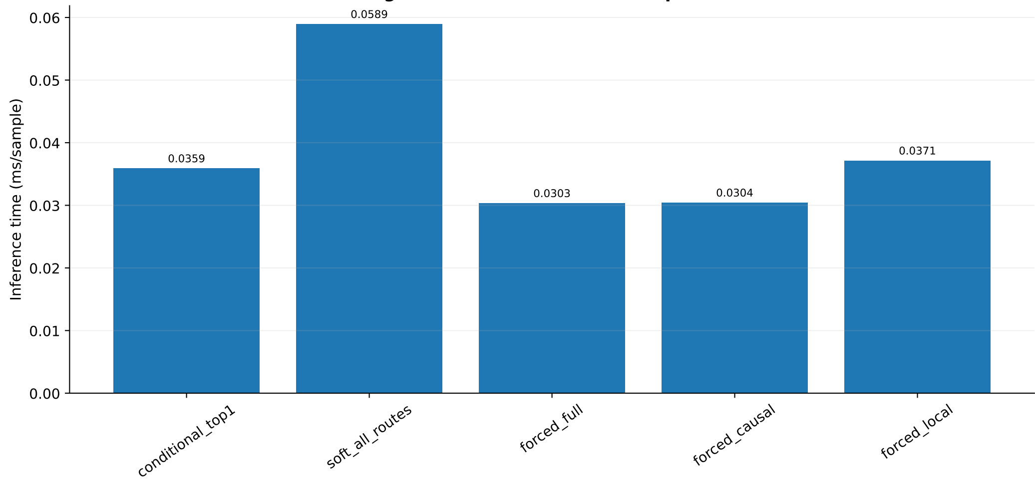
Figure 24. Inference-Time Comparison
