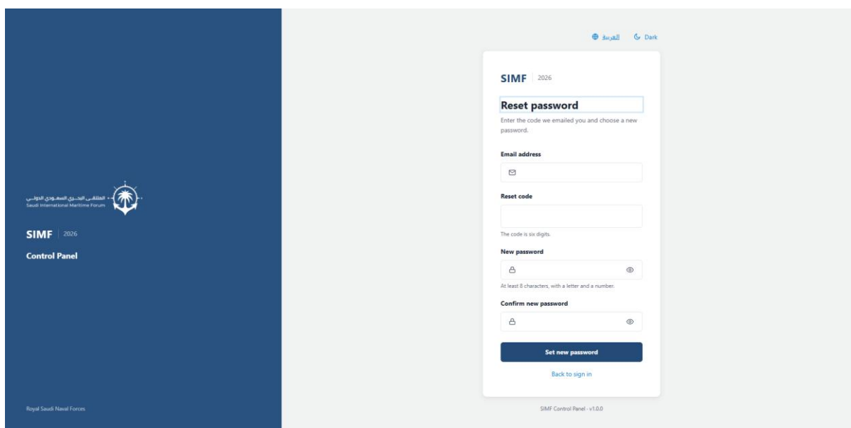
Figure 139 — /reset-password
