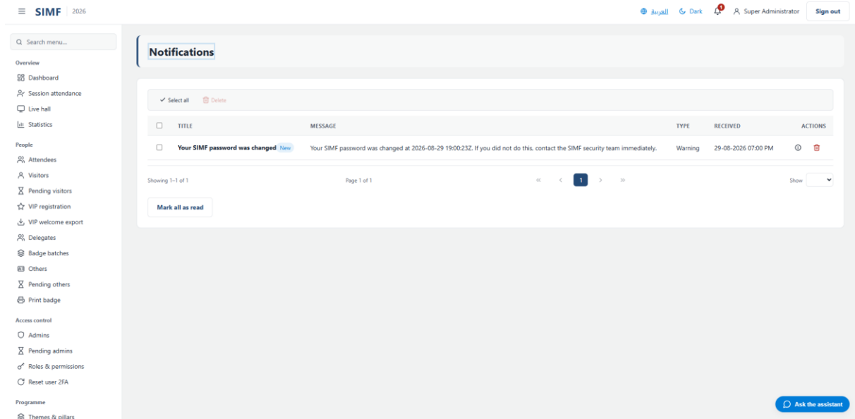
Figure 126 — /account/notifications
