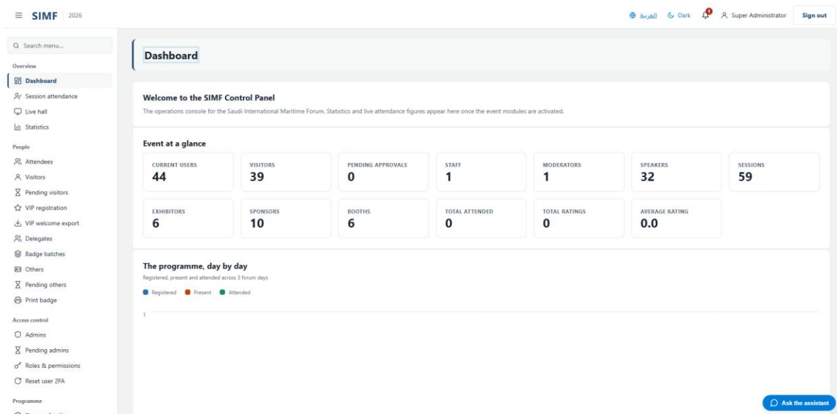
Figure 32 — Dashboard — /
