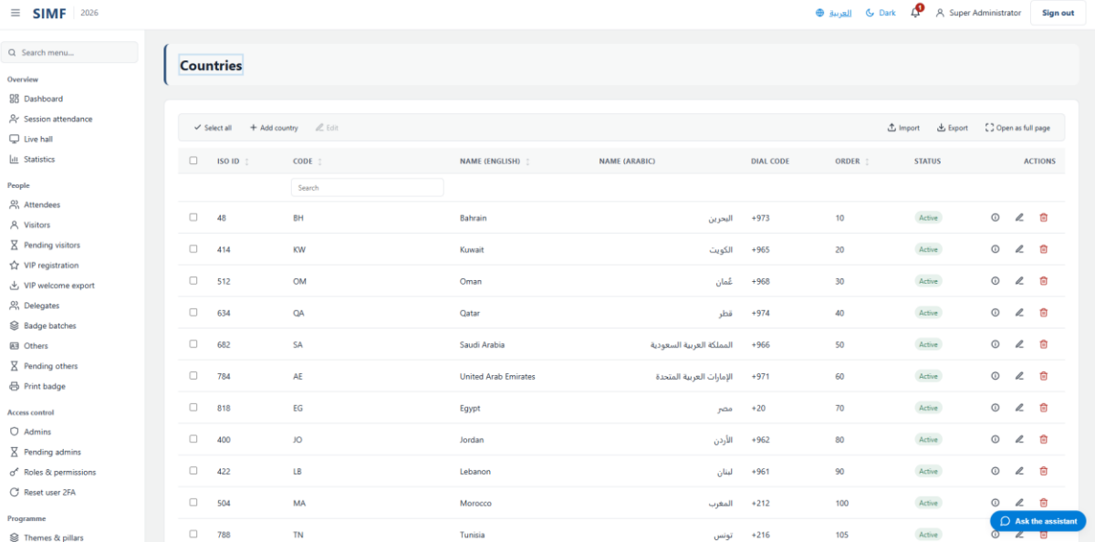
Figure 101 — Countries — /admin/countries
