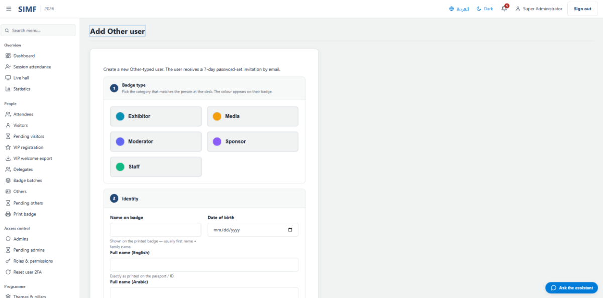
Figure 131 — /admin/others/new
