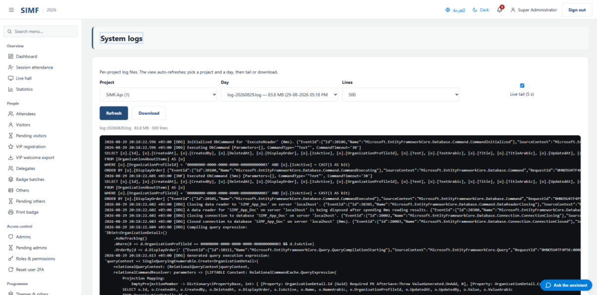
Figure 111 — Logs — /admin/logs
