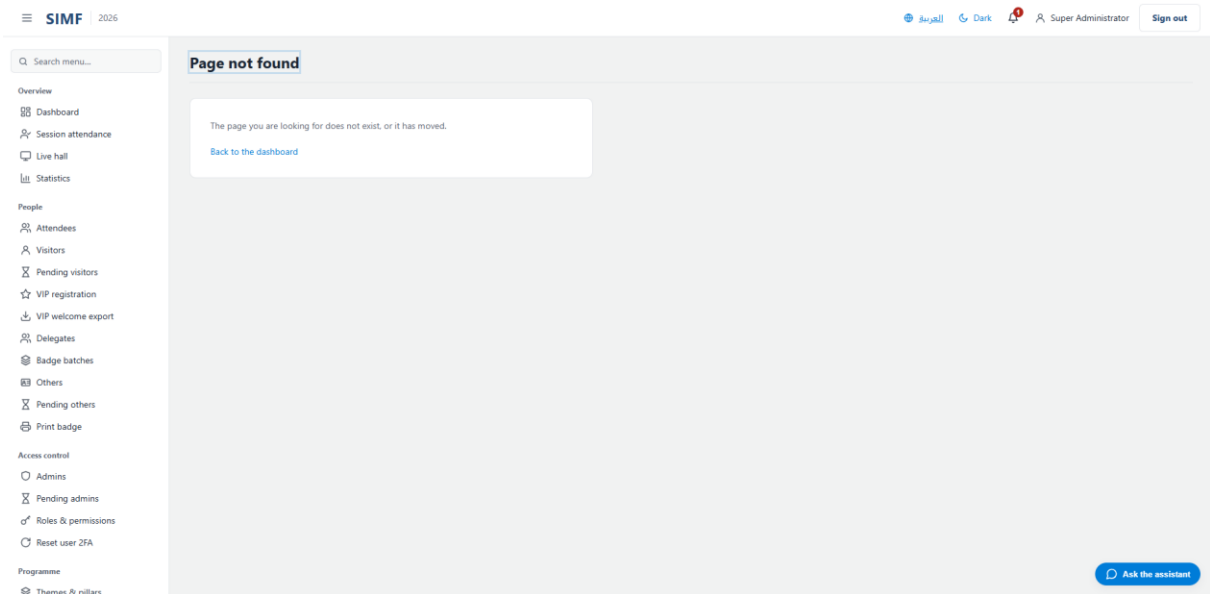
Figure 137 — /not-found
