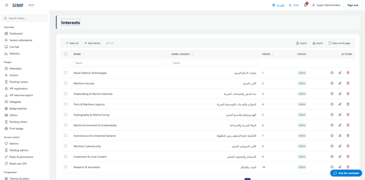
Figure 100 — Interests — /admin/interests
