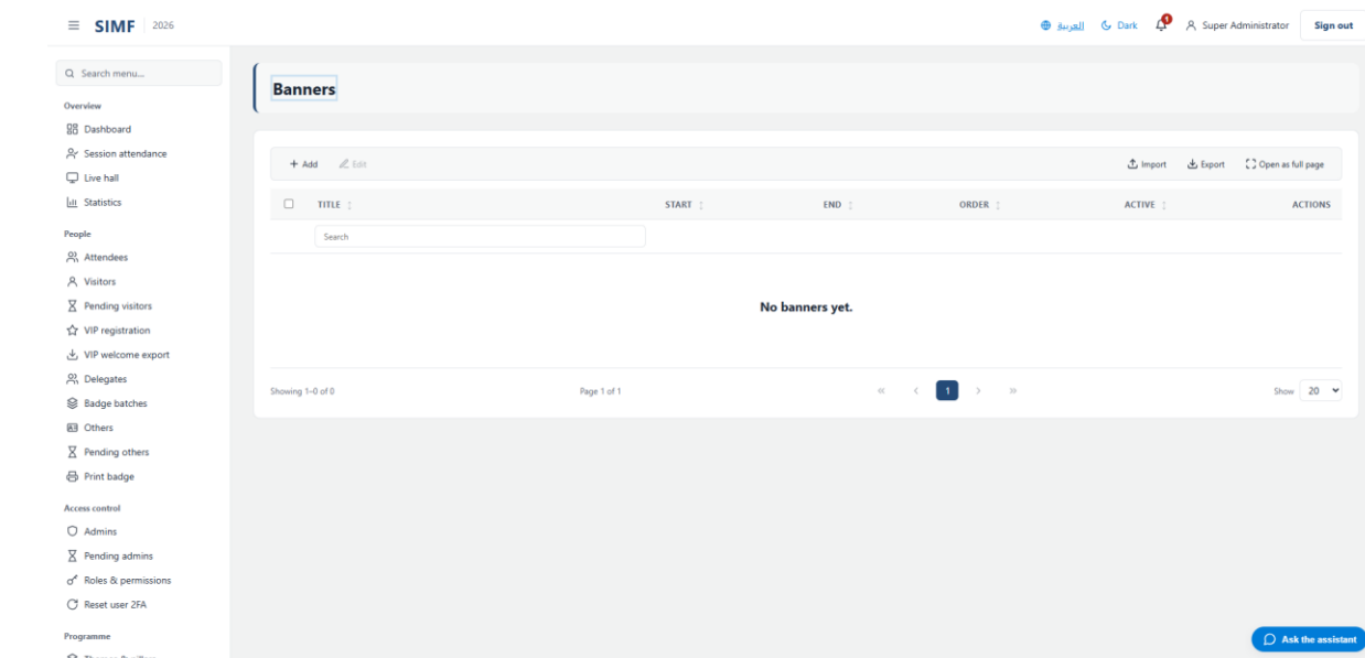
Figure 87 — Banners — /admin/banners
