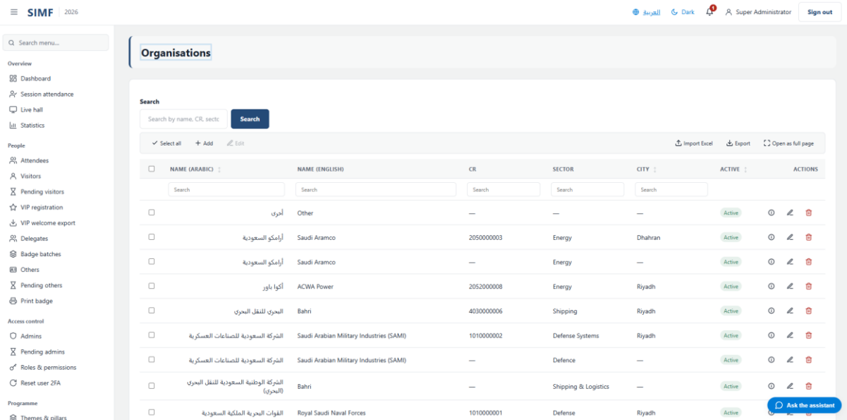
Figure 102 — Organisations — /admin/organisations
