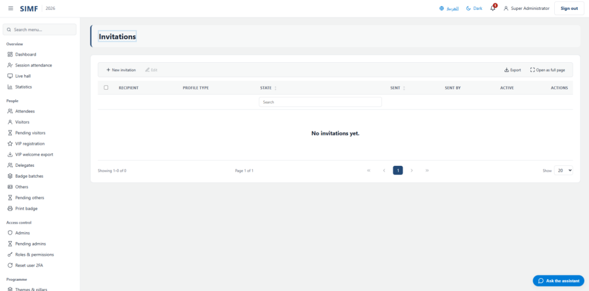
Figure 92 — Invitations — /admin/invitations
