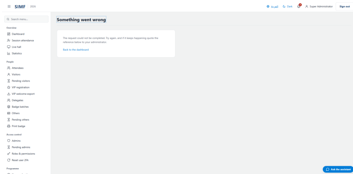
Figure 125 — /Error
