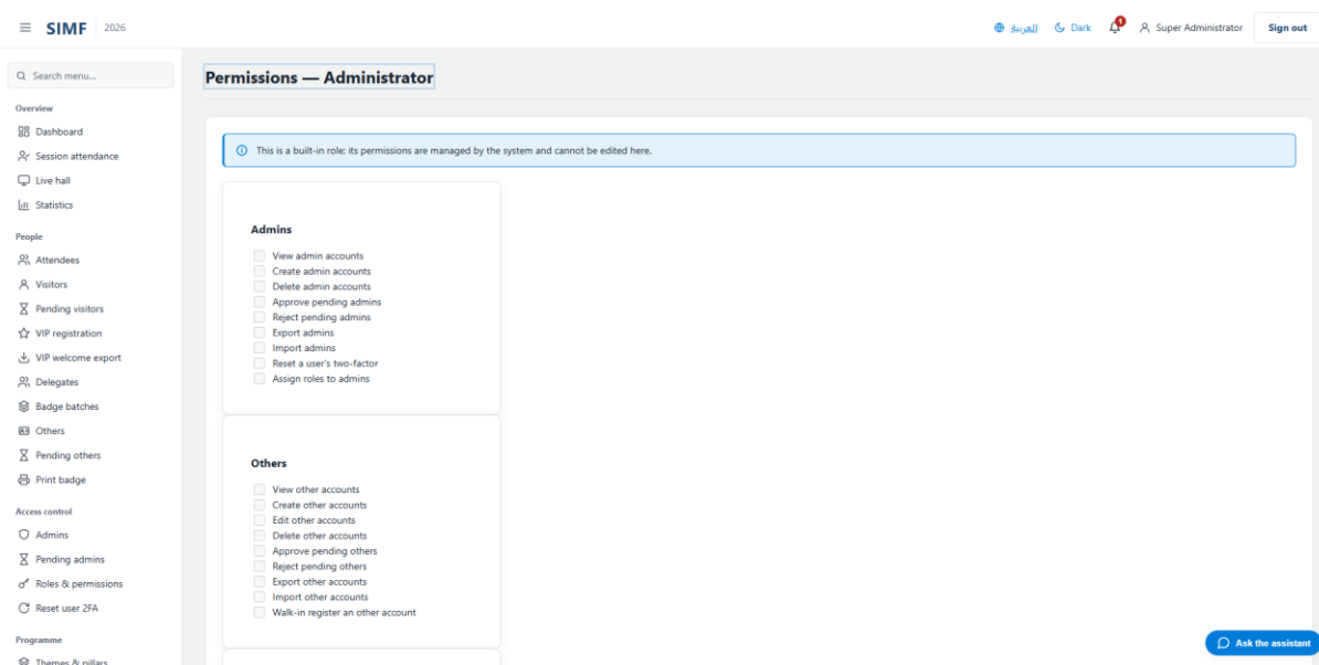
Figure 132 — /admin/roles/{RoleId:guid}/permissions
