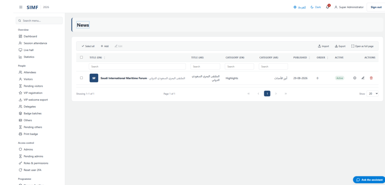
Figure 89 — News — /admin/news
