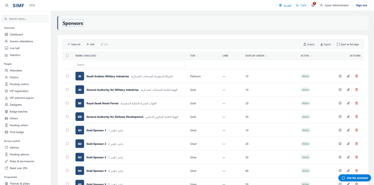
Figure 75 — Sponsors — /admin/sponsors
