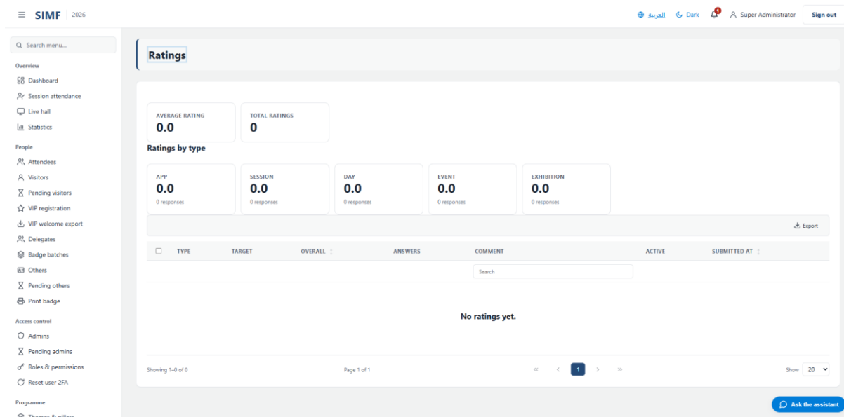
Figure 78 — Ratings — /admin/ratings
