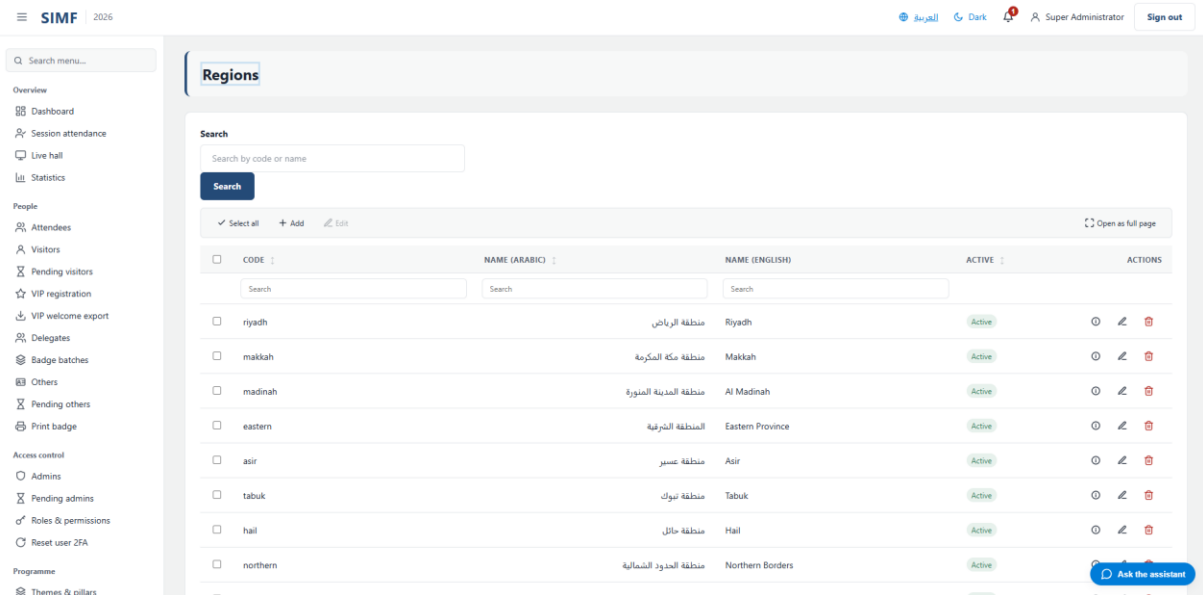
Figure 103 — Regions — /admin/regions
