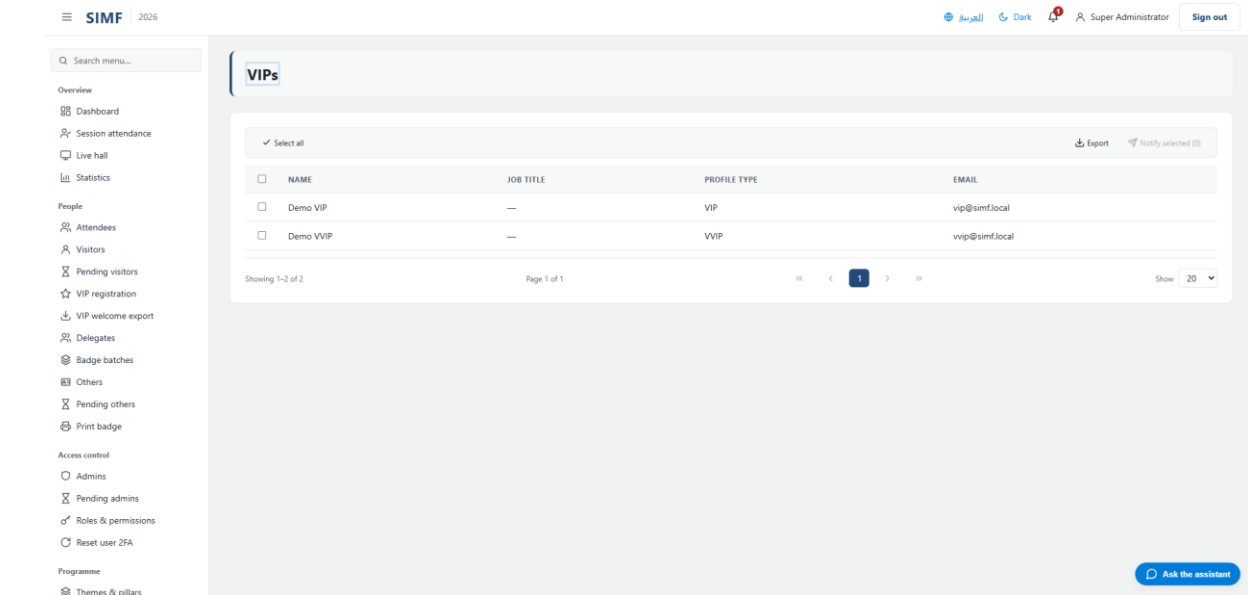
Figure 93 — VIPs — /admin/vips
