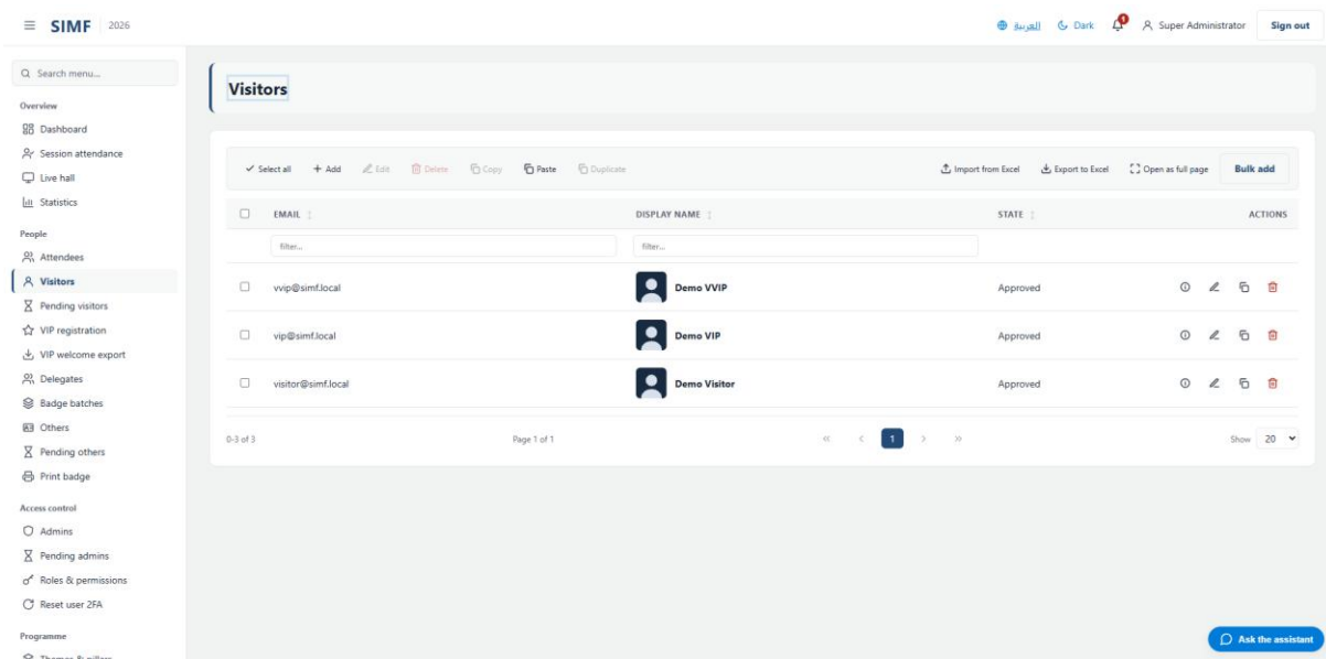
Figure 37 — Visitors — /admin/visitors
