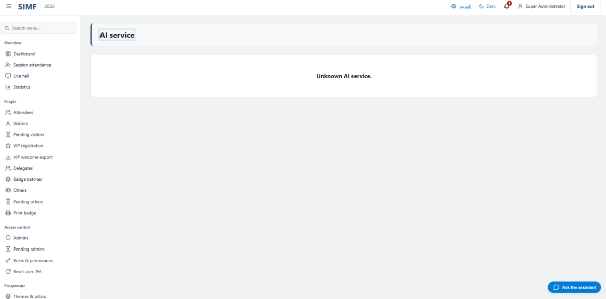
Figure 130 — /admin/ai/services/{Feature}
