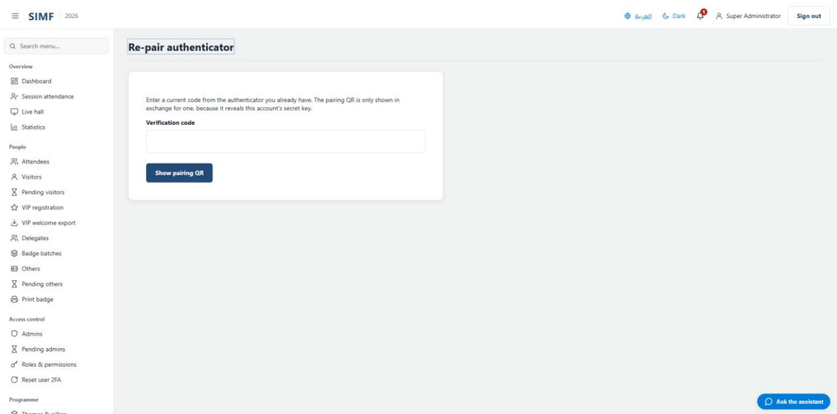
Figure 128 — /account/totp-pairing
