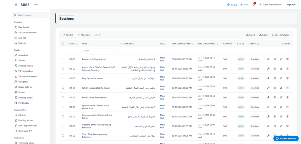
Figure 51 — Sessions — /admin/sessions
