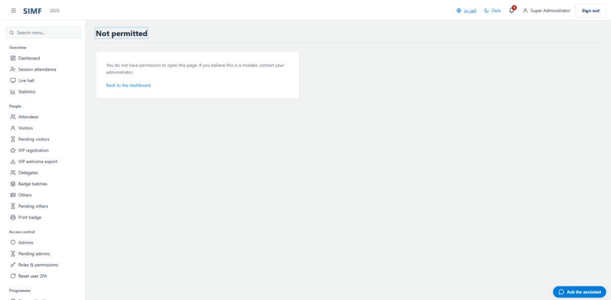
Figure 138 — /not-permitted
