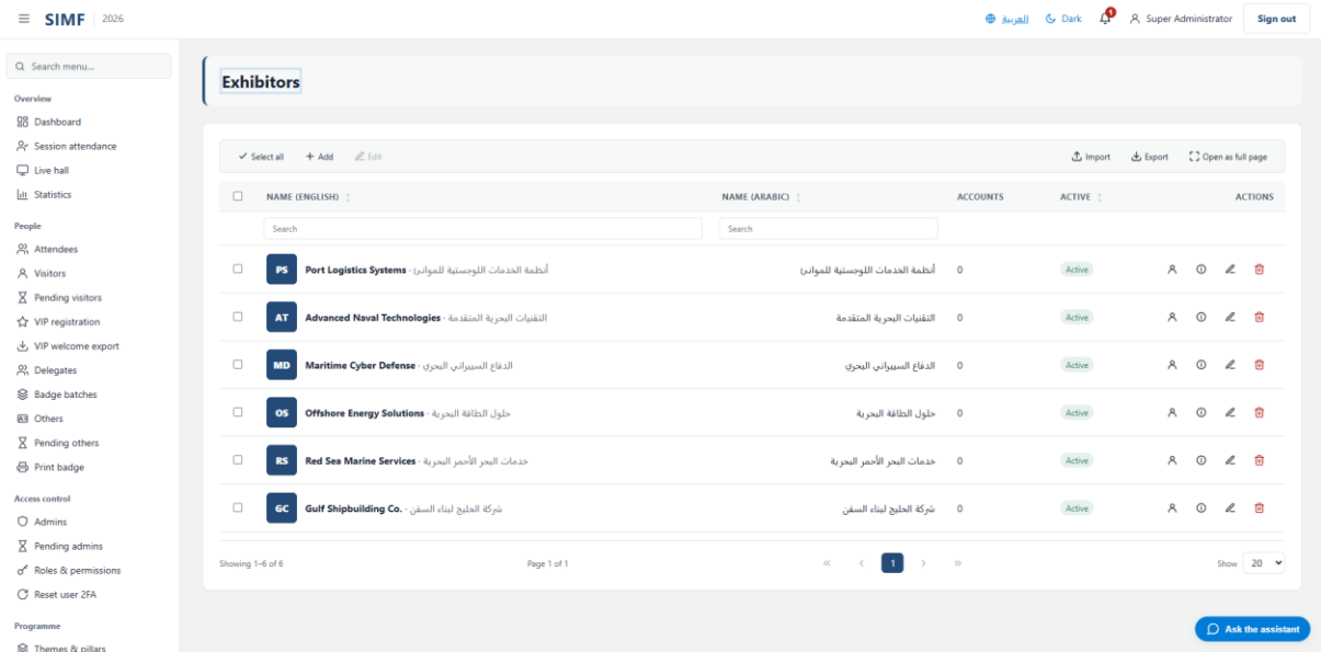
Figure 73 — Exhibitors — /admin/exhibitors
