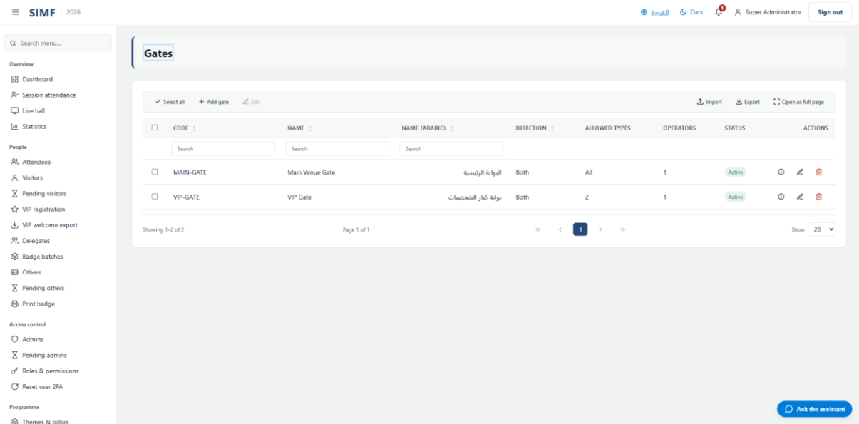
Figure 96 — Gates — /admin/gates
