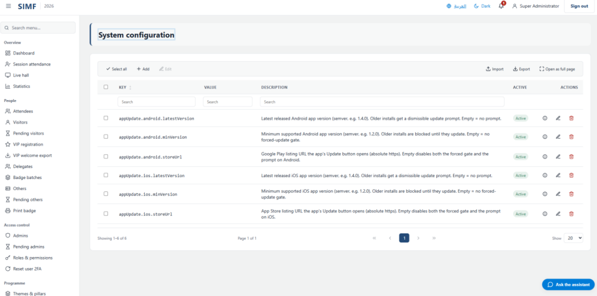
Figure 106 — Configuration — /admin/configuration
