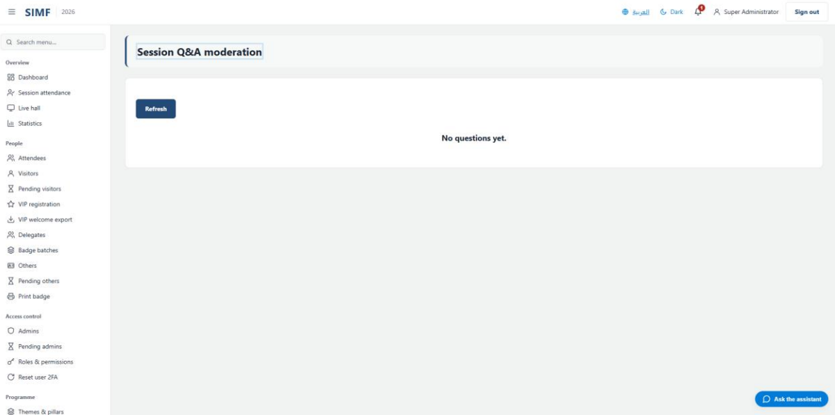
Figure 140 — /sessions/{SessionId:guid}/moderate
