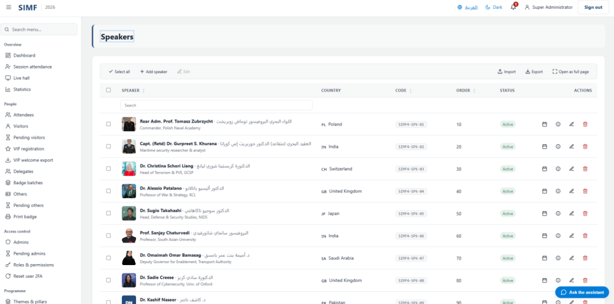
Figure 65 — Speakers — /admin/speakers
