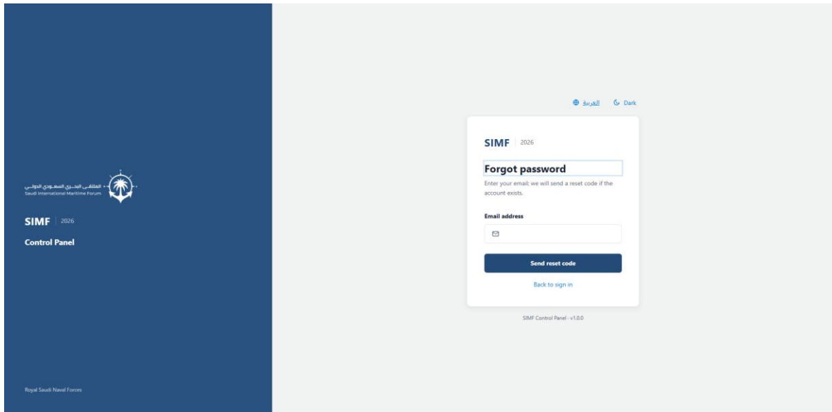
Figure 134 — /forgot-password
