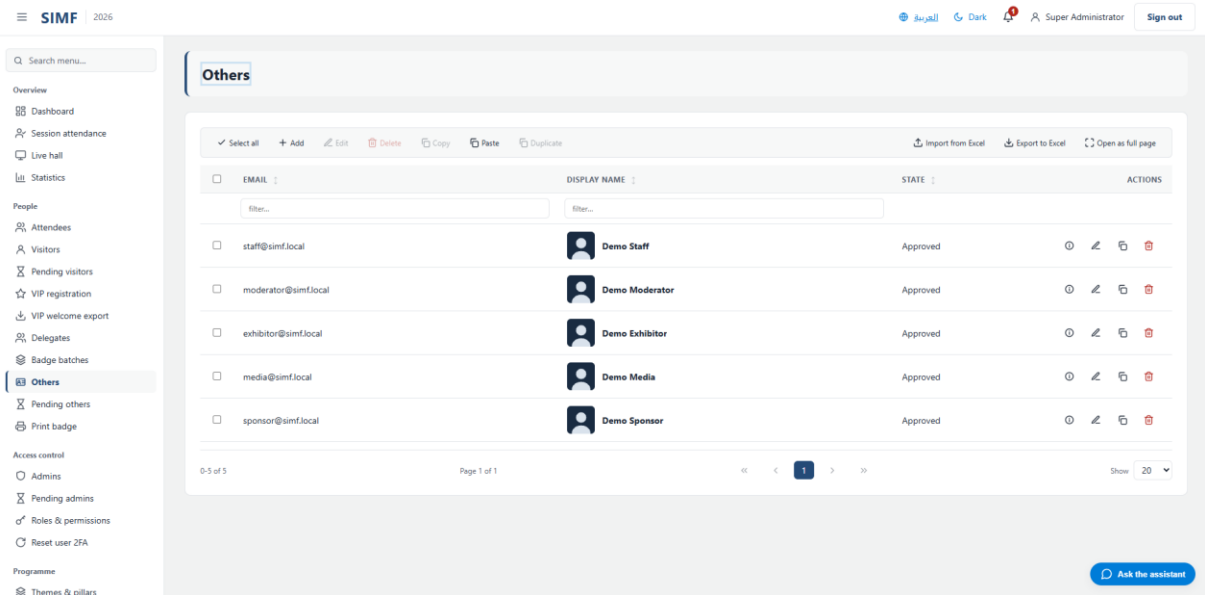
Figure 43 — Others — /admin/others
