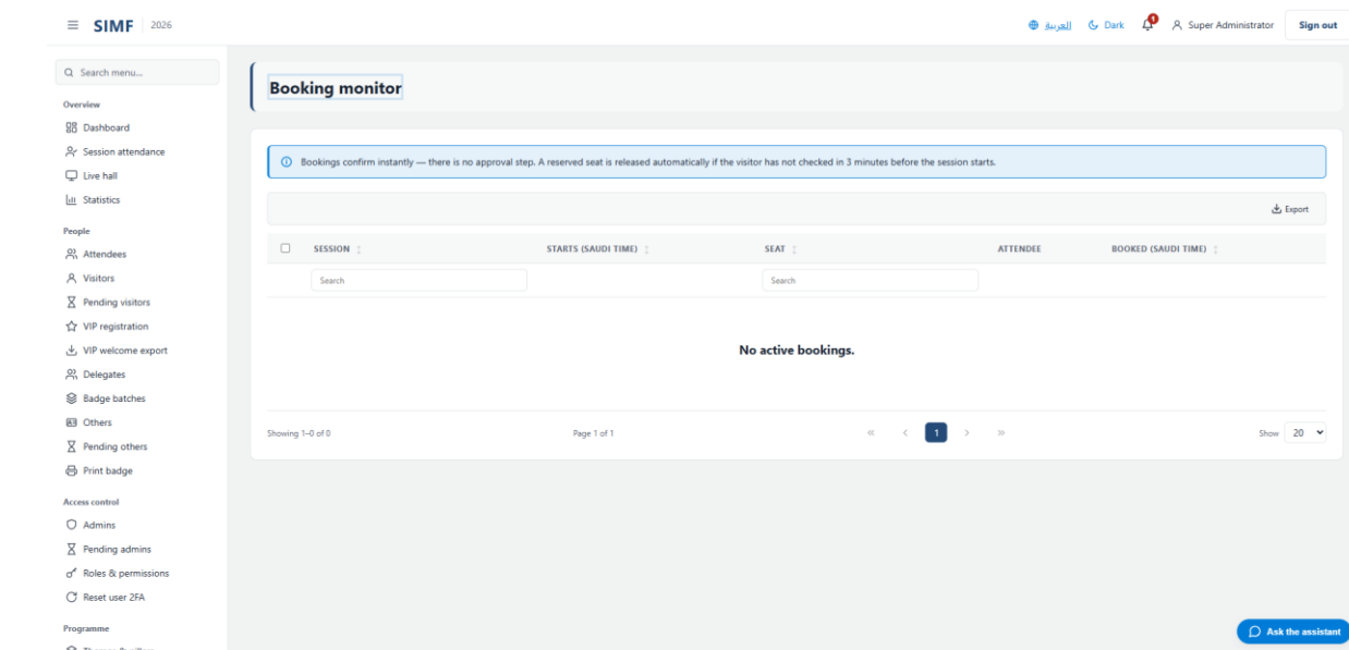
Figure 67 — Bookings — /admin/bookings
