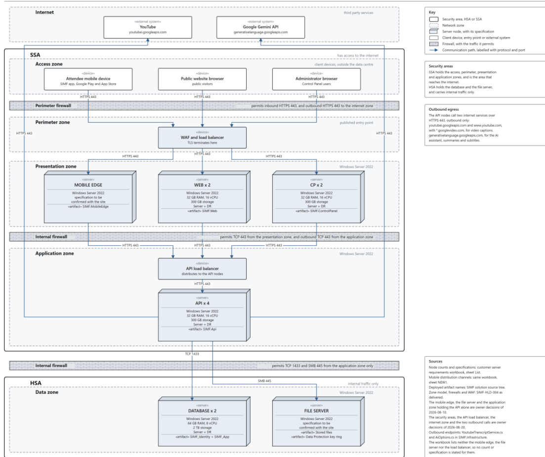
Figure 3. SIMF target deployment, security areas and internet egress. A UML deployment diagram: one node per hosting server, with its zone, its specification from the customer server requirements workbook, and the protocol and port of every path. The zones are grouped into two security areas, and the API's two outbound calls to the internet are shown crossing both firewalls.
