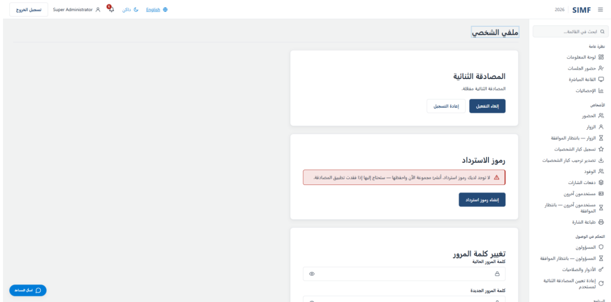
شكل 134 — /account/profile
