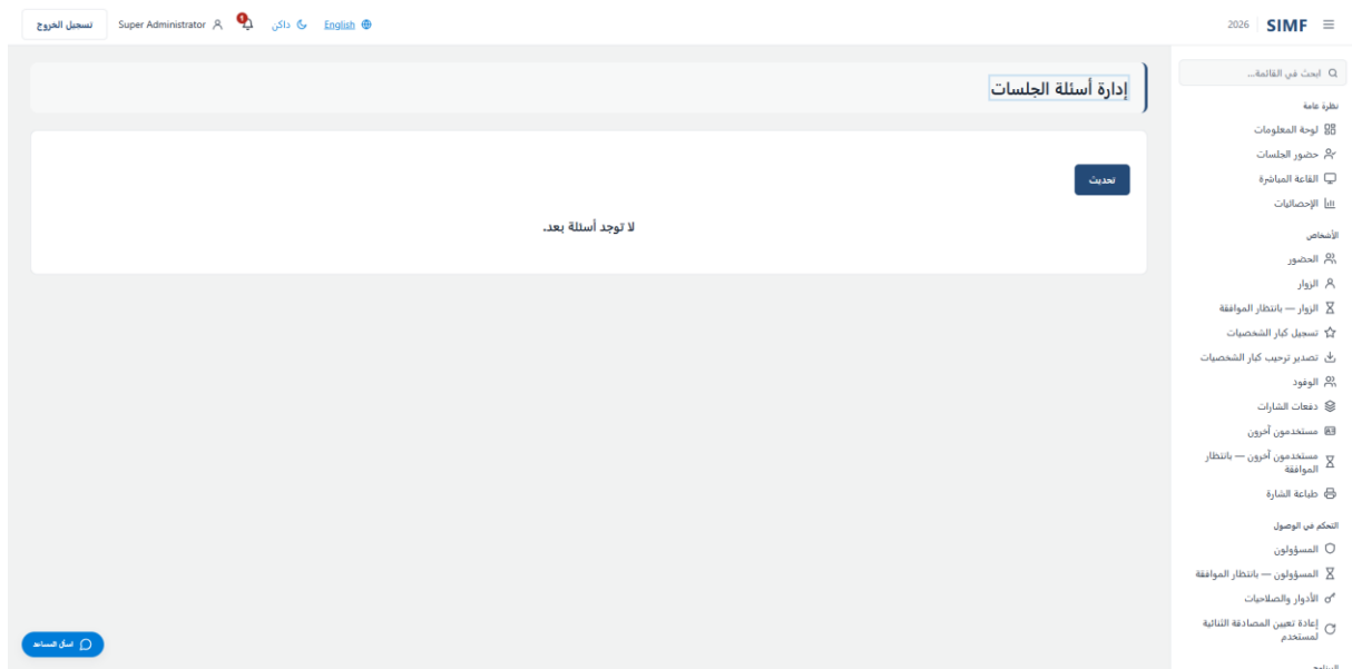
شكل 147 — /sessions/{SessionId:guid}/moderate
