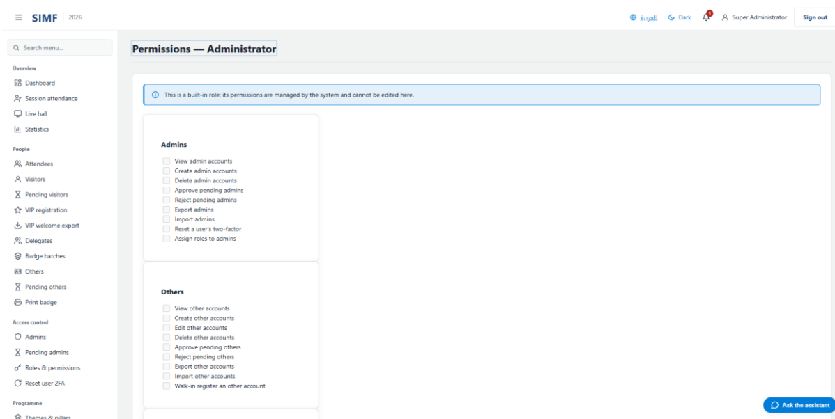
Figure 139 — /admin/roles/{RoleId:guid}/permissions
