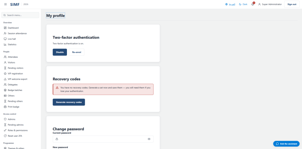
Figure 134 — /account/profile
