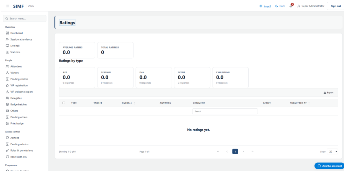
Figure 85 — Ratings — /admin/ratings
