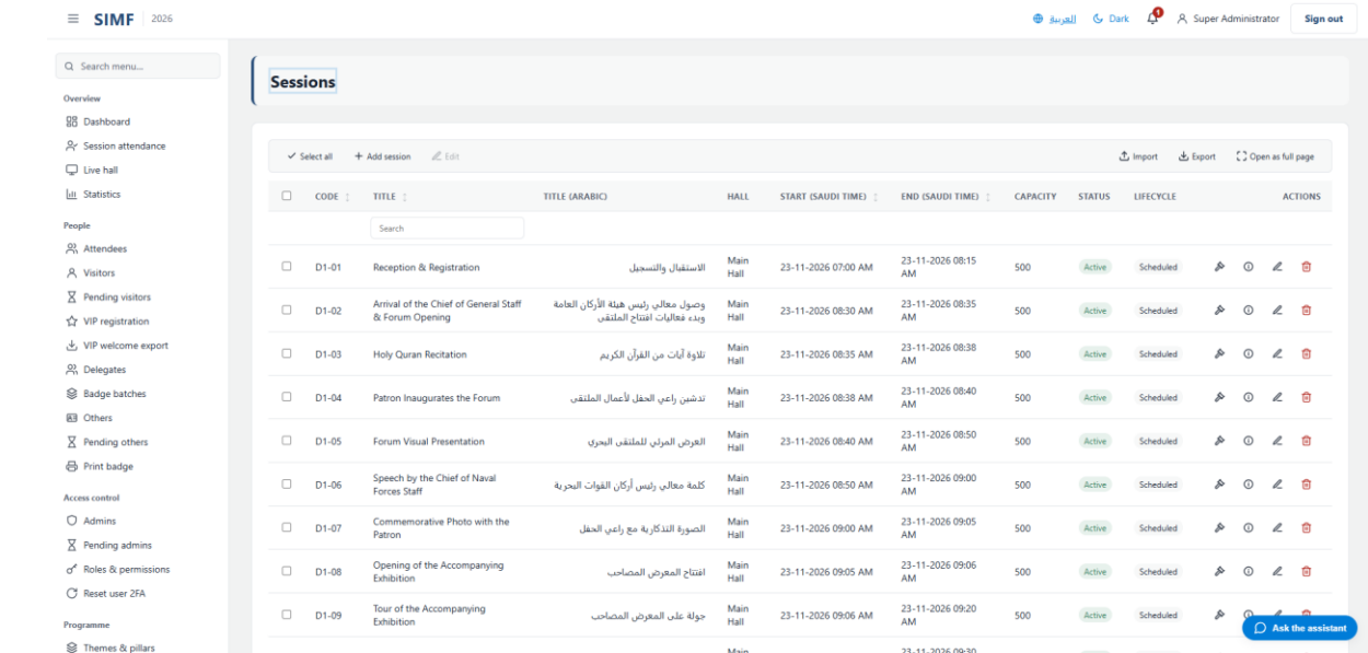
Figure 58 — Sessions — /admin/sessions
