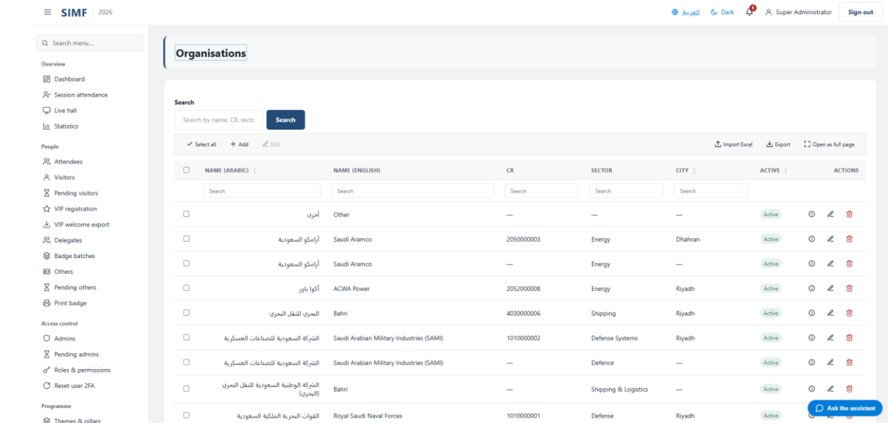
Figure 109 — Organisations — /admin/organisations
