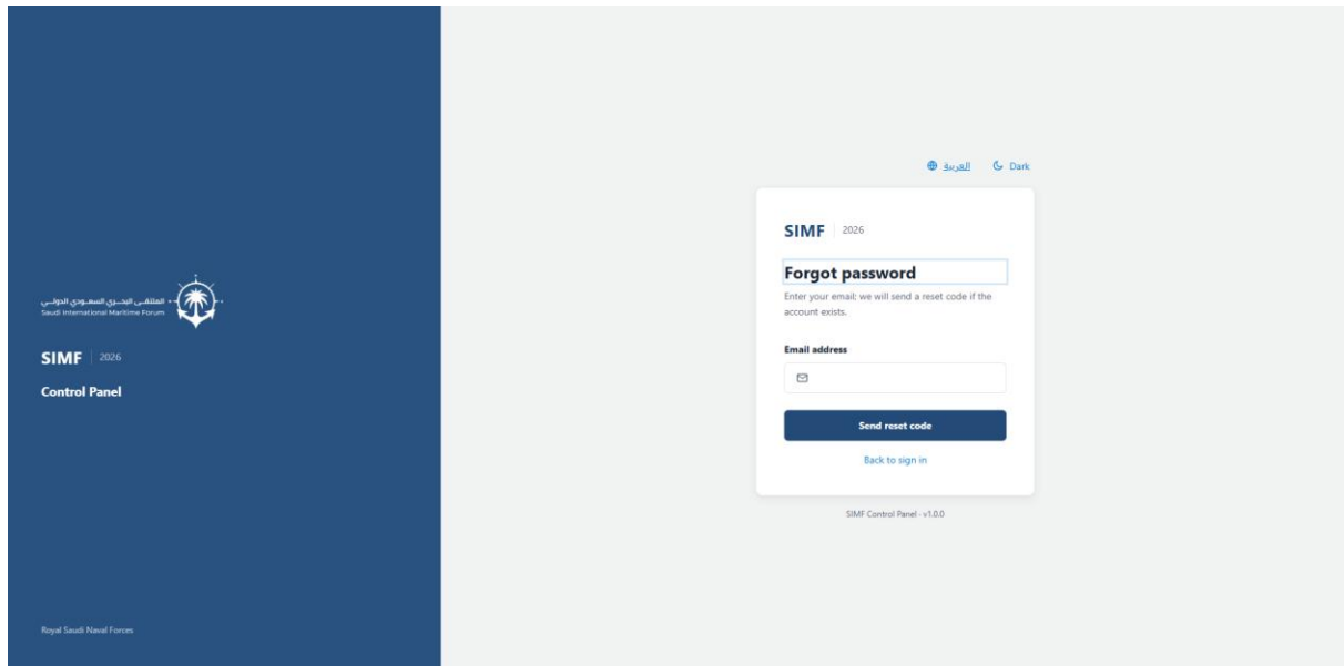
Figure 141 — /forgot-password
