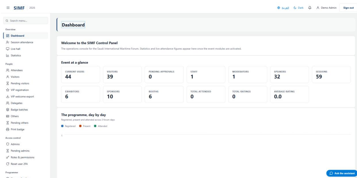
Figure 39 — Dashboard — /
