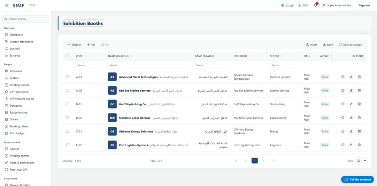
Figure 81 — Booths — /admin/booths
