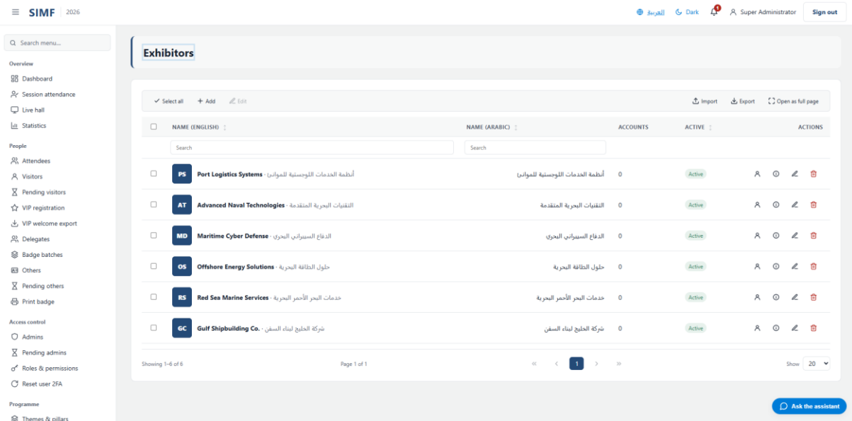
Figure 80 — Exhibitors — /admin/exhibitors
