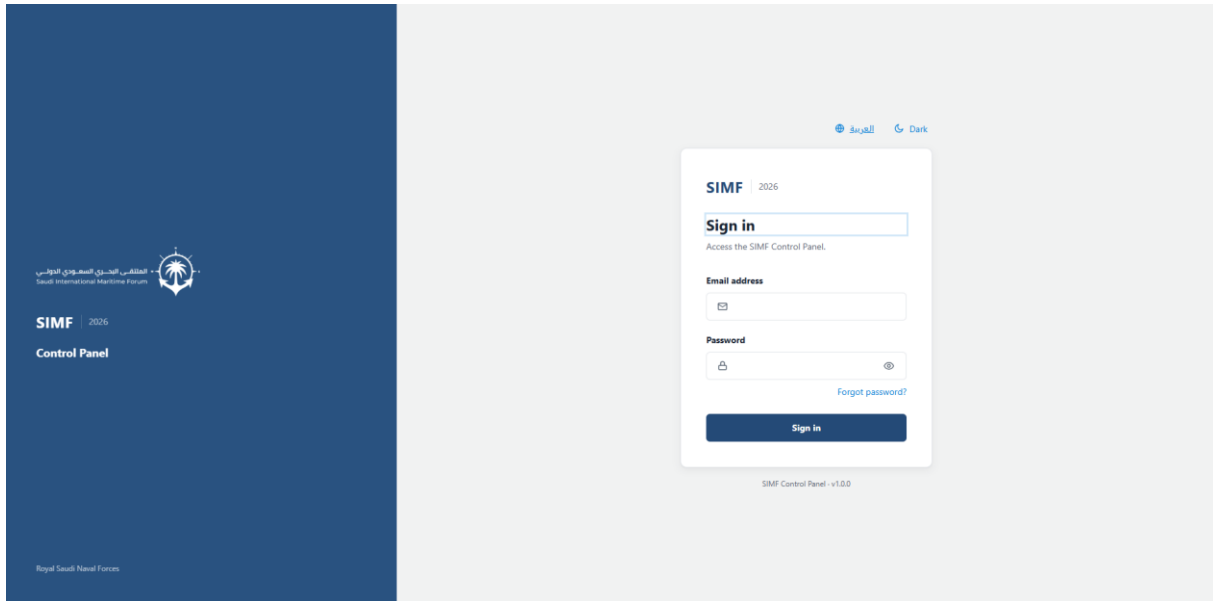
Figure 142 — /login
