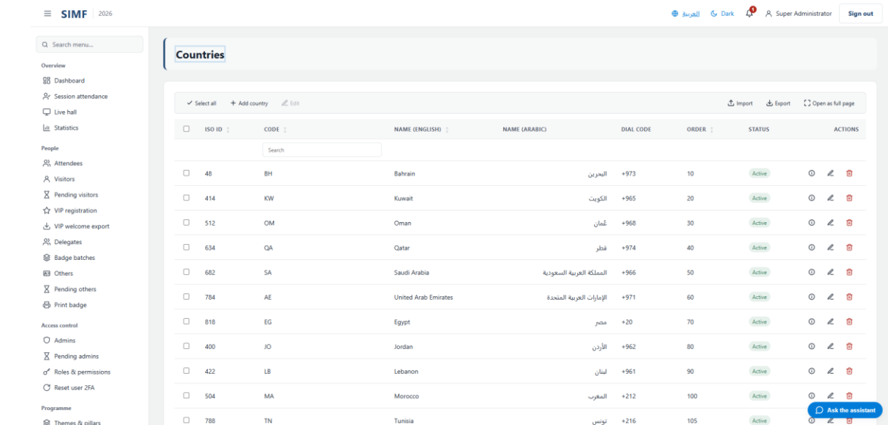
Figure 108 — Countries — /admin/countries
