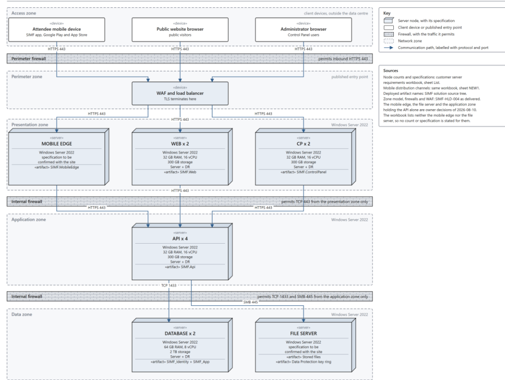
Figure 2. SIMF target three-tier deployment, agreed on 10 August 2026. A UML deployment diagram: the presentation zone holds the web, Control Panel and mobile-edge hosts, and the application zone holds the API alone, reachable only from the presentation zone.
