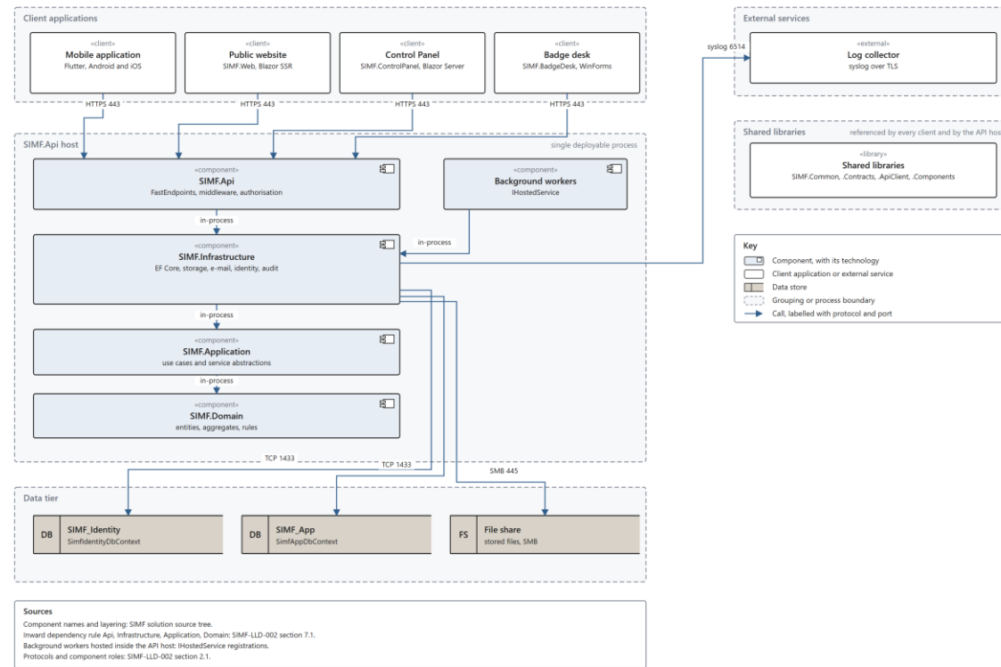
Figure 3. SIMF system components and their interaction. A UML component diagram: every component with its technology, and every call labelled with its protocol and port.
