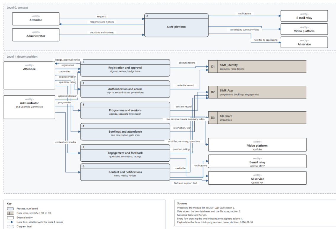
Figure 4. SIMF system and data flow. A data flow diagram in Gane and Sarson notation: a level 0 context view and a level 1 decomposition that balances with it.
