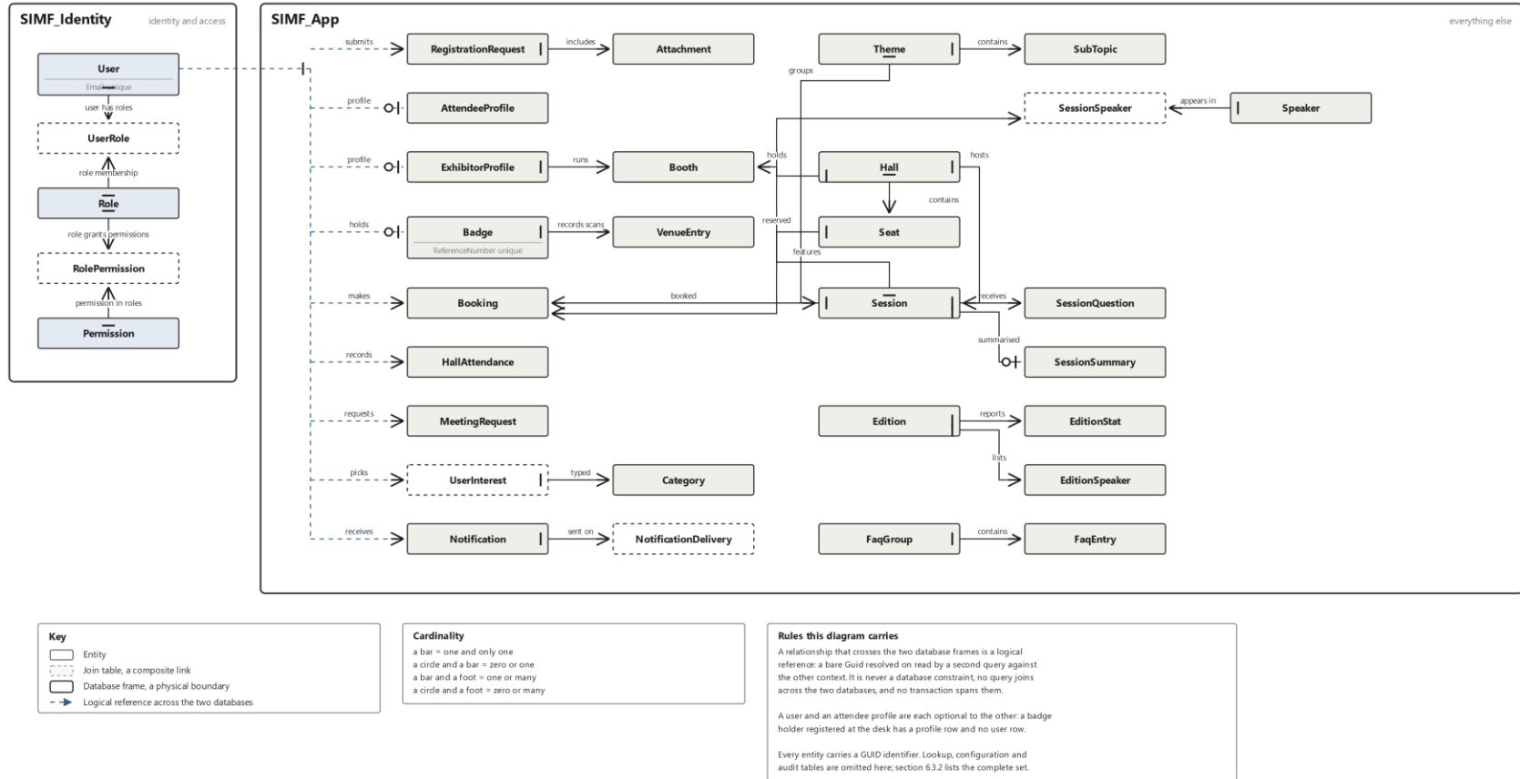
Figure 2. The core entity relationship diagram, in crow's foot notation. The two database frames are physically separate, so a relationship that crosses a frame is a logical reference held in application code and never a foreign key.
