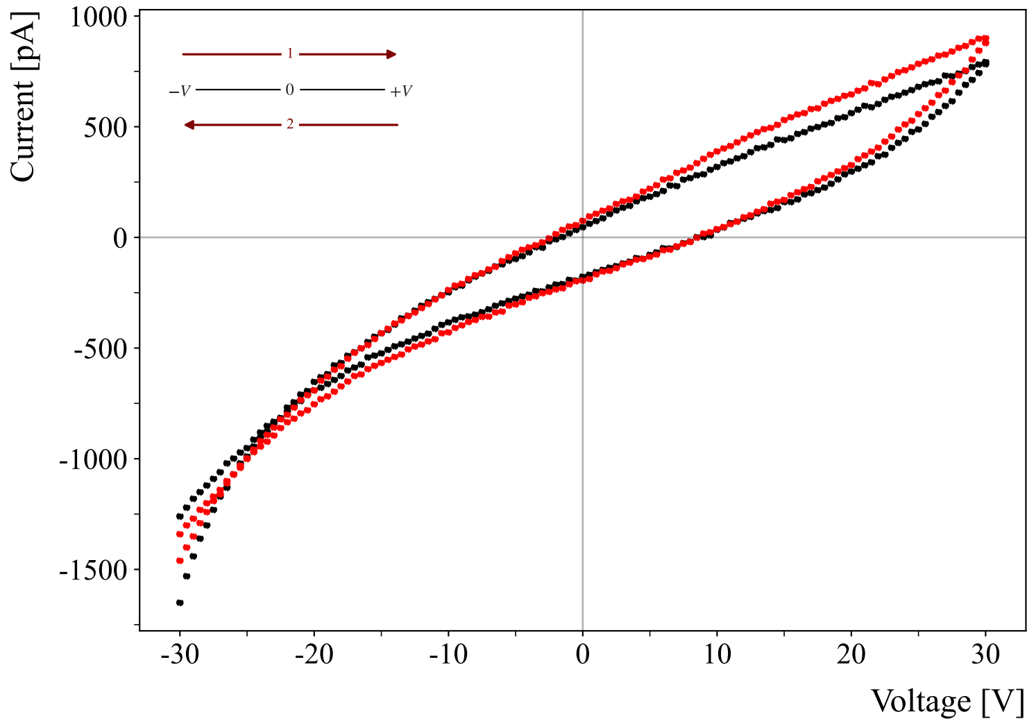
DG-PCB001_IV_7.5mm_both
