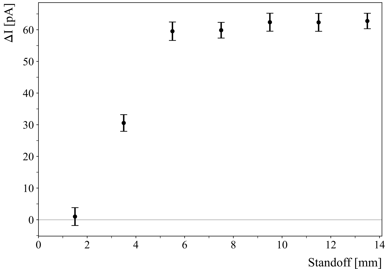
DG-PCB001_dynamics_standoff_30V
