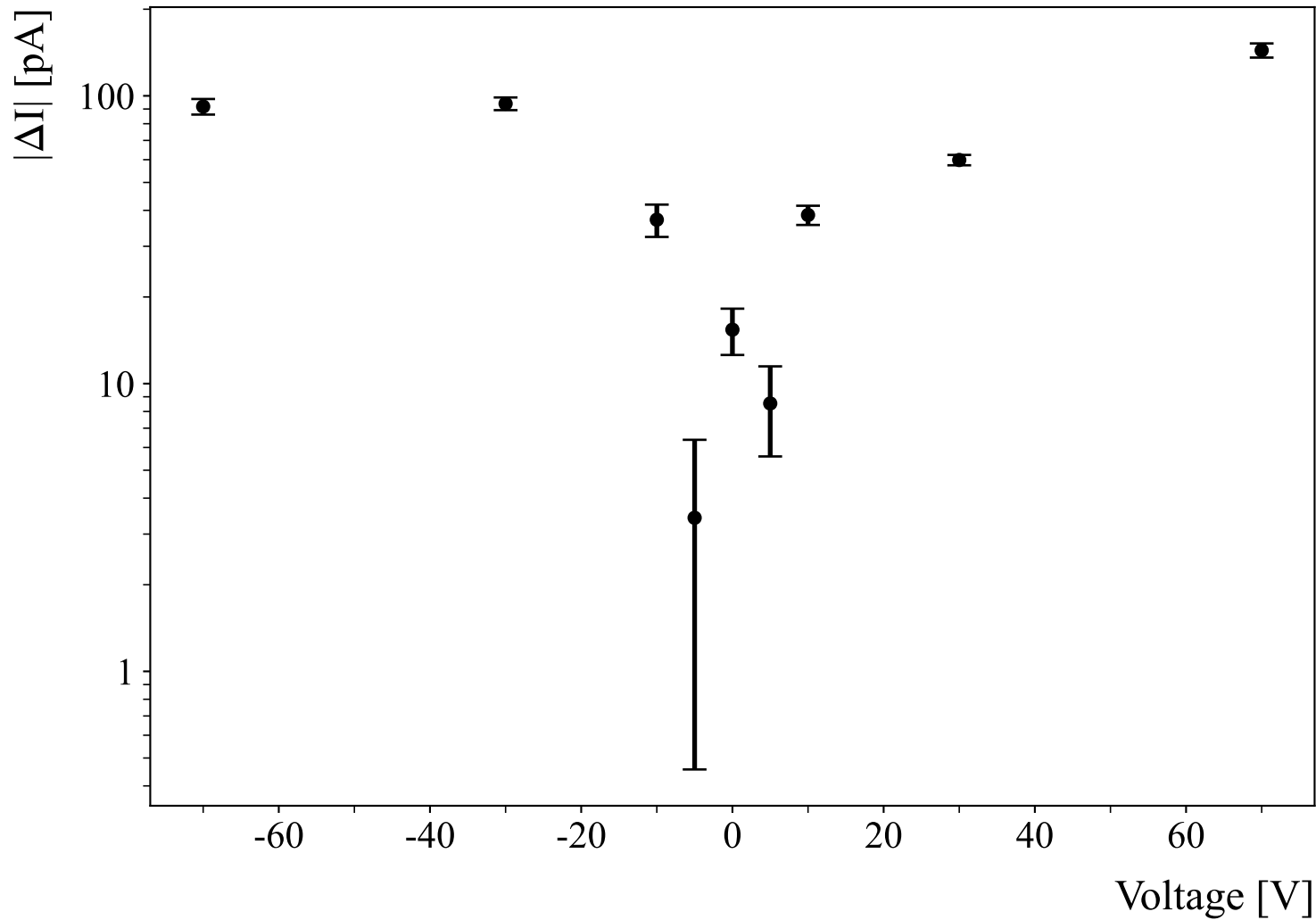
DG-PCB001_dynamics_voltage_7.5mm
