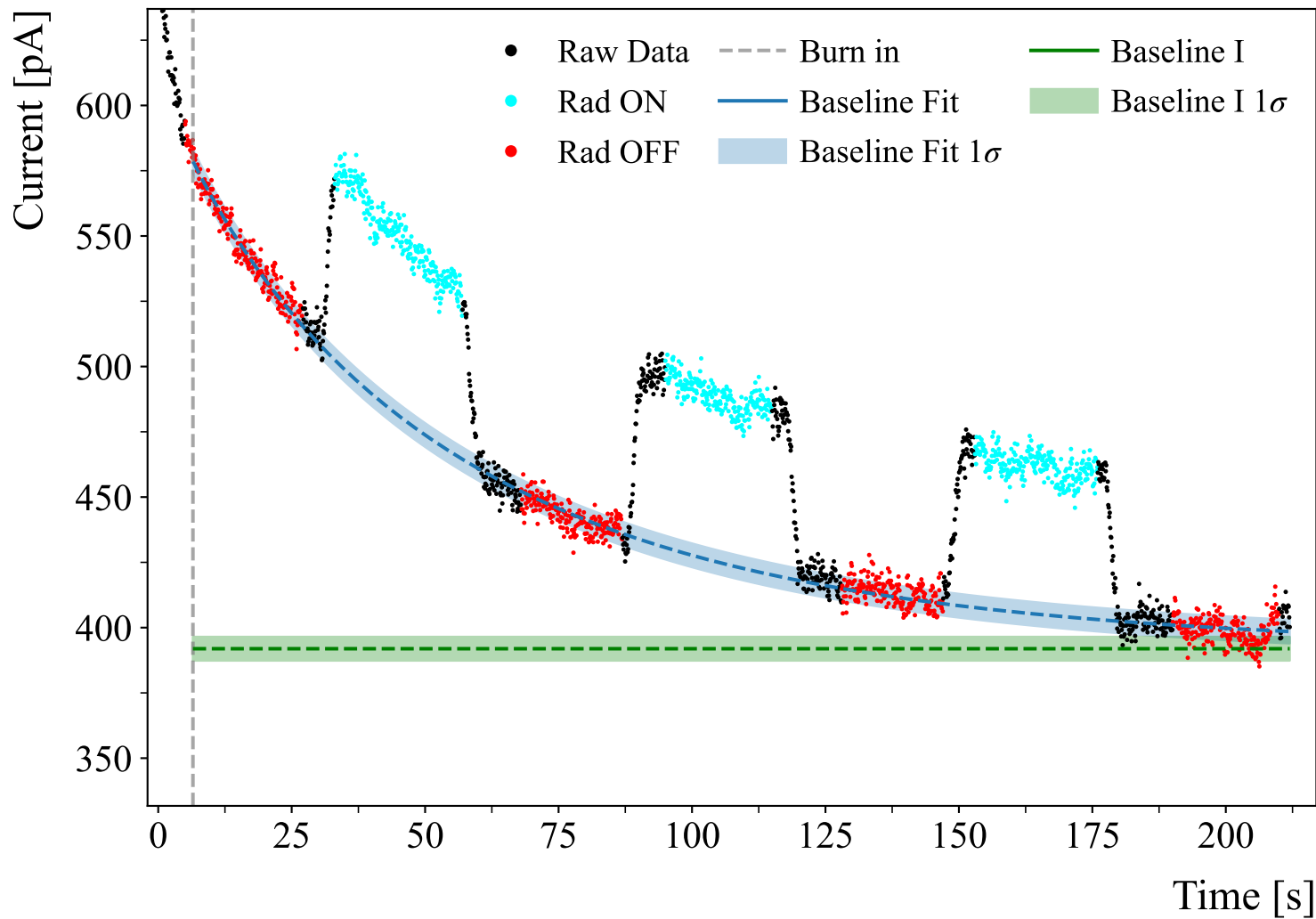
dynamic_standoffs_30V_11.5mm_initial
