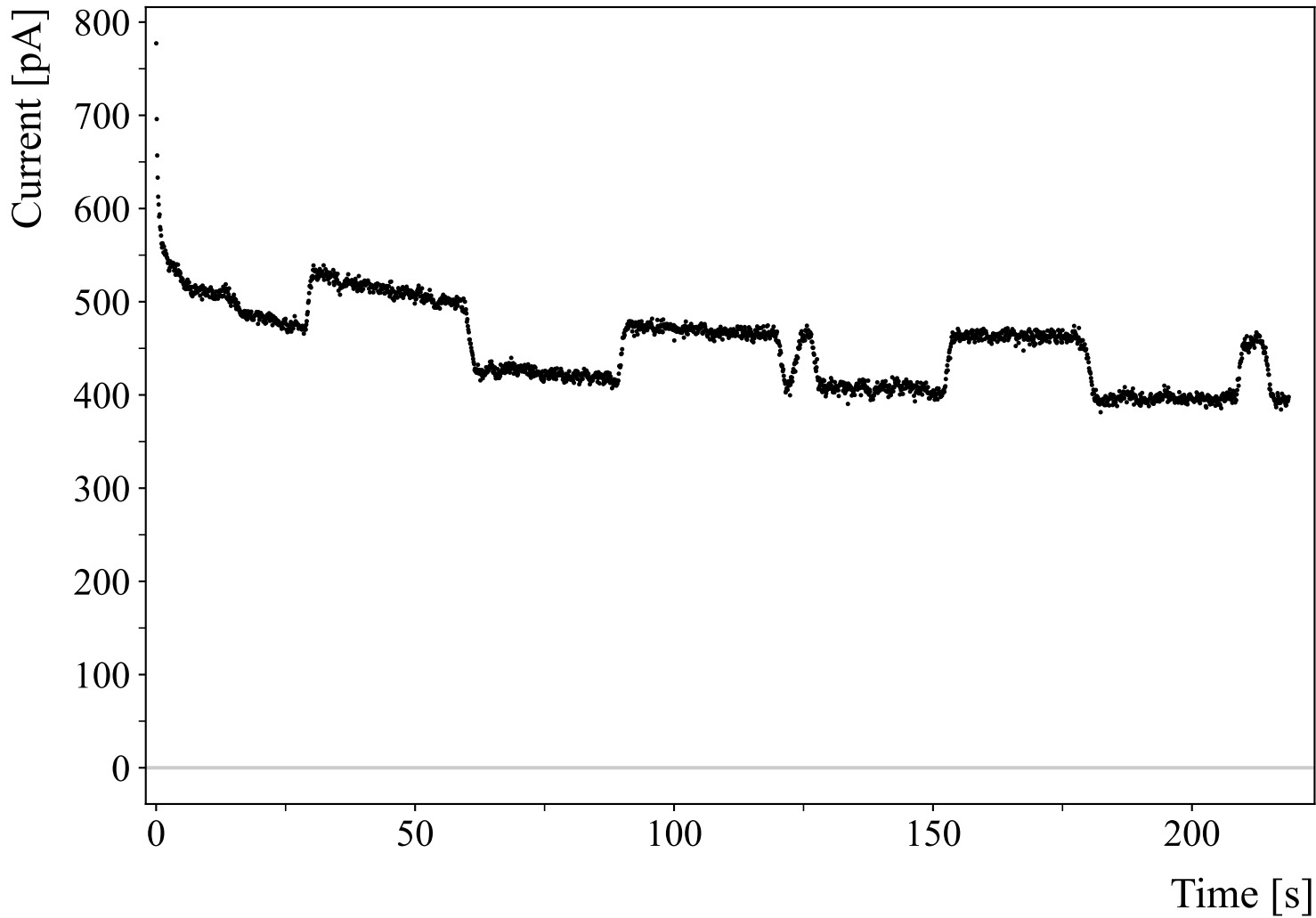
dynamic_standoffs_30V_7.5mm_raw
