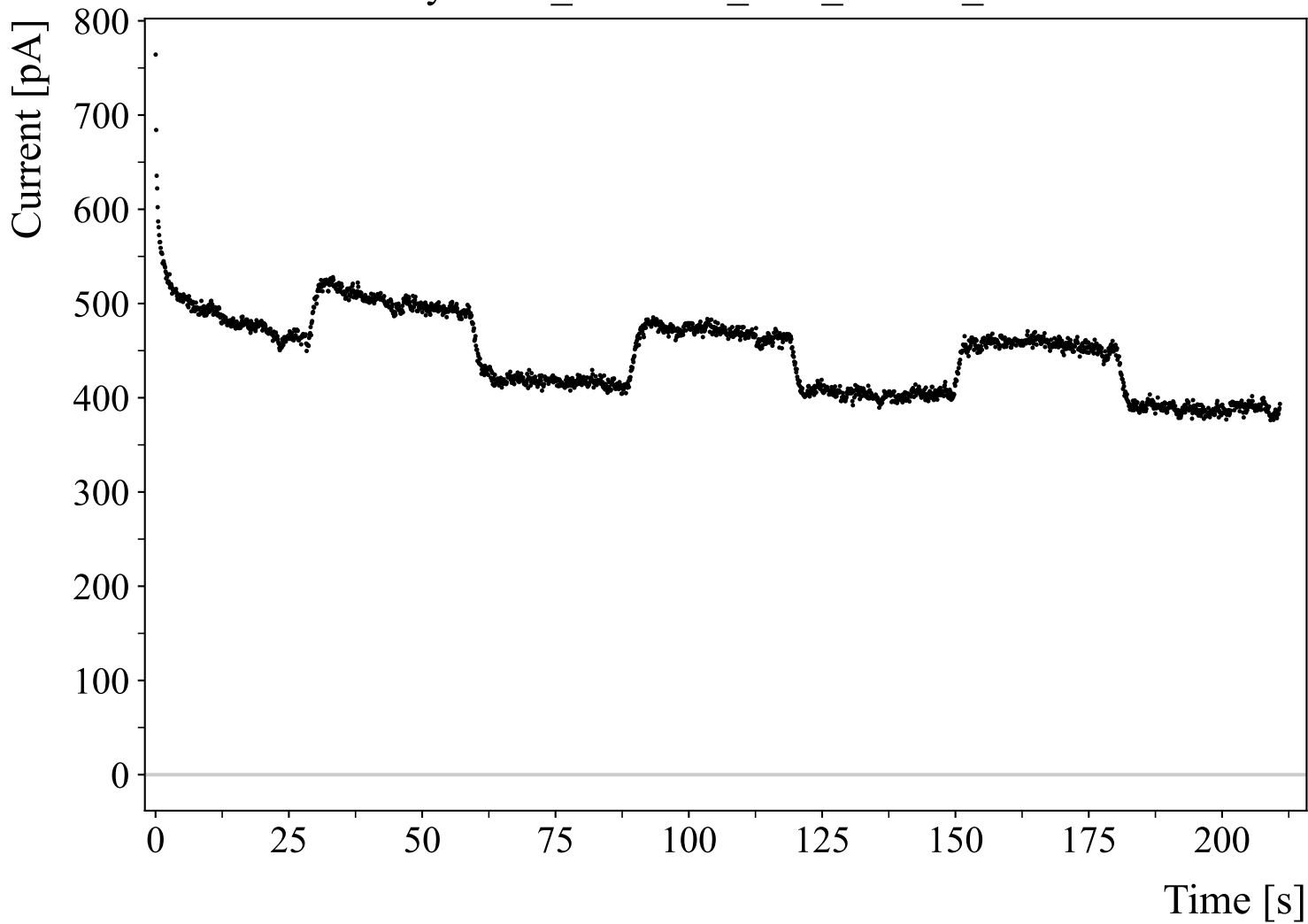
dynamic_standoffs_30V_9.5mm_raw
