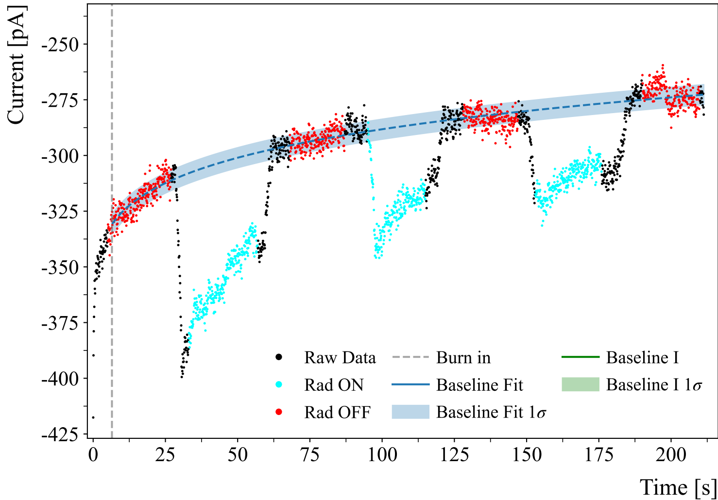
dynamic_voltages_-10V_7.5mm_initial
