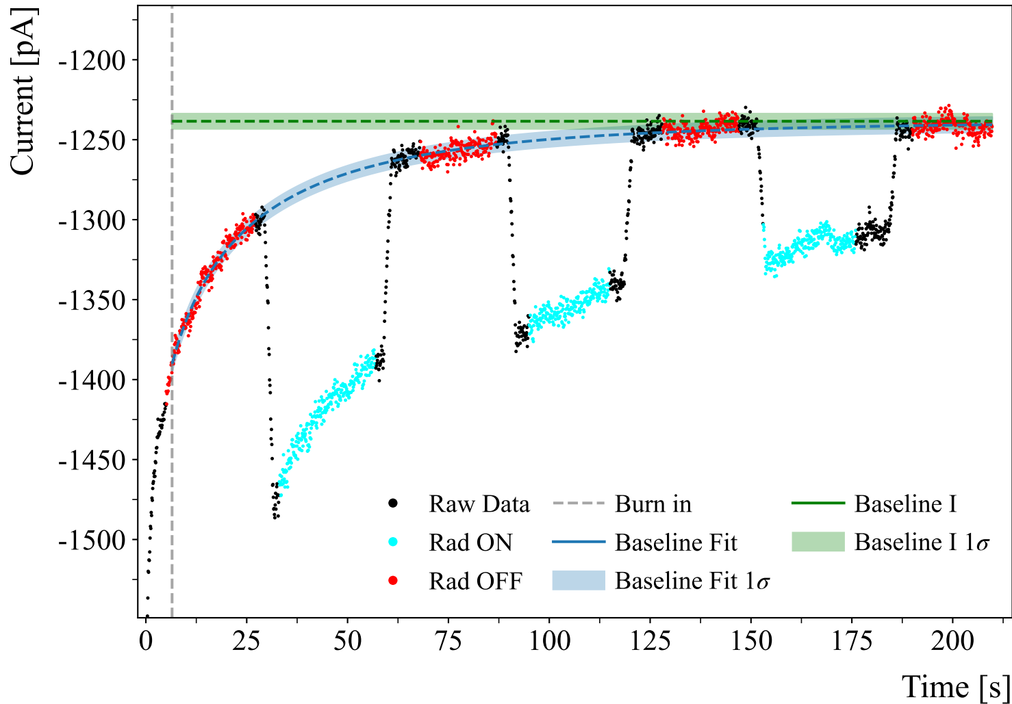
dynamic_voltages_-30V_7.5mm_initial
