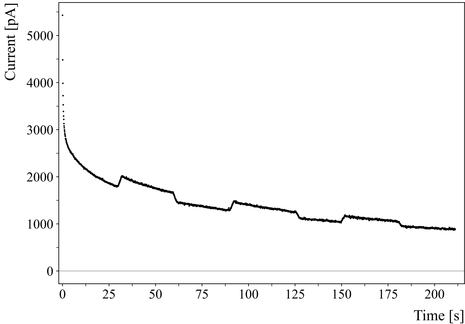
dynamic_voltages_70V_7.5mm_raw
