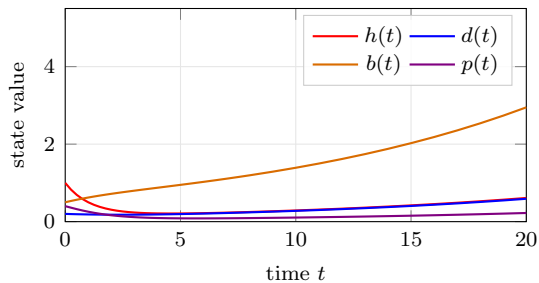
(a) x_0 = (1.0, 0.2, 0.5, 0.4)
