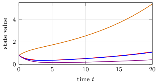
(c) x_0 = (0.8, 0.8, 0.8, 0.8)
