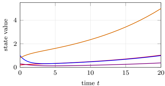
(b) x_0 = (0.2, 1.0, 0.8, 0.3)
