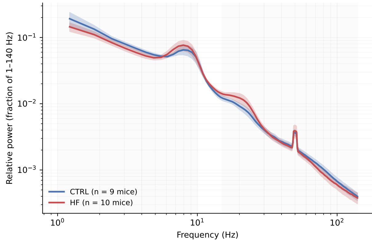
Group-average LH PSD — Cable1
