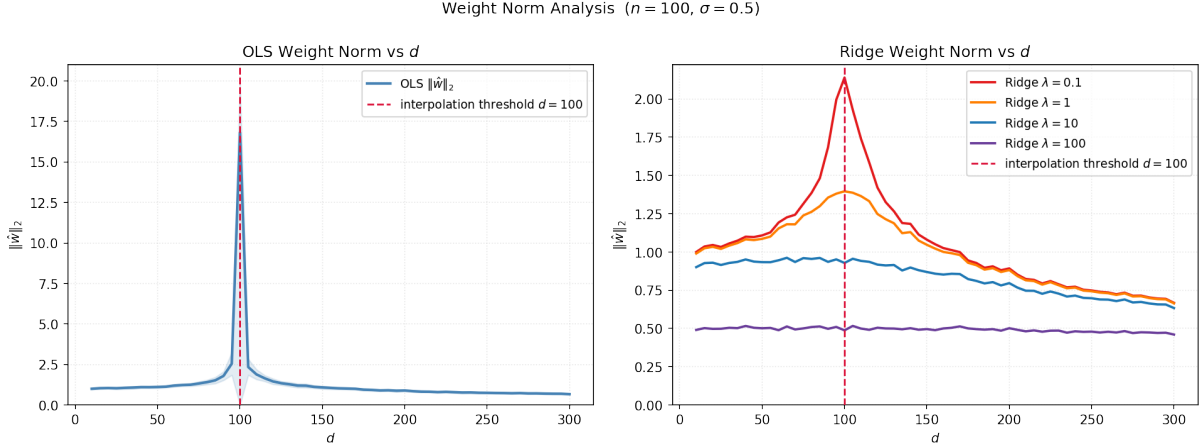
Figure 5: \ell_2 weight norm for OLS (left) and Ridge (right) vs. d ( n = 100, \sigma = 0.5 ).
