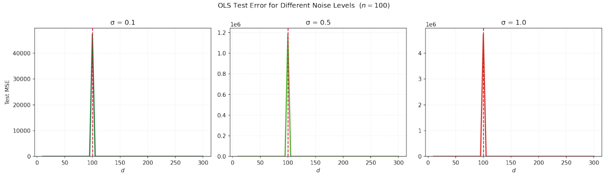
Figure 4: OLS test MSE for each noise level on its own y-axis scale. Left: \sigma = 0.1 . Centre: \sigma = 0.5 . Right: \sigma = 1.0 .
