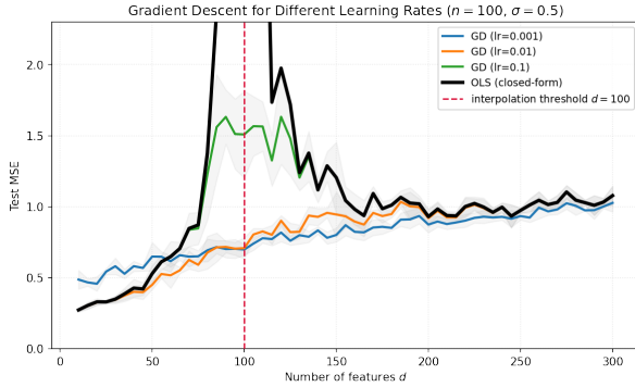
Figure 7: Effect of learning rate ( \eta ) on GD test MSE. Fixed 800 epochs.
