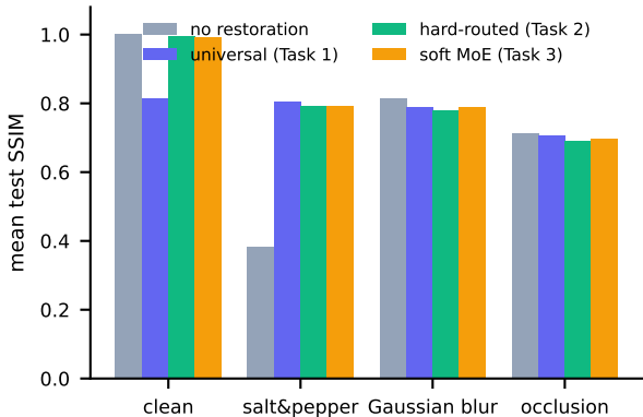
SSIM by input type (36,690 test inputs)
