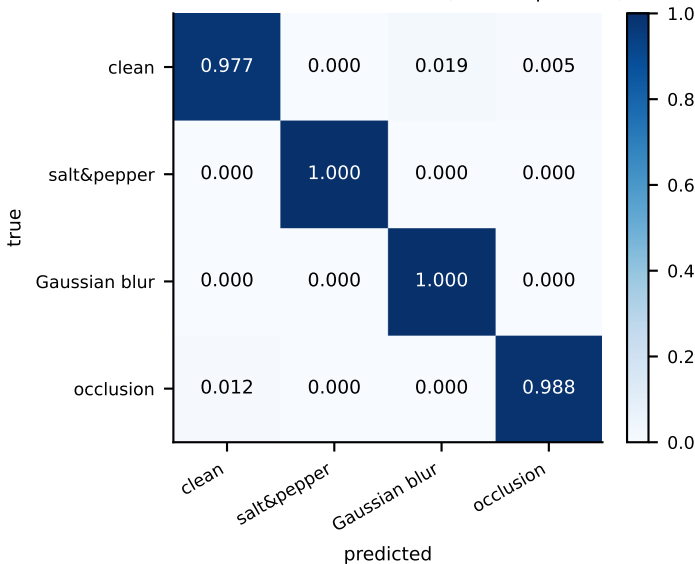
Normalised confusion matrix (full test protocol)
