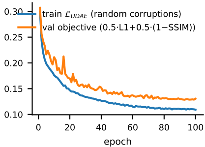
Loss
