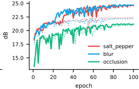
Specialists: validation PSNR (dotted = first run, \alpha \approx 0.29 )
