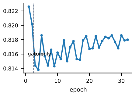
Validation SSIM (warm-up, then joint)
